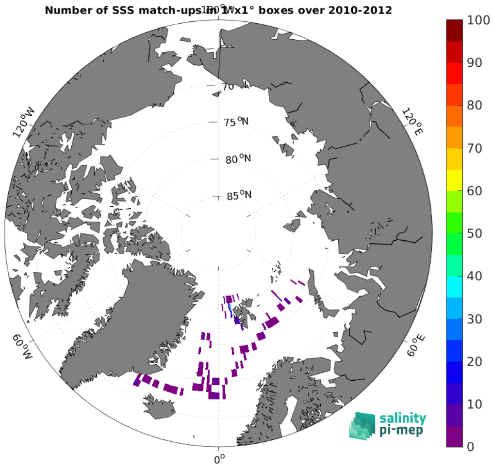
Figure 4: Number of SSS match-ups between Marine mammals SSS and the CCI SSS L4 Merged-OI v3.2 - 7-day running (ESA) SSS product for the Arctic Ocean Pi-MEP region over 1^\circ \times 1^\circ boxes and for the full satellite product period.
