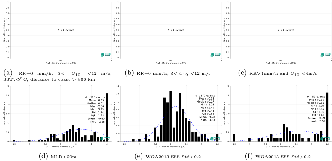
Figure 13: Normalized histogram of \Delta\text{SSS} (CCI SSS L4 Merged-OI v3.2 - 7-day running (ESA) - Marine mammals) for 6 different subdatasets corresponding to: RR=0 mm/h, 3 < U_{10} < 12 m/s, SST > 5^\circ\text{C} , distance to coast > 800 km (a), RR=0 mm/h, 3 < U_{10} < 12 m/s (b), RR > 1\text{mm/h} and U_{10} < 4\text{m/s} (c), MLD < 20\text{m} (d), WOA2013 SSS Std < 0.2 (e), WOA2013 SSS Std > 0.2 (f).
