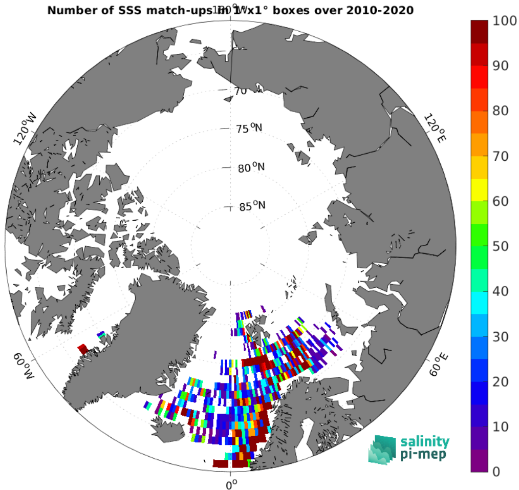
Figure 4: Number of SSS match-ups between ICES SSS and the CCI SSS L4 Merged-OI v3.2 - 7-day running (ESA) SSS product for the Arctic Ocean Pi-MEP region over 1^\circ \times 1^\circ boxes and for the full satellite product period.
