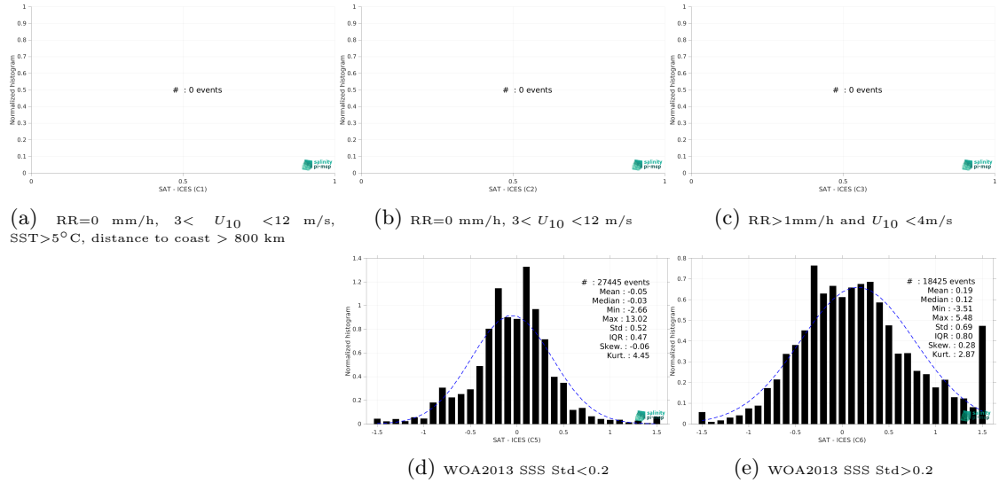
Figure 13: Normalized histogram of \Delta SSS (CCI SSS L4 Merged-OI v3.2 - 7-day running (ESA) - ICES) for 5 different subdatasets corresponding to: RR=0 mm/h, 3 < U_{10} < 12 m/s, SST > 5°C, distance to coast > 800 km (a), RR=0 mm/h, 3 < U_{10} < 12 m/s (b), RR > 1mm/h and U_{10} < 4 m/s (c), WOA2013 SSS Std < 0.2 (d), WOA2013 SSS Std > 0.2 (e).
