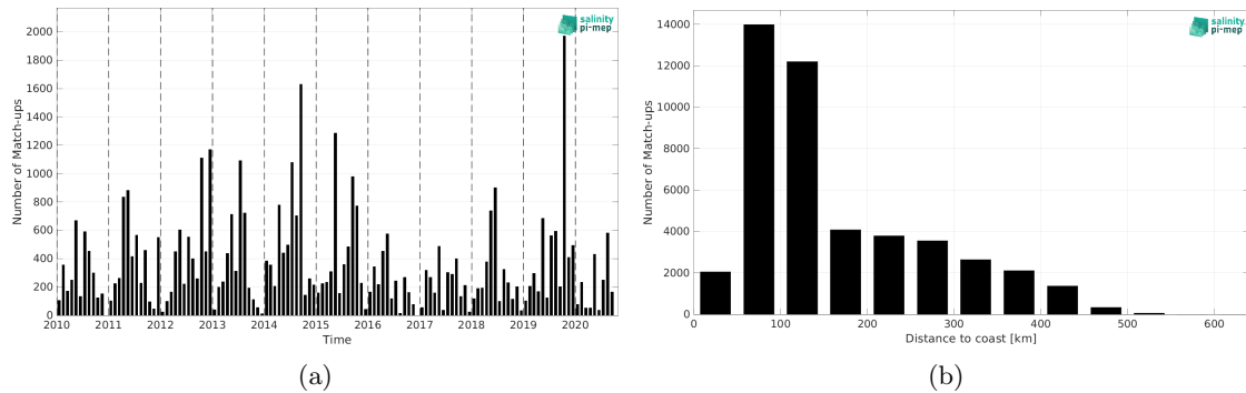
Figure 1: Number of match-ups between ICES and CCI SSS L4 Merged-OI v3.2 - 7-day running (ESA) SSS as a function of time (a) and as function of the distance to coast (b) over the Arctic Ocean Pi-MEP region and for the full satellite product period.
