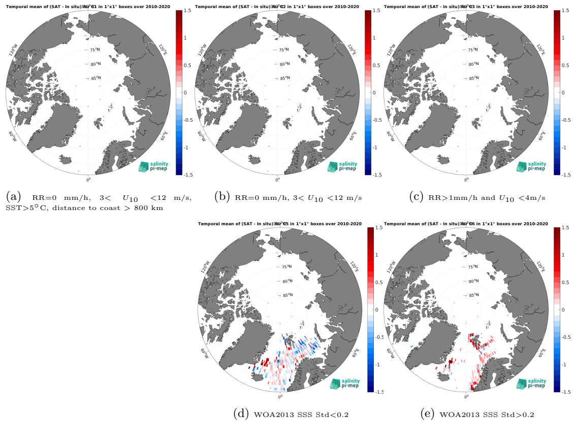
Figure 12: Temporal mean gridded over spatial boxes of size 1^{\circ}\times 1^{\circ} of \Delta\text{SSS} (CCI SSS L4 Merged-OI v3.2 - 7-day running (ESA) - ICES) for 5 different subdatasets corresponding to:RR=0 mm/h, 3 < U_{10} < 12 m/s, SST > 5^{\circ}\text{C} , distance to coast > 800 km (a), RR=0 mm/h, 3 < U_{10} < 12 m/s (b), RR > 1 mm/h and U_{10} < 4 m/s (c), WOA2013 SSS Std < 0.2 (d), WOA2013 SSS Std > 0.2 (e).
