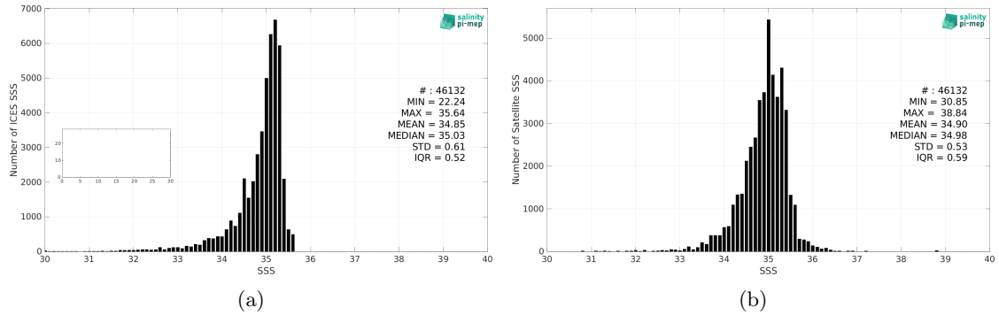
Figure 2: Histograms of SSS from ICES (a) and CCI SSS L4 Merged-OI v3.2 - 7-day running (ESA) (b) considering all match-up pairs per bins of 0.1 over the Arctic Ocean Pi-MEP region and for the full satellite product period.
