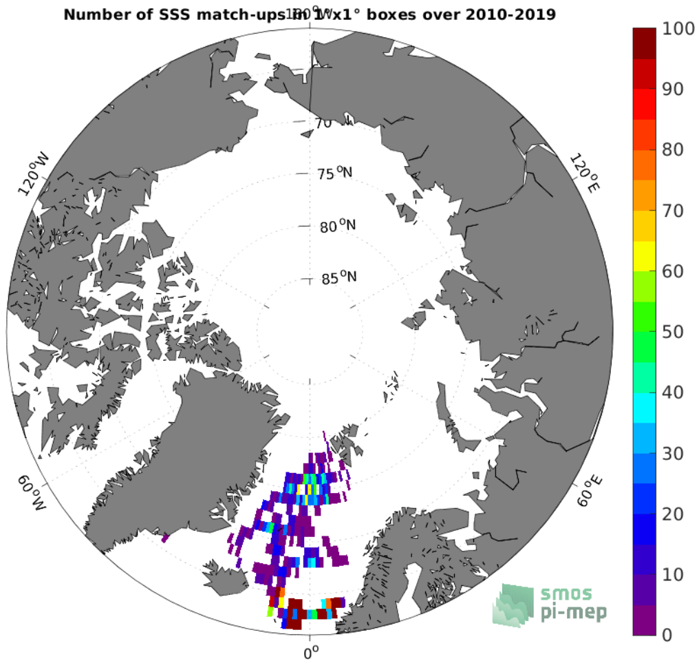
Figure 3: Number of SSS match-ups between Surface drifters SSS and the CCI SSS L4 Merged-OI v3.2 - 7-day running (ESA) SSS product for the Arctic Ocean Pi-MEP region over 1^\circ \times 1^\circ boxes and for the full satellite product period.
