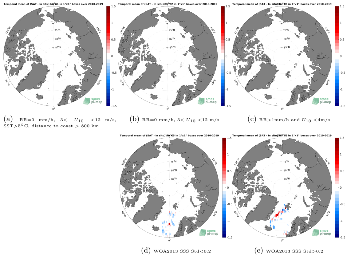
Figure 11: Temporal mean gridded over spatial boxes of size 1^{\circ}\times 1^{\circ} of \Delta\text{SSS} (CCI SSS L4 Merged-OI v3.2 - 7-day running (ESA) - Surface drifters) for 5 different subdatasets corresponding to:RR=0 mm/h, 3 < U_{10} < 12 m/s, SST >5^{\circ}\text{C} , distance to coast > 800 km (a), RR=0 mm/h, 3 < U_{10} < 12 m/s (b), RR >1 mm/h and U_{10} < 4 m/s (c), WOA2013 SSS Std <0.2 (d), WOA2013 SSS Std >0.2 (e).
