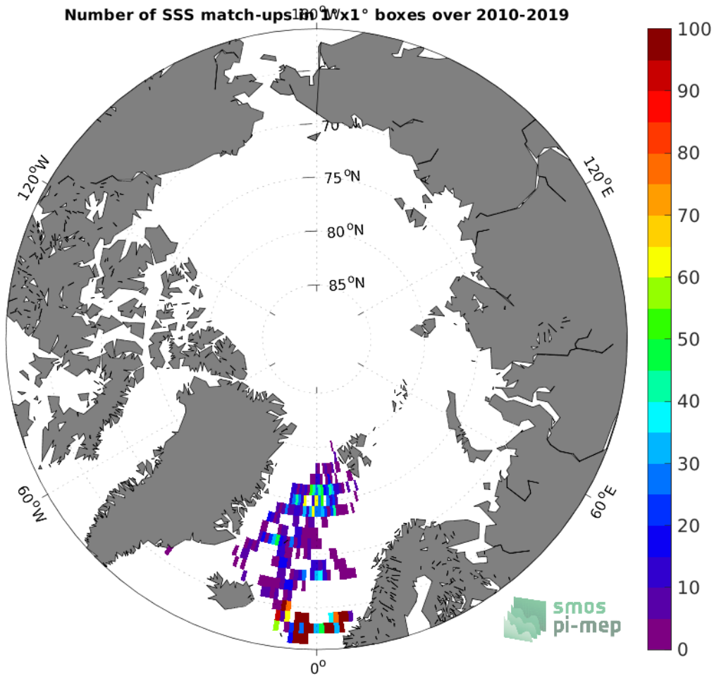
Figure 3: Number of SSS match-ups between Surface drifters SSS and the CCI SSS L4 Merged-OI v3.2 - 7-day running (ESA) SSS product for the Arctic Ocean Pi-MEP region over 1^{\circ} \times 1^{\circ} boxes and for the full satellite product period.
