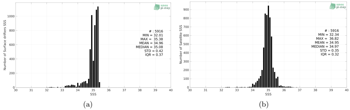
Figure 2: Histograms of SSS from Surface drifters (a) and CCI SSS L4 Merged-OI v3.2 - 7-day running (ESA) (b) considering all match-up pairs per bins of 0.1 over the Arctic Ocean Pi-MEP region and for the full satellite product period.
