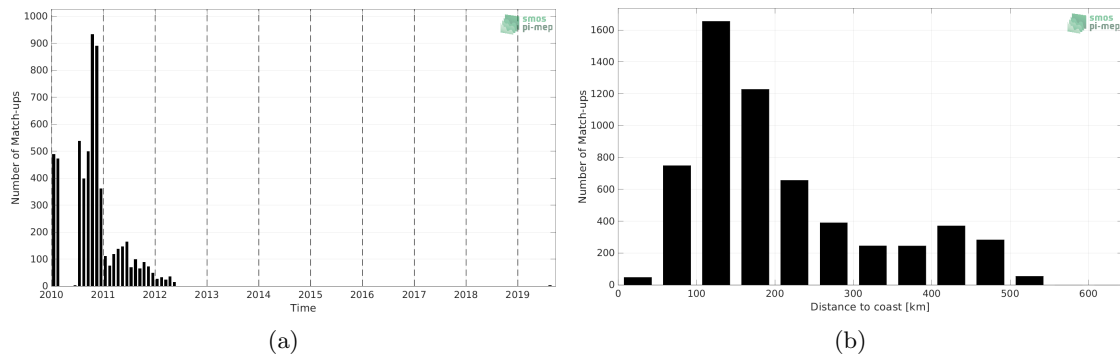
Figure 1: Number of match-ups between Surface drifters and CCI SSS L4 Merged-OI v3.2 - 7-day running (ESA) SSS as a function of time (a) and as function of the distance to coast (b) over the Arctic Ocean Pi-MEP region and for the full satellite product period.
