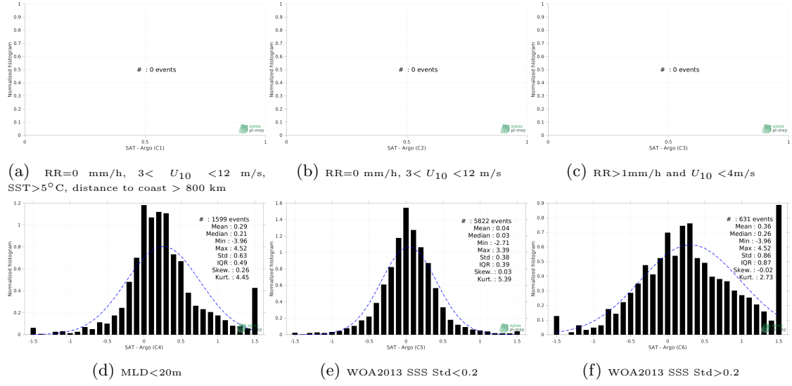
Figure 13: Normalized histogram of \Delta\text{SSS} (CCI SSS L4 Merged-OI v3.2 - 7-day running (ESA) - Argo) for 6 different subdatasets corresponding to: RR=0 mm/h, 3 < U_{10} < 12 m/s, SST > 5^{\circ}\text{C} , distance to coast > 800 km (a), RR=0 mm/h, 3 < U_{10} < 12 m/s (b), RR > 1\text{mm/h} and U_{10} < 4\text{m/s} (c), MLD < 20\text{m} (d), WOA2013 SSS Std < 0.2 (e), WOA2013 SSS Std > 0.2 (f).
