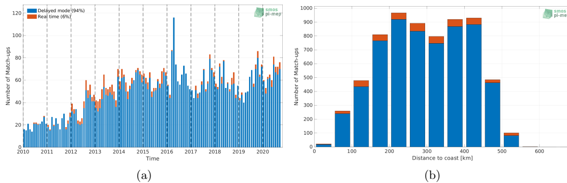
Figure 1: Number of match-ups between Argo and CCI SSS L4 Merged-OI v3.2 - 7-day running (ESA) SSS as a function of time (a) and as function of the distance to coast (b) over the Arctic Ocean Pi-MEP region and for the full satellite product period.
