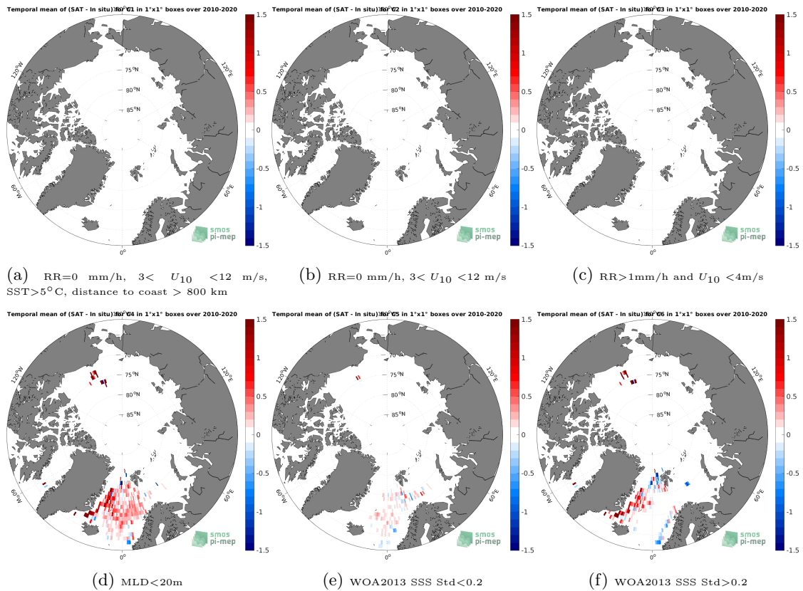
Figure 12: Temporal mean gridded over spatial boxes of size 1^{\circ}\times 1^{\circ} of \Delta\text{SSS} (CCI SSS L4 Merged-OI v3.2 - 7-day running (ESA) - Argo) for 6 different subdatasets corresponding to:RR=0 mm/h, 3 < U_{10} < 12 m/s, SST > 5^{\circ}\text{C} , distance to coast > 800 km (a), RR=0 mm/h, 3 < U_{10} < 12 m/s (b), RR > 1\text{mm/h} and U_{10} < 4\text{m/s} (c),MLD < 20\text{m} (d),WOA2013 SSS Std < 0.2 (e),WOA2013 SSS Std > 0.2 (f).
