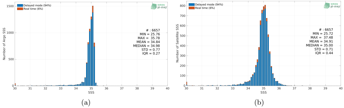
Figure 2: Histograms of SSS from Argo (a) and CCI SSS L4 Merged-OI v3.2 - 7-day running (ESA) (b) considering all match-up pairs per bins of 0.1 over the Arctic Ocean Pi-MEP region and for the full satellite product period.
