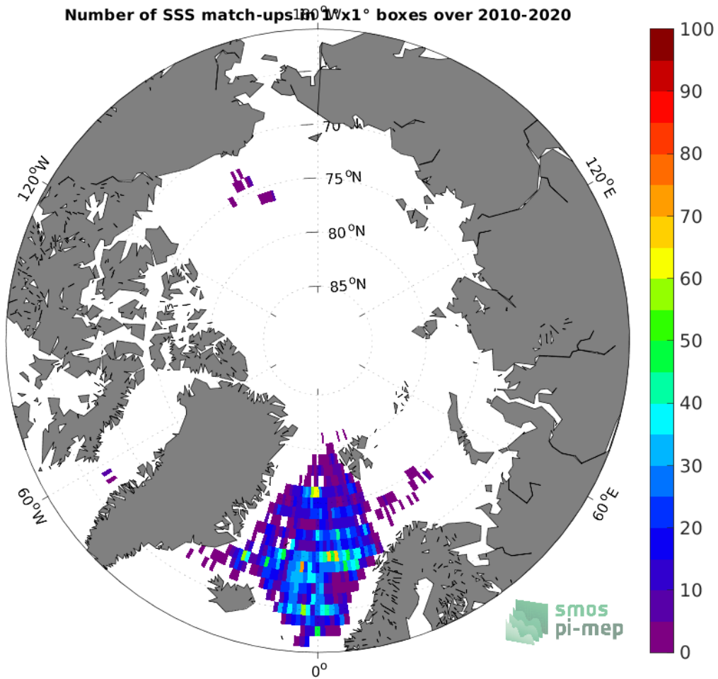
Figure 4: Number of SSS match-ups between Argo SSS and the CCI SSS L4 Merged-OI v3.2 - 7-day running (ESA) SSS product for the Arctic Ocean Pi-MEP region over 1^\circ \times 1^\circ boxes and for the full satellite product period.
