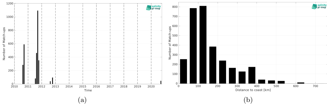
Figure 1: Number of match-ups between TSG (SAMOS) and CCI SSS L4 Merged-OI v3.2 - 30-day running (ESA) SSS as a function of time (a) and as function of the distance to coast (b) over the Arctic Ocean Pi-MEP region and for the full satellite product period.
