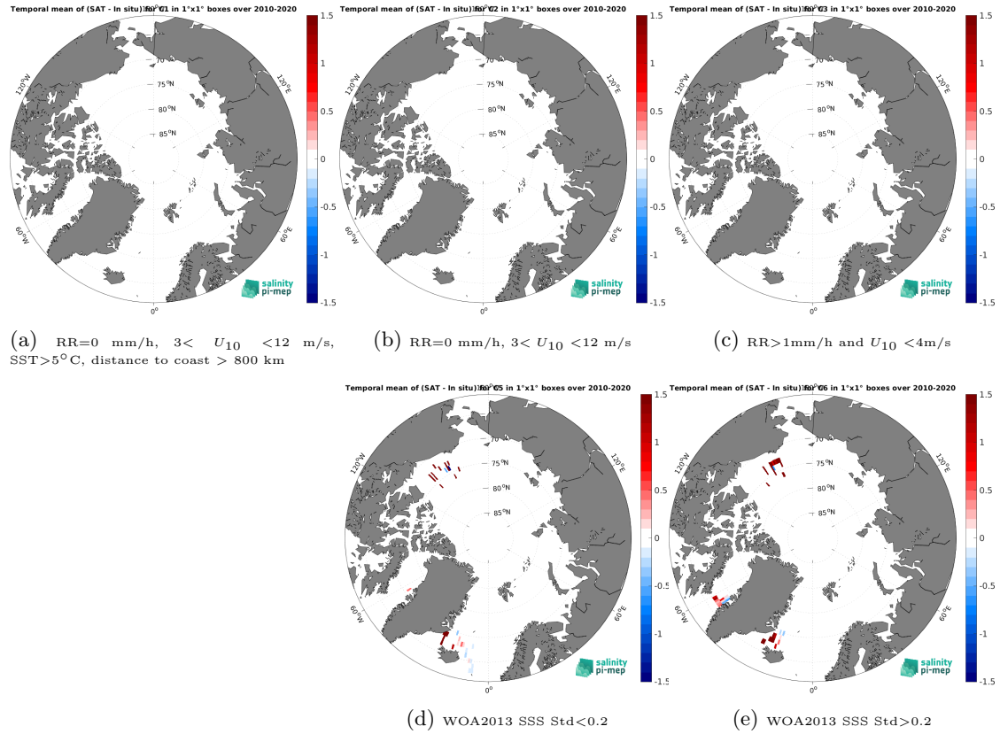
Figure 12: Temporal mean gridded over spatial boxes of size 1^{\circ}\times 1^{\circ} of \Delta\text{SSS} (CCI SSS L4 Merged-OI v3.2 - 30-day running (ESA) - TSG (SAMOS)) for 5 different subdatasets corresponding to: RR=0 mm/h, 3 < U_{10} < 12 m/s, SST > 5^{\circ}\text{C} , distance to coast > 800 km (a), RR=0 mm/h, 3 < U_{10} < 12 m/s (b), RR > 1 mm/h and U_{10} < 4 m/s (c), WOA2013 SSS Std < 0.2 (d), WOA2013 SSS Std > 0.2 (e).
