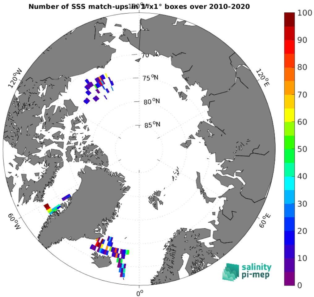
Figure 4: Number of SSS match-ups between TSG (SAMOS) SSS and the CCI SSS L4 Merged-OI v3.2 - 30-day running (ESA) SSS product for the Arctic Ocean Pi-MEP region over 1^\circ \times 1^\circ boxes and for the full satellite product period.
