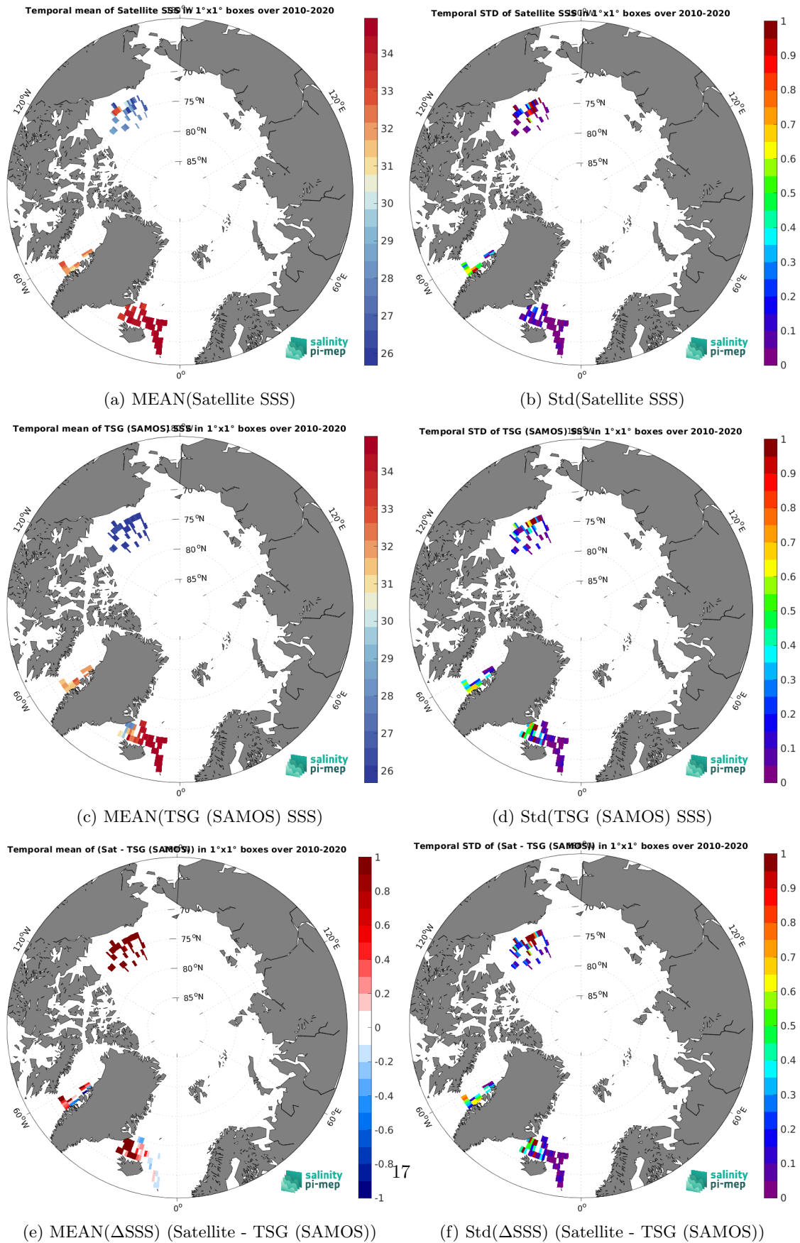
Figure 6: Temporal mean (left) and Std (right) of SSS from CCI SSS L4 Merged-OI v3.2 - 30-day running (ESA) (top), TSG (SAMOS) (middle), and of \Delta SSS (Satellite - TSG (SAMOS)). Only match-up pairs are used to generate these maps.
