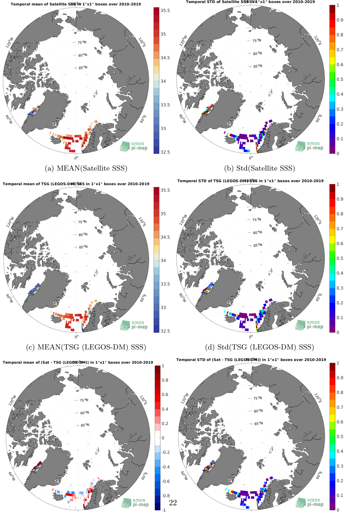
(e) MEAN( \Delta SSS) (Satellite - TSG (LEGOS-DM)) (f) Std( \Delta SSS) (Satellite - TSG (LEGOS-DM)) Figure 6: Temporal mean (left) and Std (right) of SSS from CCI SSS L4 Merged-OI v3.2 - 30-day running (ESA) (top), TSG (LEGOS-DM) (middle), and of \Delta SSS (Satellite - TSG (LEGOS-DM)). Only match-up pairs are used to generate these maps.
