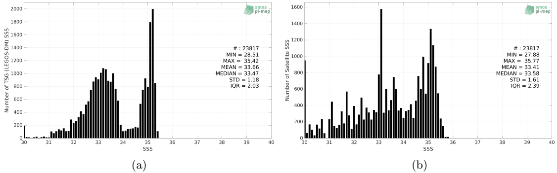
Figure 2: Histograms of SSS from TSG (LEGOS-DM) (a) and CCI SSS L4 Merged-OI v3.2 - 30-day running (ESA) (b) considering all match-up pairs per bins of 0.1 over the Arctic Ocean Pi-MEP region and for the full satellite product period.
