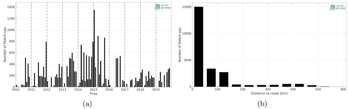
Figure 1: Number of match-ups between TSG (LEGOS-DM) and CCI SSS L4 Merged-OI v3.2 - 30-day running (ESA) SSS as a function of time (a) and as function of the distance to coast (b) over the Arctic Ocean Pi-MEP region and for the full satellite product period.
