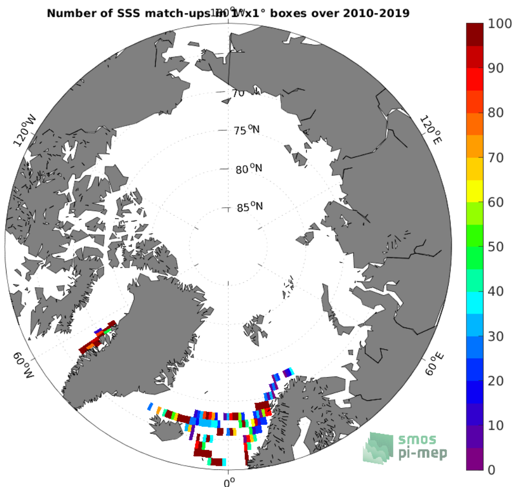
Figure 4: Number of SSS match-ups between TSG (LEGOS-DM) SSS and the CCI SSS L4 Merged-OI v3.2 - 30-day running (ESA) SSS product for the Arctic Ocean Pi-MEP region over 1^\circ \times 1^\circ boxes and for the full satellite product period.
