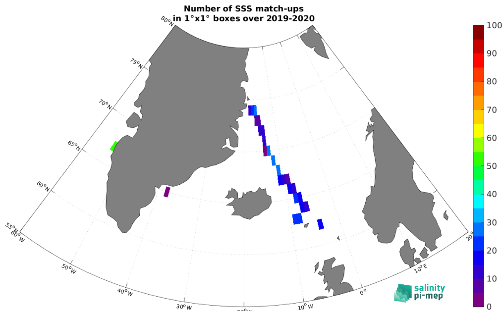
Figure 4: Number of SSS match-ups between TSG (Lauge-Koch) SSS and the CCI SSS L4 Merged-OI v3.2 - 30-day running (ESA) SSS product for the Arctic Ocean Pi-MEP region over 1^\circ \times 1^\circ boxes and for the full satellite product period.
