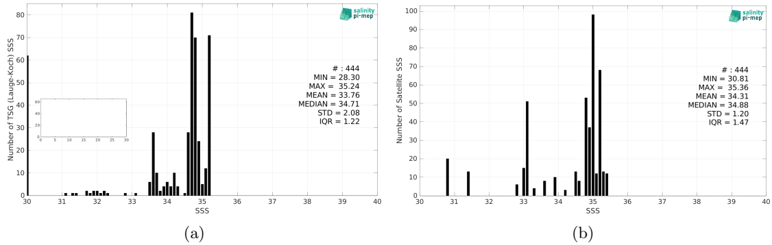
Figure 2: Histograms of SSS from TSG (Lauge-Koch) (a) and CCI SSS L4 Merged-OI v3.2 - 30-day running (ESA) (b) considering all match-up pairs per bins of 0.1 over the Arctic Ocean Pi-MEP region and for the full satellite product period.
