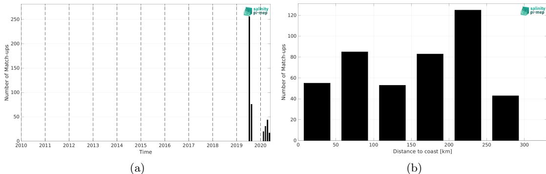
Figure 1: Number of match-ups between TSG (Lauge-Koch) and CCI SSS L4 Merged-OI v3.2 - 30-day running (ESA) SSS as a function of time (a) and as function of the distance to coast (b) over the Arctic Ocean Pi-MEP region and for the full satellite product period.
