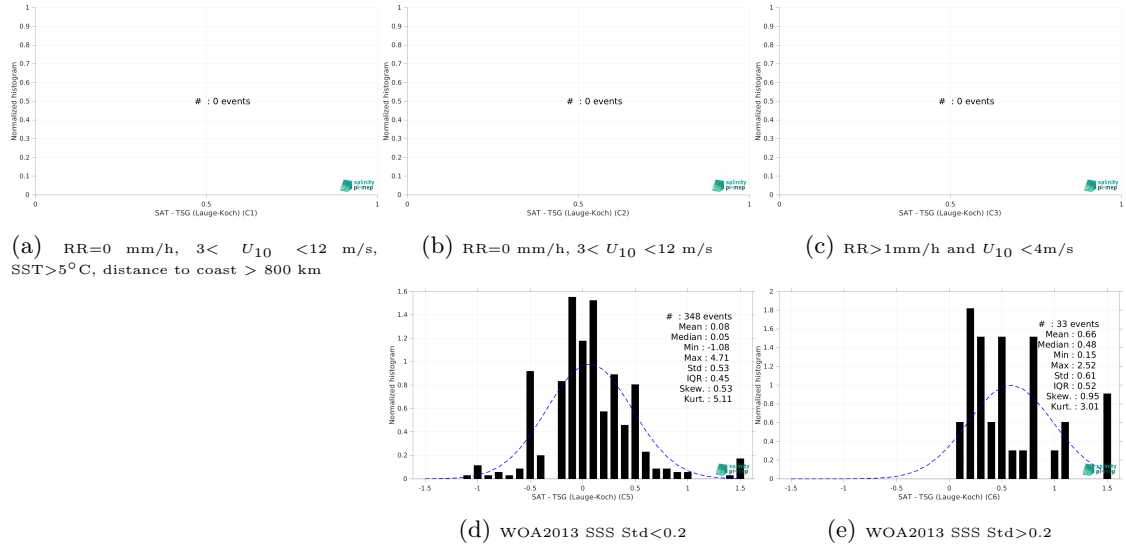
Figure 13: Normalized histogram of \Delta SSS (CCI SSS L4 Merged-OI v3.2 - 30-day running (ESA) - TSG (Lauge-Koch)) for 5 different subdatasets corresponding to: RR=0 mm/h, 3 < U_{10} < 12 m/s, SST>5°C, distance to coast > 800 km (a), RR=0 mm/h, 3 < U_{10} < 12 m/s (b), RR>1mm/h and U_{10} < 4 m/s (c), WOA2013 SSS Std<0.2 (d), WOA2013 SSS Std>0.2 (e).
