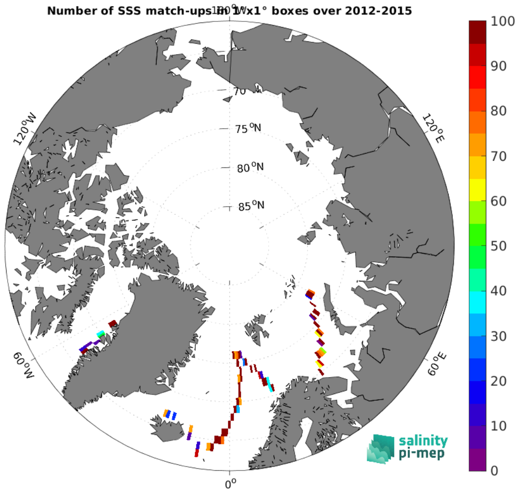
Figure 4: Number of SSS match-ups between TSG (GOSUD-Sailing-ship) SSS and the CCI SSS L4 Merged-OI v3.2 - 30-day running (ESA) SSS product for the Arctic Ocean Pi-MEP region over 1^{\circ} \times 1^{\circ} boxes and for the full satellite product period.
