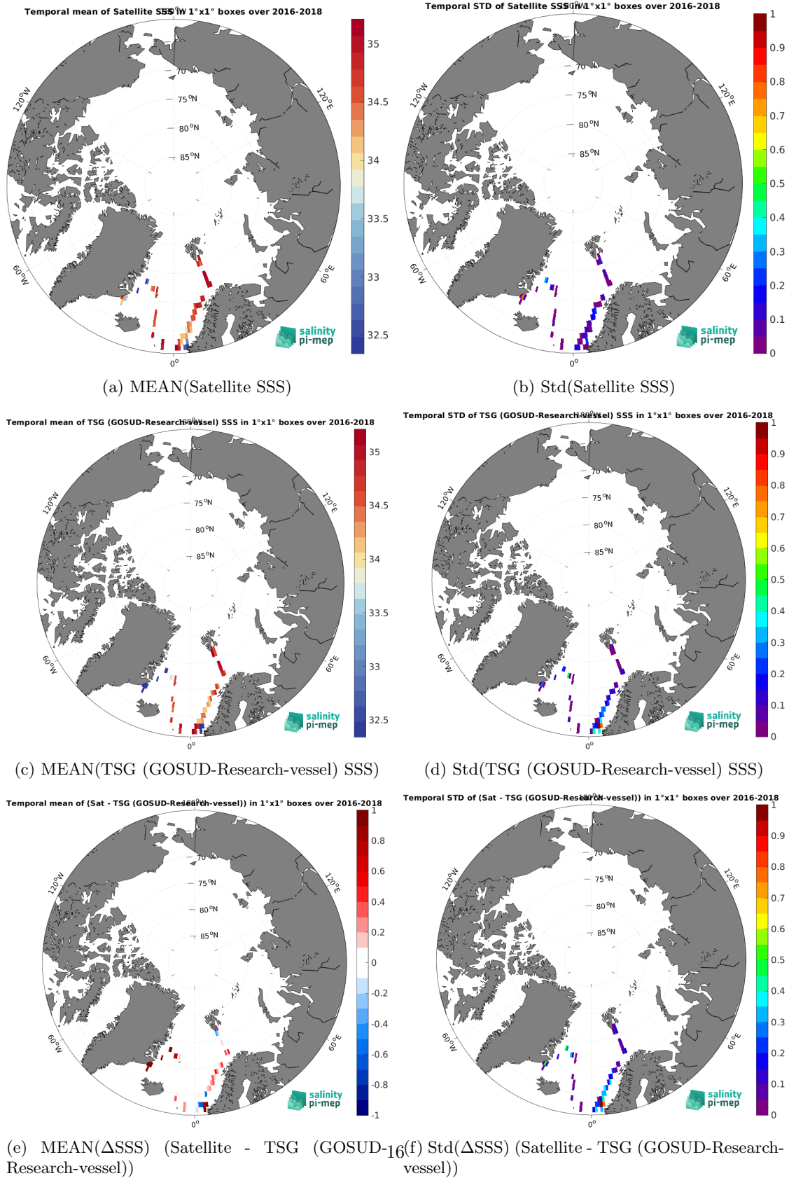
Figure 6: Temporal mean (left) and Std (right) of SSS from CCI SSS L4 Merged-OI v3.2 - 30-day running (ESA) (top), TSG (GOSUD-Research-vessel) (middle), and of \Delta SSS (Satellite - TSG (GOSUD-Research-vessel)). Only match-up pairs are used to generate these maps.
