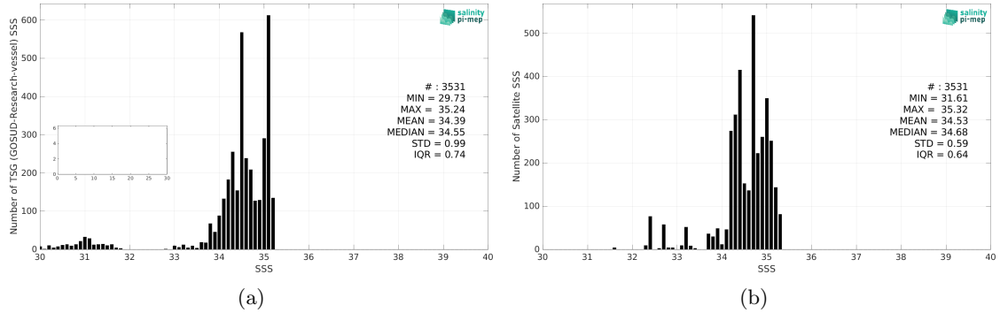
Figure 2: Histograms of SSS from TSG (GOSUD-Research-vessel) (a) and CCI SSS L4 Merged-OI v3.2 - 30-day running (ESA) (b) considering all match-up pairs per bins of 0.1 over the Arctic Ocean Pi-MEP region and for the full satellite product period.
