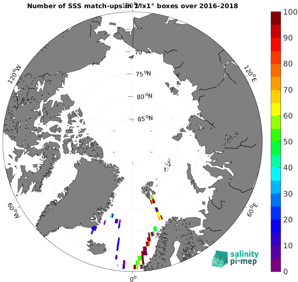
Figure 4: Number of SSS match-ups between TSG (GOSUD-Research-vessel) SSS and the CCI SSS L4 Merged-OI v3.2 - 30-day running (ESA) SSS product for the Arctic Ocean Pi-MEP region over 1^\circ \times 1^\circ boxes and for the full satellite product period.
