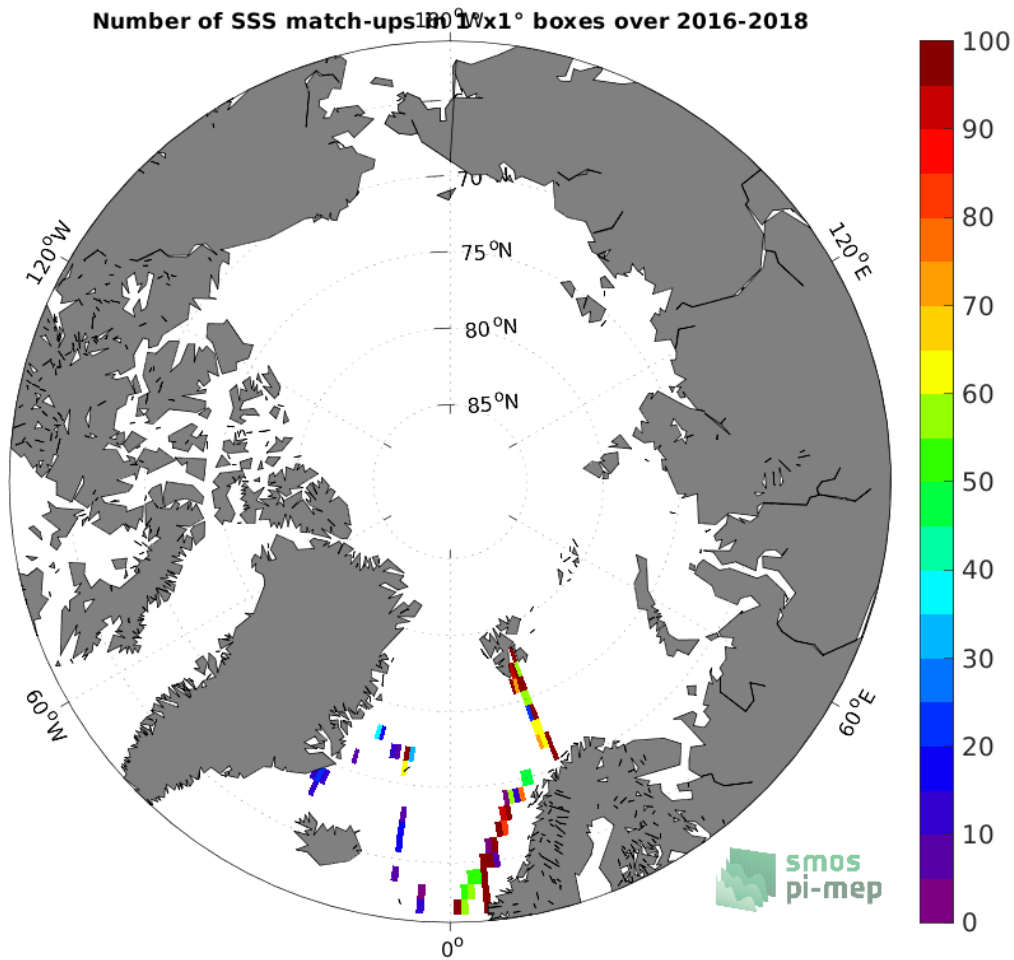
Figure 4: Number of SSS match-ups between TSG (GOSUD-Research-vessel) SSS and the CCI SSS L4 Merged-OI v3.2 - 30-day running (ESA) SSS product for the Arctic Ocean Pi-MEP region over 1^{\circ} \times 1^{\circ} boxes and for the full satellite product period.
