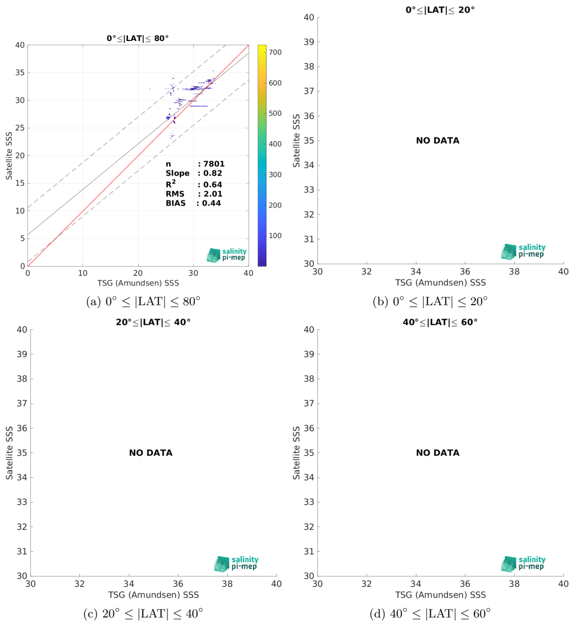
Figure 9: Contour maps of the concentration of CCI SSS L4 Merged-OI v3.2 - 30-day running (ESA) SSS (y-axis) versus TSG (Amundsen) SSS (x-axis) at match-up pairs for different latitude bands. For each plot, the red line shows x=y . The black thin and dashed lines indicate a linear fit through the data cloud and the \pm 95\% confidence levels, respectively. The number match-up pairs n , the slope and R^2 coefficient of the linear fit, the root mean square (RMS) and the mean bias between satellite and in situ data are indicated for each latitude band in each plots.
