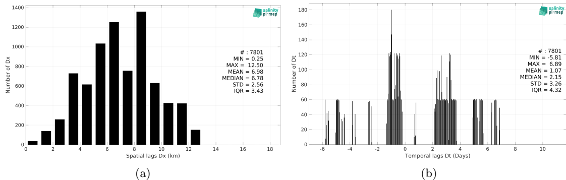
Figure 5: Histograms of the spatial (a) and temporal (b) lags between the location/time of the TSG (Amundsen) measurement and the date of the corresponding CCI SSS L4 Merged-OI v3.2 - 30-day running (ESA) SSS pixel.
