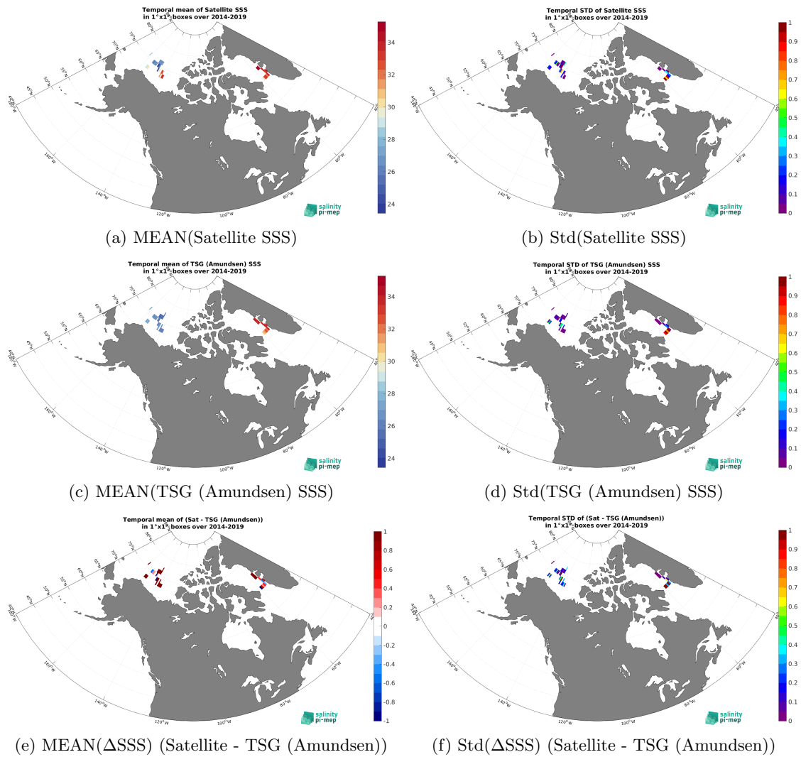
Figure 6: Temporal mean (left) and Std (right) of SSS from CCI SSS L4 Merged-OI v3.2 - 30-day running (ESA) (top), TSG (Amundsen) (middle), and of \Delta SSS (Satellite - TSG (Amundsen)). Only match-up pairs are used to generate these maps.
