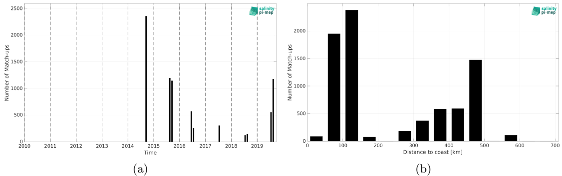
Figure 1: Number of match-ups between TSG (Amundsen) and CCI SSS L4 Merged-OI v3.2 - 30-day running (ESA) SSS as a function of time (a) and as function of the distance to coast (b) over the Arctic Ocean Pi-MEP region and for the full satellite product period.
