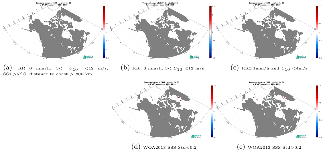
Figure 12: Temporal mean gridded over spatial boxes of size 1^{\circ}\times 1^{\circ} of \Delta\text{SSS} (CCI SSS L4 Merged-OI v3.2 - 30-day running (ESA) - TSG (Amundsen)) for 5 different subdatasets corresponding to:RR=0 mm/h, 3 < U_{10} < 12 m/s, SST >5^{\circ}\text{C} , distance to coast > 800 km (a), RR=0 mm/h, 3 < U_{10} < 12 m/s (b), RR >1 mm/h and U_{10} < 4 m/s (c), WOA2013 SSS Std <0.2 (d), WOA2013 SSS Std >0.2 (e).
