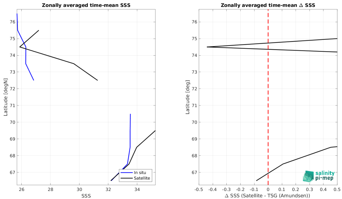
Figure 8: Left panel: Zonal mean SSS from CCI SSS L4 Merged-OI v3.2 - 30-day running (ESA) satellite product (black) and from TSG (Amundsen) (blue). Right panel: Zonal mean of \Delta SSS (Satellite - TSG (Amundsen)) for all the collected Pi-MEP match-up pairs estimated over the full satellite product period.
