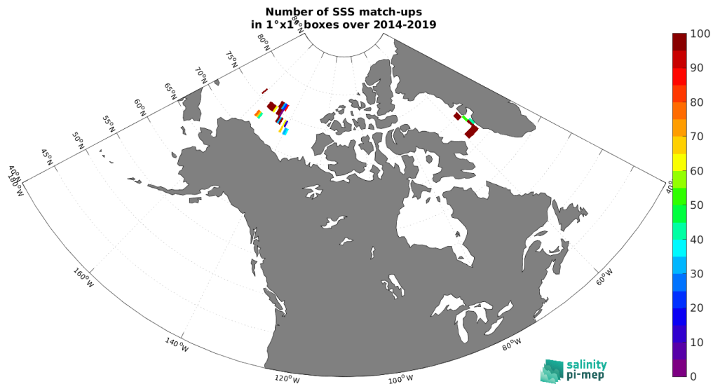
Figure 4: Number of SSS match-ups between TSG (Amundsen) SSS and the CCI SSS L4 Merged-OI v3.2 - 30-day running (ESA) SSS product for the Arctic Ocean Pi-MEP region over 1^\circ \times 1^\circ boxes and for the full satellite product period.
