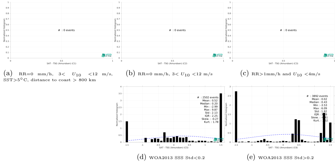
Figure 13: Normalized histogram of \Delta SSS (CCI SSS L4 Merged-OI v3.2 - 30-day running (ESA) - TSG (Amundsen)) for 5 different subdatasets corresponding to: RR=0 mm/h, 3 < U_{10} < 12 m/s, SST > 5°C, distance to coast > 800 km (a), RR=0 mm/h, 3 < U_{10} < 12 m/s (b), RR > 1mm/h and U_{10} < 4 m/s (c), WOA2013 SSS Std < 0.2 (d), WOA2013 SSS Std > 0.2 (e).
