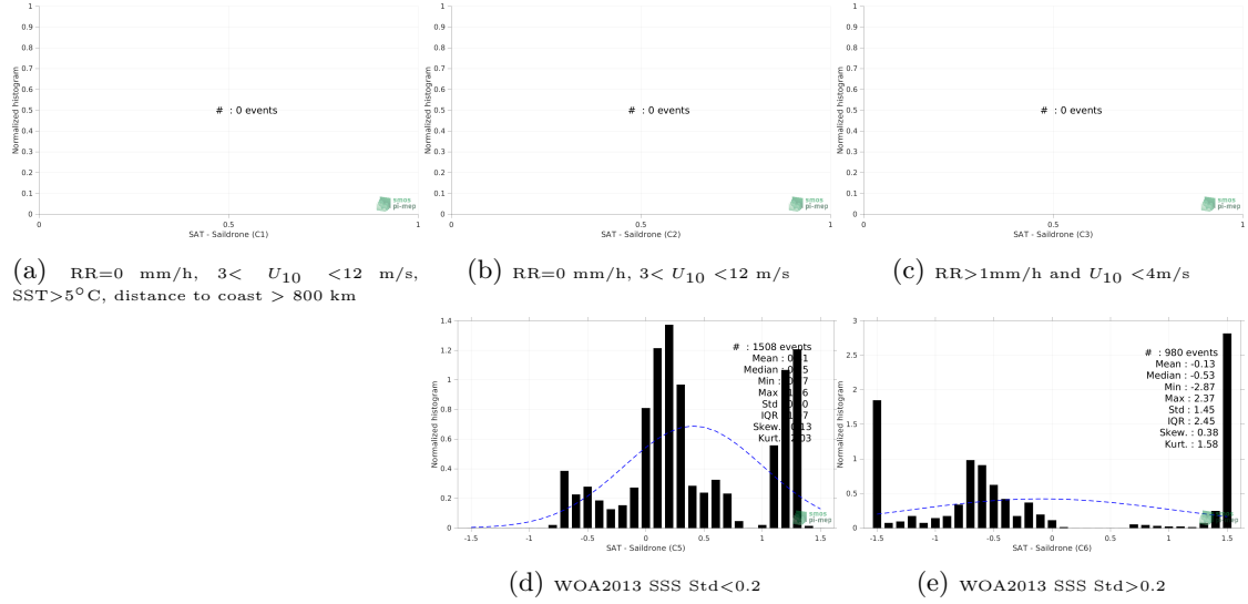
Figure 13: Normalized histogram of \Delta SSS (CCI SSS L4 Merged-OI v3.2 - 30-day running (ESA) - Sairdrone) for 5 different subdatasets corresponding to: RR=0 mm/h, 3 < U_{10} < 12 m/s, SST > 5°C, distance to coast > 800 km (a), RR=0 mm/h, 3 < U_{10} < 12 m/s (b), RR > 1mm/h and U_{10} < 4 m/s (c), WOA2013 SSS Std < 0.2 (d), WOA2013 SSS Std > 0.2 (e).
