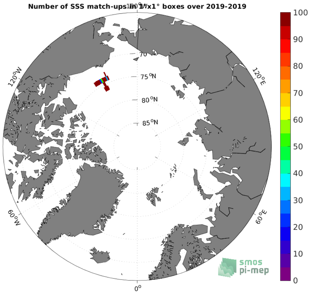
Figure 4: Number of SSS match-ups between Sairdrone SSS and the CCI SSS L4 Merged-OI v3.2 - 30-day running (ESA) SSS product for the Arctic Ocean Pi-MEP region over 1^\circ \times 1^\circ boxes and for the full satellite product period.
