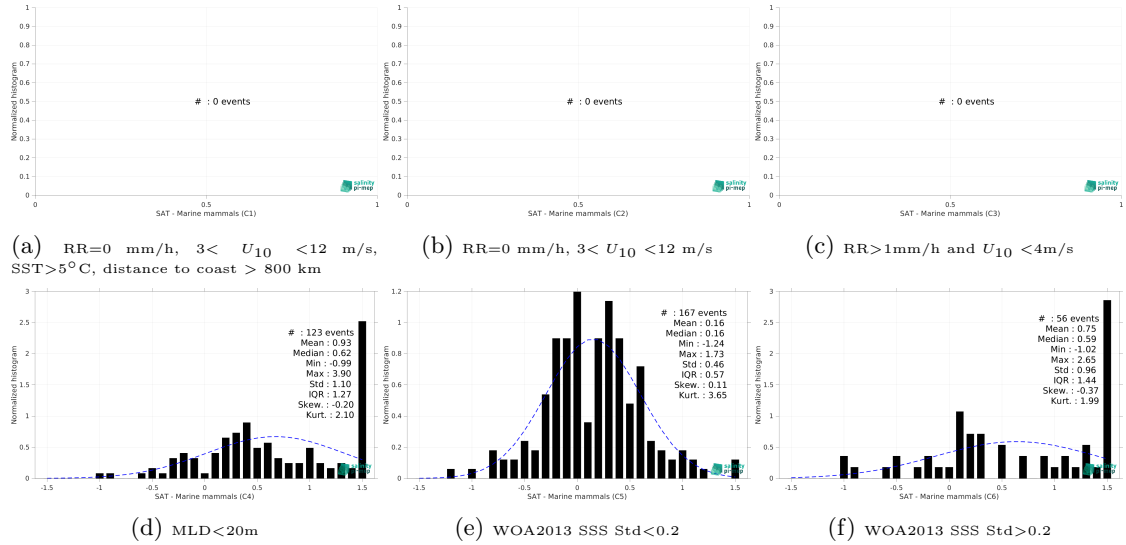
Figure 13: Normalized histogram of \Delta\text{SSS} (CCI SSS L4 Merged-OI v3.2 - 30-day running (ESA) - Marine mammals) for 6 different subdatasets corresponding to: RR=0 mm/h, 3 < U_{10} < 12 m/s, SST > 5^\circ\text{C} , distance to coast > 800 km (a), RR=0 mm/h, 3 < U_{10} < 12 m/s (b), RR > 1\text{mm/h} and U_{10} < 4\text{m/s} (c), MLD < 20\text{m} (d), WOA2013 SSS Std < 0.2 (e), WOA2013 SSS Std > 0.2 (f).
