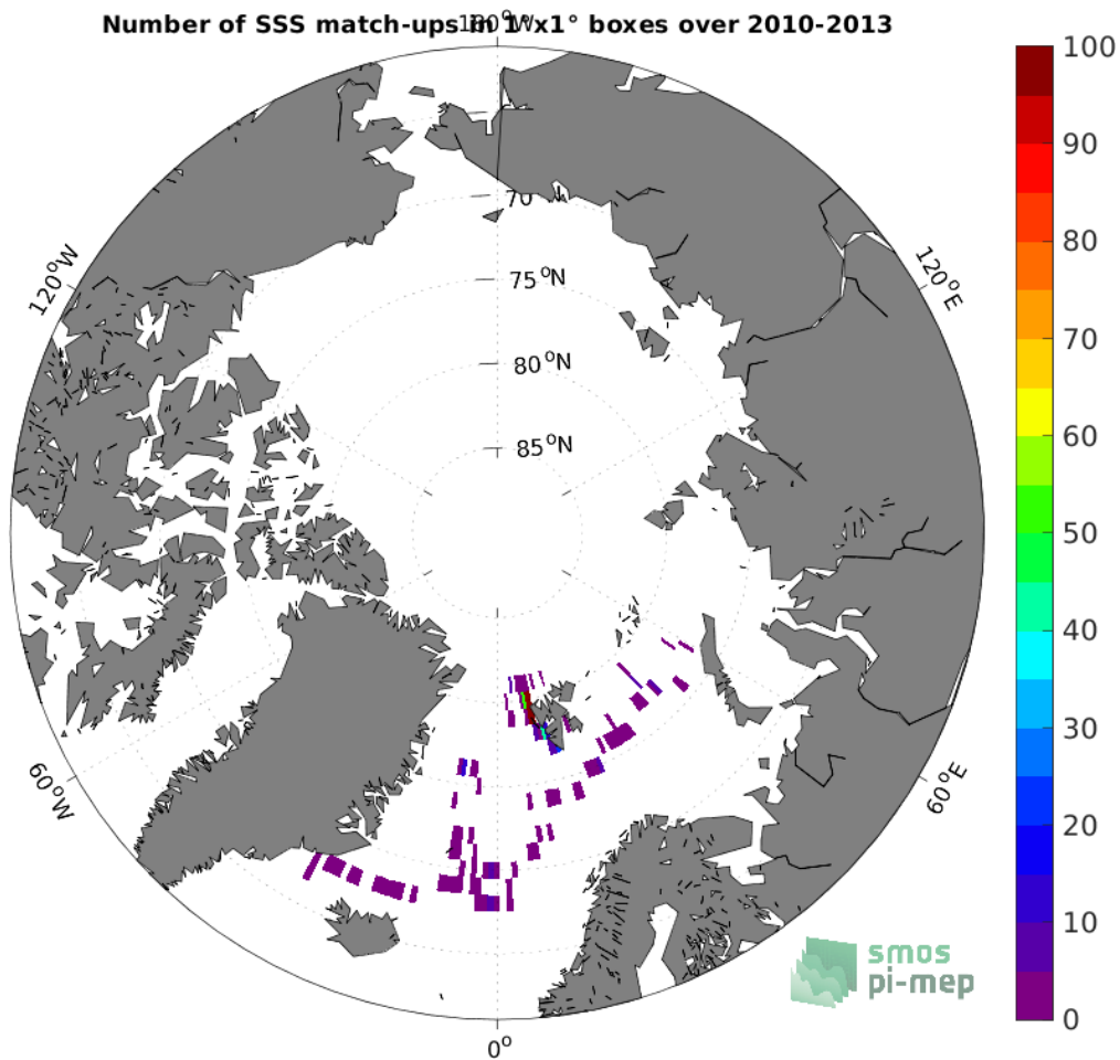
Figure 4: Number of SSS match-ups between Marine mammals SSS and the CCI SSS L4 Merged-OI v3.2 - 30-day running (ESA) SSS product for the Arctic Ocean Pi-MEP region over 1^\circ \times 1^\circ boxes and for the full satellite product period.
