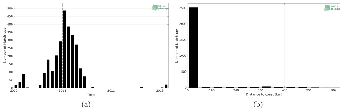
Figure 1: Number of match-ups between Marine mammals and CCI SSS L4 Merged-OI v3.2 - 30-day running (ESA) SSS as a function of time (a) and as function of the distance to coast (b) over the Arctic Ocean Pi-MEP region and for the full satellite product period.
