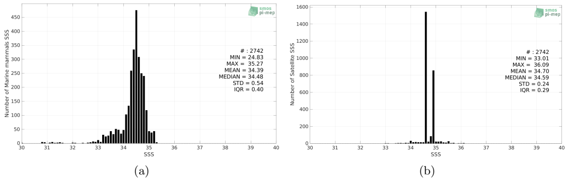
Figure 2: Histograms of SSS from Marine mammals (a) and CCI SSS L4 Merged-OI v3.2 - 30-day running (ESA) (b) considering all match-up pairs per bins of 0.1 over the Arctic Ocean Pi-MEP region and for the full satellite product period.
