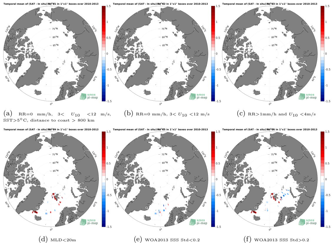
Figure 12: Temporal mean gridded over spatial boxes of size 1^{\circ}\times 1^{\circ} of \Delta\text{SSS} (CCI SSS L4 Merged-OI v3.2 - 30-day running (ESA) - Marine mammals) for 6 different subdatasets corresponding to: RR=0 mm/h, 3 < U_{10} < 12 m/s, SST > 5^{\circ}\text{C} , distance to coast > 800 km (a), RR=0 mm/h, 3 < U_{10} < 12 m/s (b), RR > 1\text{mm/h} and U_{10} < 4\text{m/s} (c), MLD < 20\text{m} (d), WOA2013 SSS Std < 0.2 (e), WOA2013 SSS Std > 0.2 (f).
