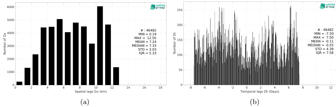
Figure 5: Histograms of the spatial (a) and temporal (b) lags between the location/time of the ICES measurement and the date of the corresponding CCI SSS L4 Merged-OI v3.2 - 30-day running (ESA) SSS pixel.
