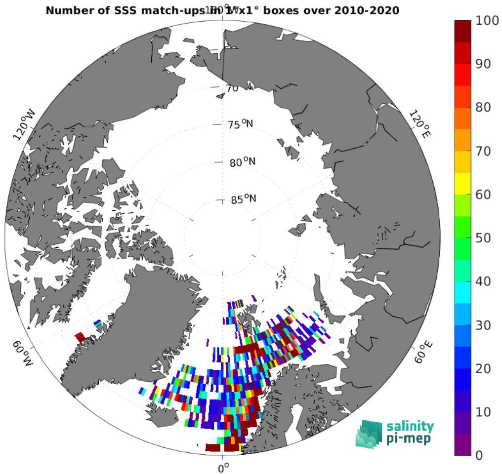
Figure 4: Number of SSS match-ups between ICES SSS and the CCI SSS L4 Merged-OI v3.2 - 30-day running (ESA) SSS product for the Arctic Ocean Pi-MEP region over 1^\circ \times 1^\circ boxes and for the full satellite product period.
