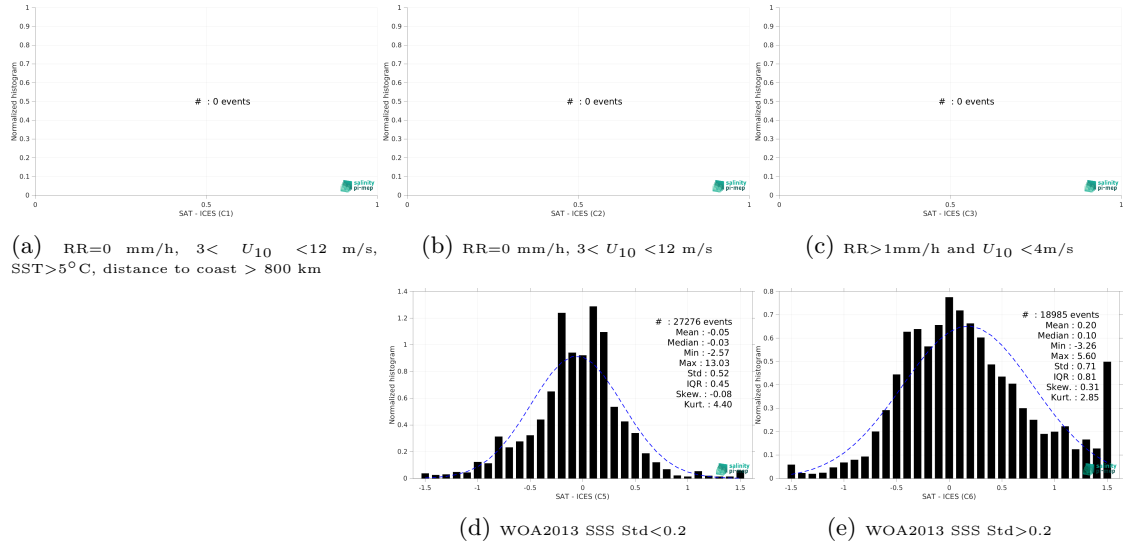
Figure 13: Normalized histogram of \Delta SSS (CCI SSS L4 Merged-OI v3.2 - 30-day running (ESA) - ICES) for 5 different subdatasets corresponding to: RR=0 mm/h, 3 < U_{10} < 12 m/s, SST >5^{\circ} C, distance to coast > 800 km (a), RR=0 mm/h, 3 < U_{10} < 12 m/s (b), RR >1 mm/h and U_{10} < 4 m/s (c), WOA2013 SSS Std <0.2 (d), WOA2013 SSS Std >0.2 (e).
