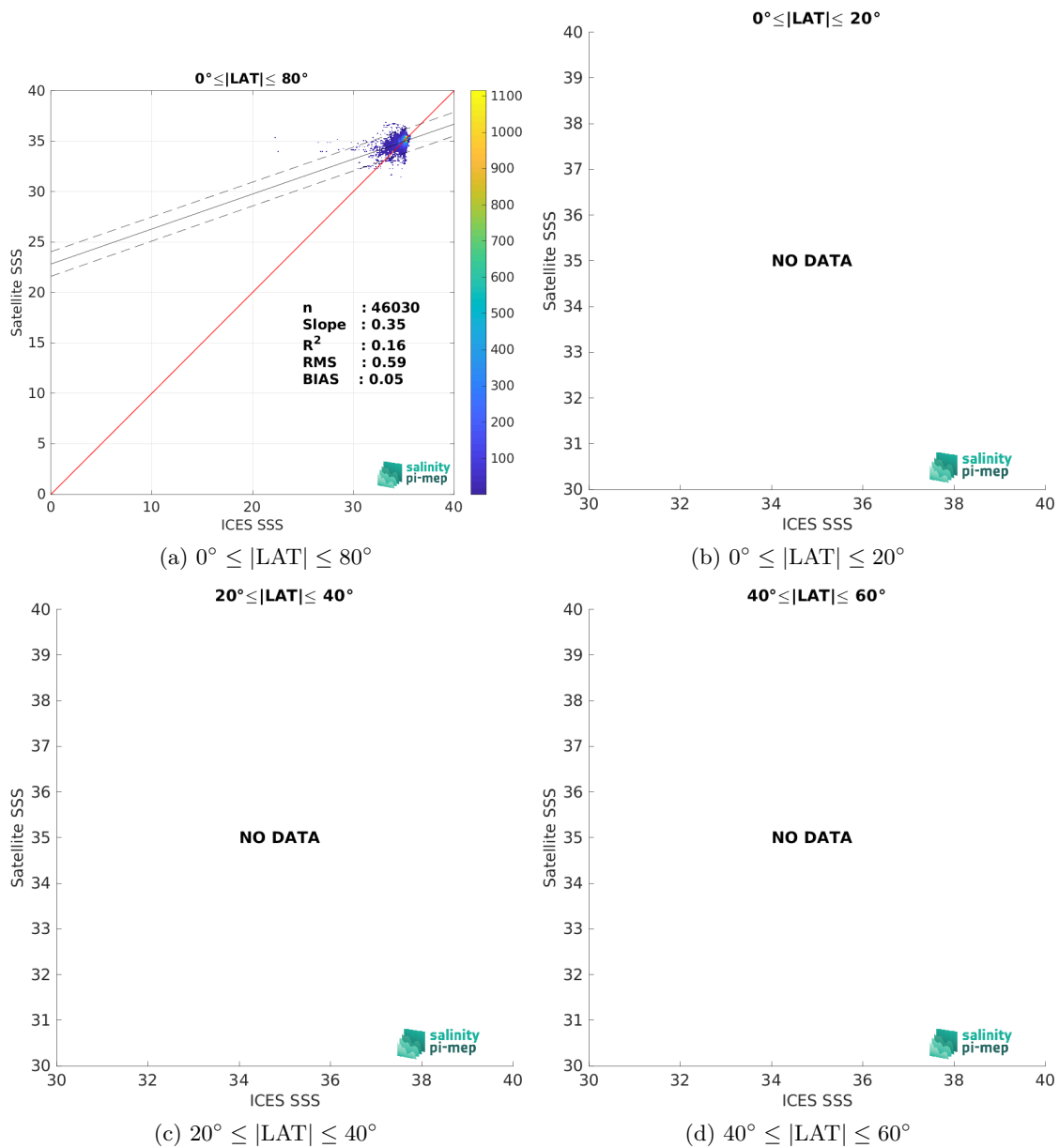
Figure 9: Contour maps of the concentration of CCI SSS L4 Merged-OI v3.2 - 30-day running (ESA) SSS (y-axis) versus ICES SSS (x-axis) at match-up pairs for different latitude bands. For each plot, the red line shows x=y . The black thin and dashed lines indicate a linear fit through the data cloud and the \pm 95\% confidence levels, respectively. The number match-up pairs n , the slope and R^2 coefficient of the linear fit, the root mean square (RMS) and the mean bias between satellite and in situ data are indicated for each latitude band in each plots.
