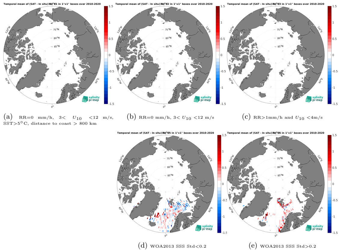
Figure 12: Temporal mean gridded over spatial boxes of size 1^{\circ}\times 1^{\circ} of \Delta\text{SSS} (CCI SSS L4 Merged-OI v3.2 - 30-day running (ESA) - ICES) for 5 different subdatasets corresponding to: RR=0 mm/h, 3 < U_{10} < 12 m/s, SST > 5^{\circ}\text{C} , distance to coast > 800 km (a), RR=0 mm/h, 3 < U_{10} < 12 m/s (b), RR > 1 mm/h and U_{10} < 4 m/s (c), WOA2013 SSS Std < 0.2 (d), WOA2013 SSS Std > 0.2 (e).
