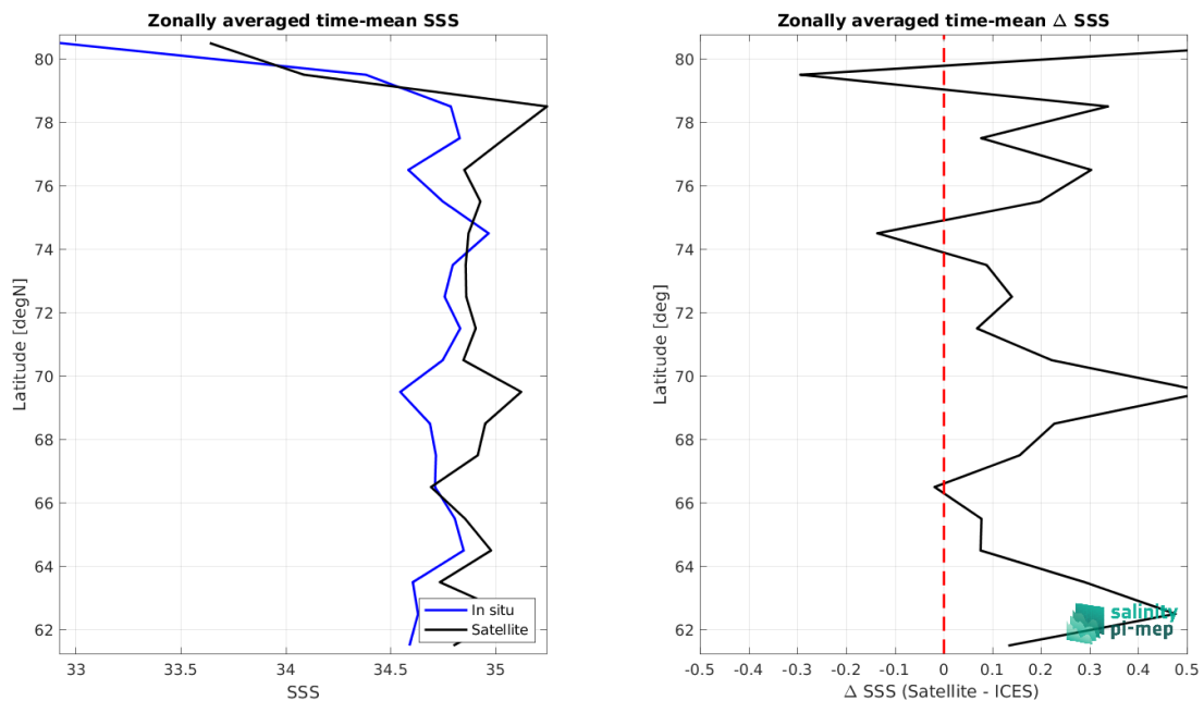
Figure 8: Left panel: Zonal mean SSS from CCI SSS L4 Merged-OI v3.2 - 30-day running (ESA) satellite product (black) and from ICES (blue). Right panel: Zonal mean of \Delta SSS (Satellite - ICES) for all the collected Pi-MEP match-up pairs estimated over the full satellite product period.
