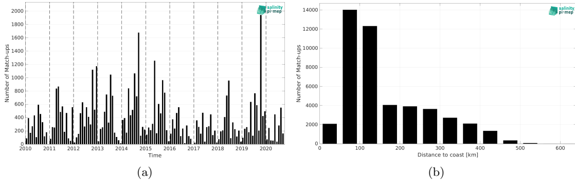
Figure 1: Number of match-ups between ICES and CCI SSS L4 Merged-OI v3.2 - 30-day running (ESA) SSS as a function of time (a) and as function of the distance to coast (b) over the Arctic Ocean Pi-MEP region and for the full satellite product period.
