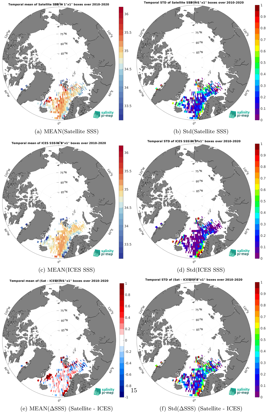
Figure 6: Temporal mean (left) and Std (right) of SSS from CCI SSS L4 Merged-OI v3.2 - 30-day running (ESA) (top), ICES (middle), and of \Delta SSS (Satellite - ICES). Only match-up pairs are used to generate these maps.
