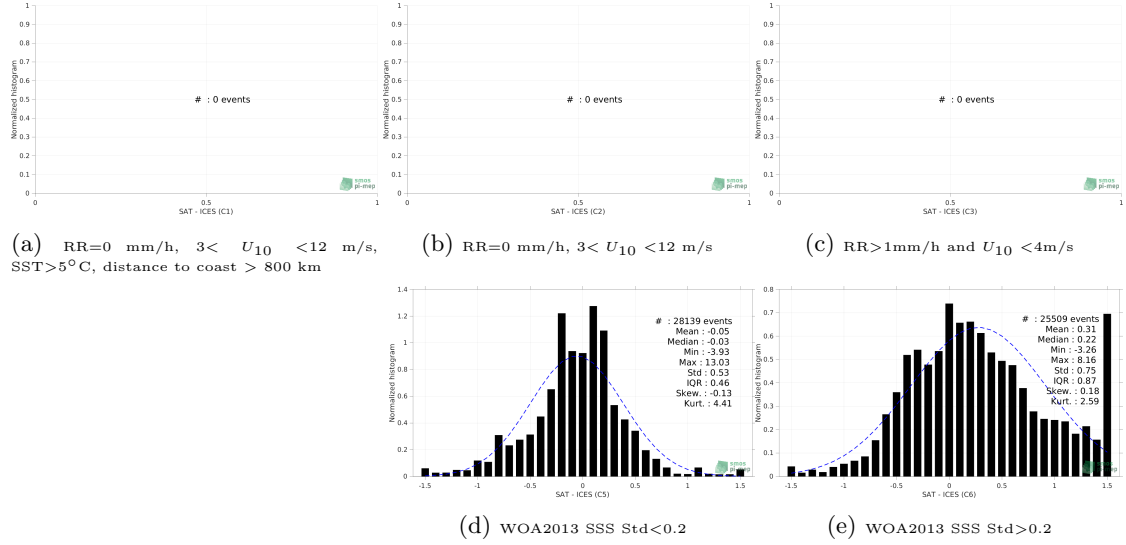
Figure 13: Normalized histogram of \Delta SSS (CCI SSS L4 Merged-OI v3.2 - 30-day running (ESA) - ICES) for 5 different subdatasets corresponding to: RR=0 mm/h, 3 < U_{10} < 12 m/s, SST>5°C, distance to coast > 800 km (a), RR=0 mm/h, 3 < U_{10} < 12 m/s (b), RR>1mm/h and U_{10} < 4 m/s (c), WOA2013 SSS Std<0.2 (d), WOA2013 SSS Std>0.2 (e).
