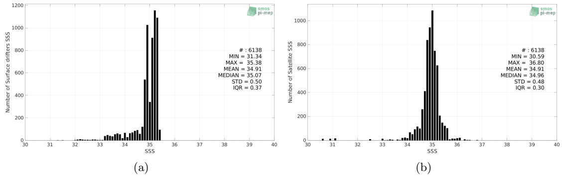
Figure 2: Histograms of SSS from Surface drifters (a) and CCI SSS L4 Merged-OI v3.2 - 30-day running (ESA) (b) considering all match-up pairs per bins of 0.1 over the Arctic Ocean Pi-MEP region and for the full satellite product period.
