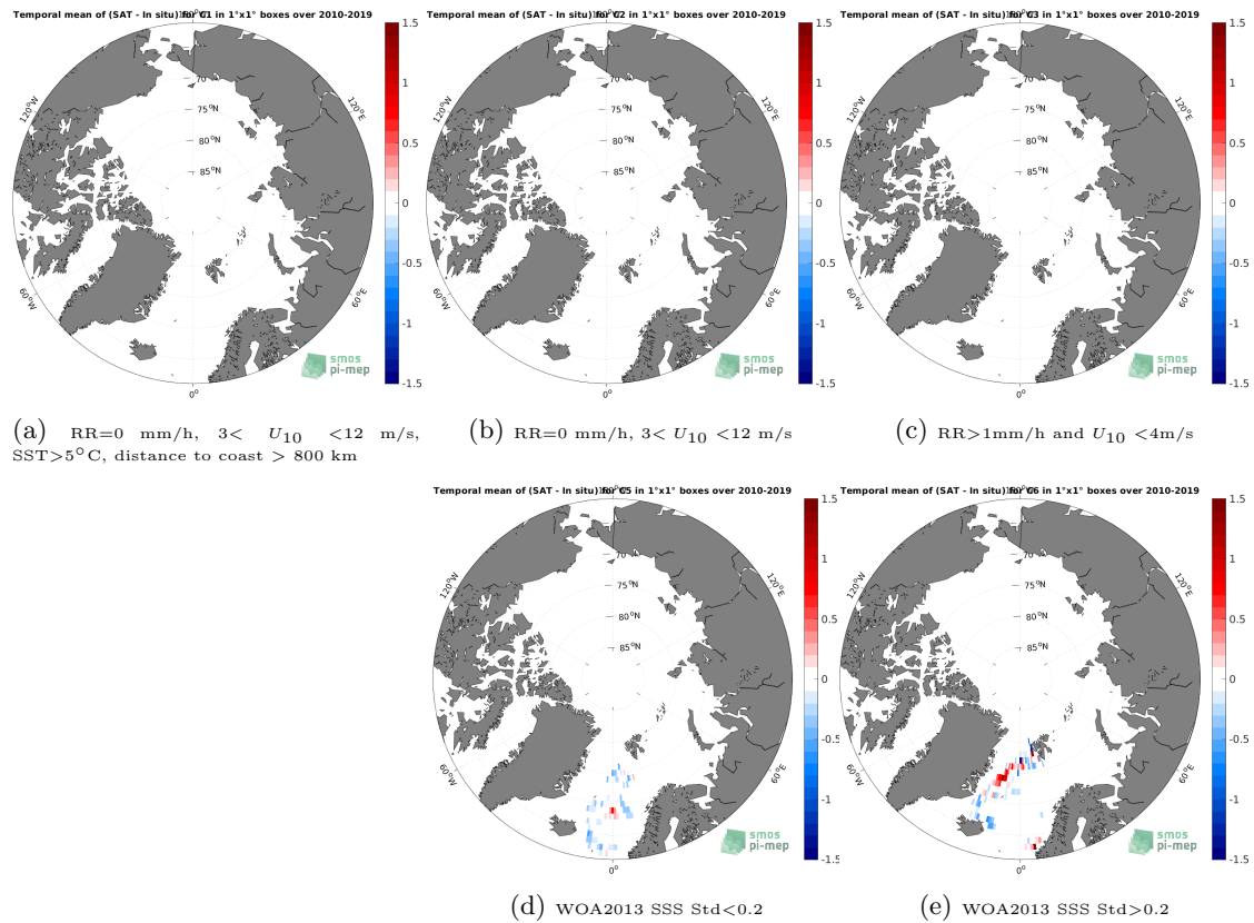
Figure 11: Temporal mean gridded over spatial boxes of size 1^{\circ}\times 1^{\circ} of \Delta\text{SSS} (CCI SSS L4 Merged-OI v3.2 - 30-day running (ESA) - Surface drifters) for 5 different subdatasets corresponding to: RR=0 mm/h, 3 < U_{10} < 12 m/s, SST > 5^{\circ}\text{C} , distance to coast > 800 km (a), RR=0 mm/h, 3 < U_{10} < 12 m/s (b), RR > 1 mm/h and U_{10} < 4 m/s (c), WOA2013 SSS Std < 0.2 (d), WOA2013 SSS Std > 0.2 (e).
