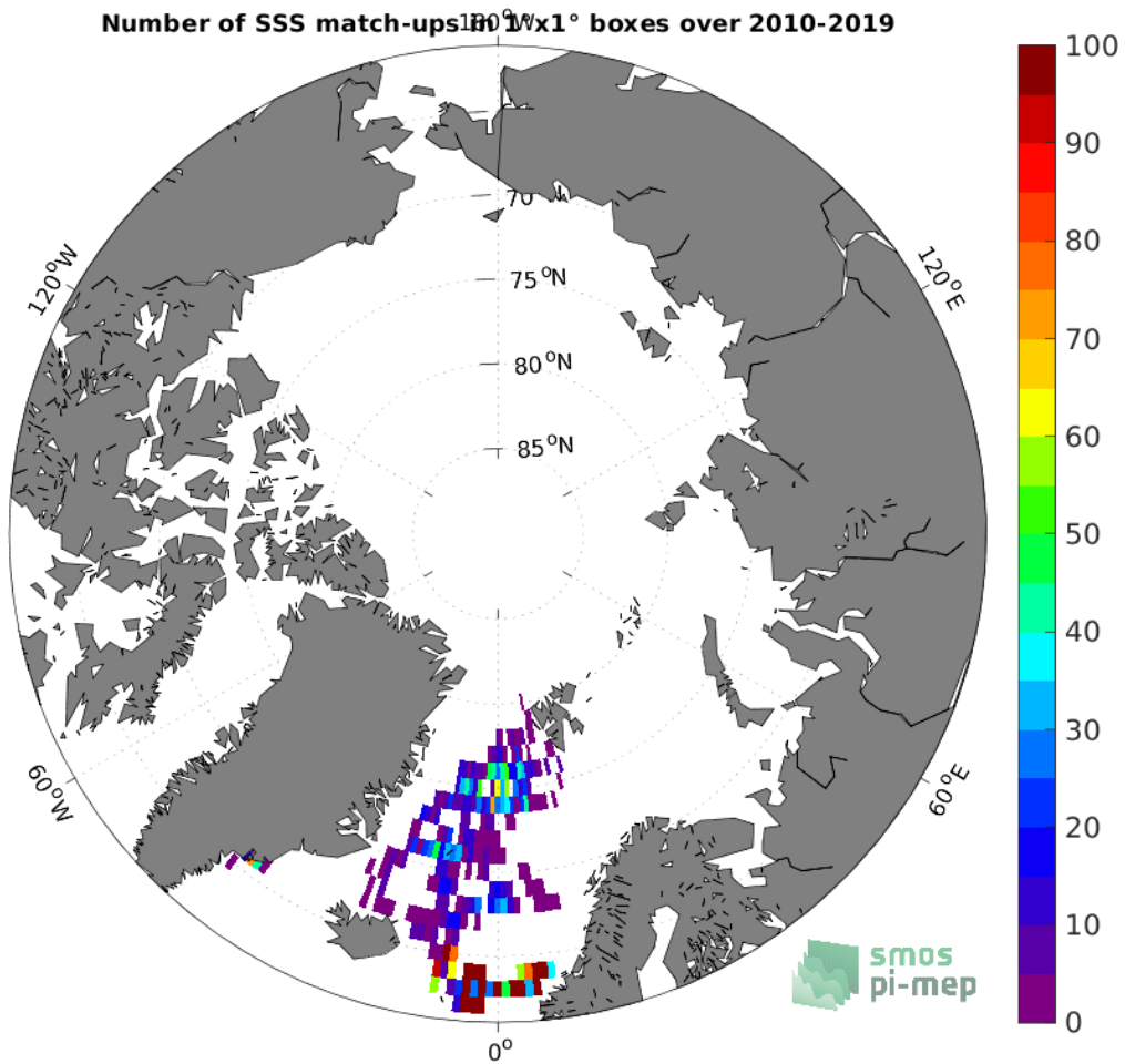
Figure 3: Number of SSS match-ups between Surface drifters SSS and the CCI SSS L4 Merged-OI v3.2 - 30-day running (ESA) SSS product for the Arctic Ocean Pi-MEP region over 1^{\circ} \times 1^{\circ} boxes and for the full satellite product period.
