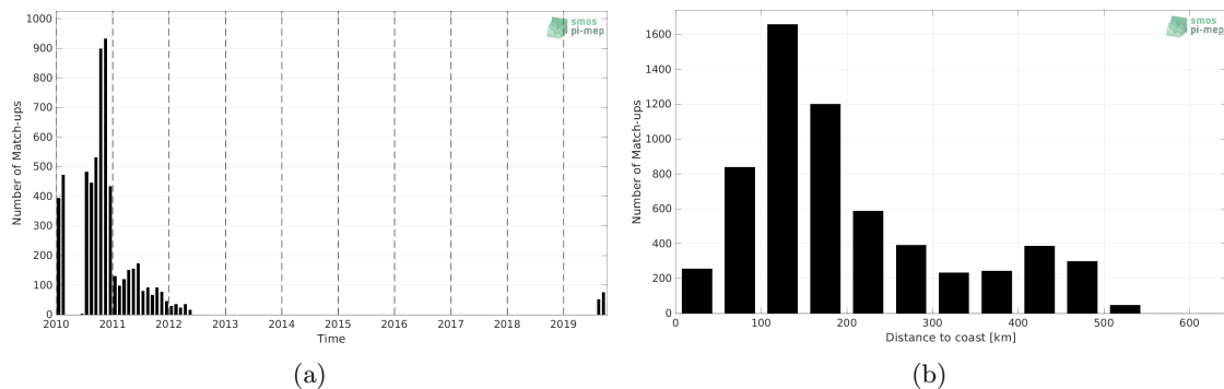
Figure 1: Number of match-ups between Surface drifters and CCI SSS L4 Merged-OI v3.2 - 30-day running (ESA) SSS as a function of time (a) and as function of the distance to coast (b) over the Arctic Ocean Pi-MEP region and for the full satellite product period.
