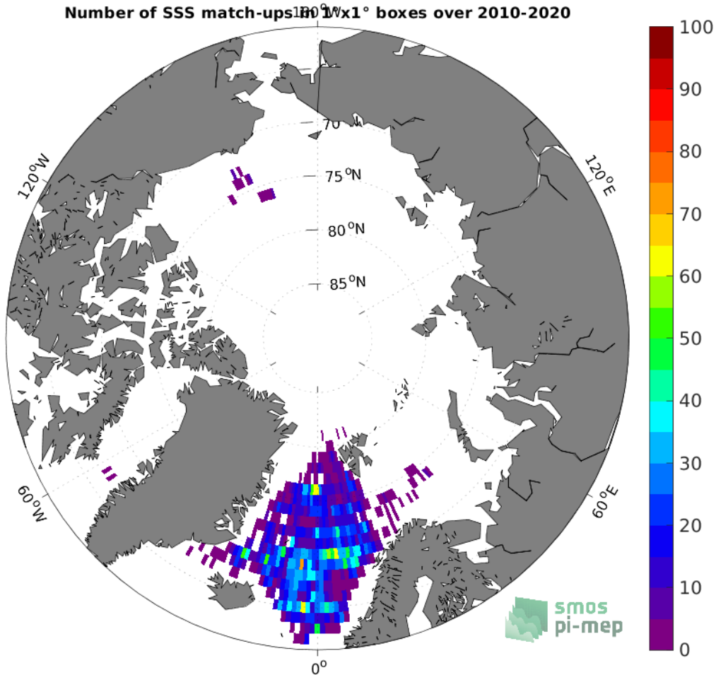
Figure 4: Number of SSS match-ups between Argo SSS and the CCI SSS L4 Merged-OI v3.2 - 30-day running (ESA) SSS product for the Arctic Ocean Pi-MEP region over 1^\circ \times 1^\circ boxes and for the full satellite product period.
