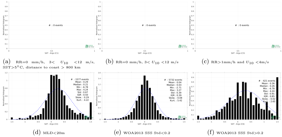
Figure 13: Normalized histogram of \Delta\text{SSS} (CCI SSS L4 Merged-OI v3.2 - 30-day running (ESA) - Argo) for 6 different subdatasets corresponding to: RR=0 mm/h, 3 < U_{10} < 12 m/s, SST > 5^{\circ}\text{C} , distance to coast > 800 km (a), RR=0 mm/h, 3 < U_{10} < 12 m/s (b), RR > 1\text{mm/h} and U_{10} < 4\text{m/s} (c), MLD < 20\text{m} (d), WOA2013 SSS Std < 0.2 (e), WOA2013 SSS Std > 0.2 (f).
