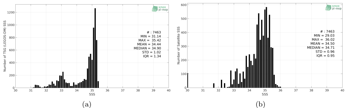
Figure 2: Histograms of SSS from TSG (LEGOS-DM) (a) and CCI L4 Merged-OI v2.31 - 30-day running (ESA) (b) considering all match-up pairs per bins of 0.1 over the Arctic Ocean Pi-MEP region and for the full satellite product period.
