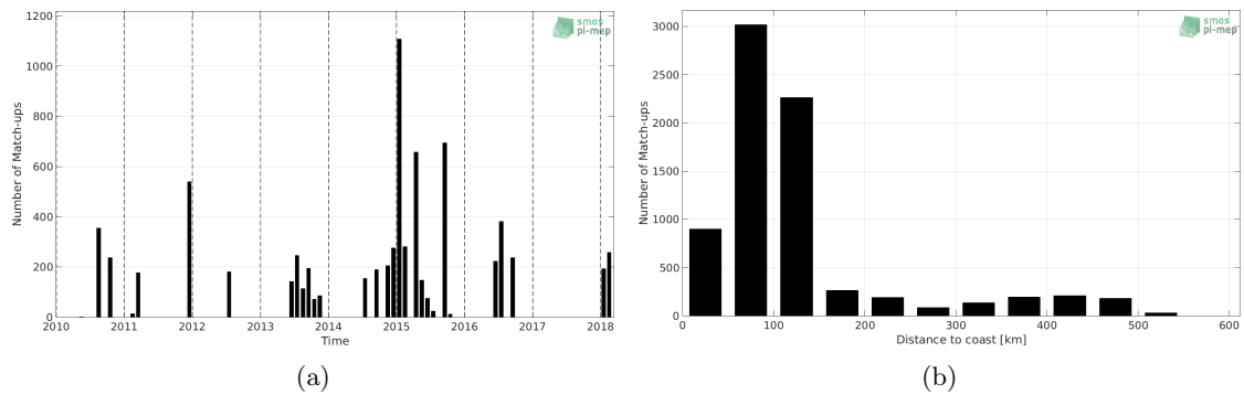
Figure 1: Number of match-ups between TSG (LEGOS-DM) and CCI L4 Merged-OI v2.31 - 30-day running (ESA) SSS as a function of time (a) and as function of the distance to coast (b) over the Arctic Ocean Pi-MEP region and for the full satellite product period.
