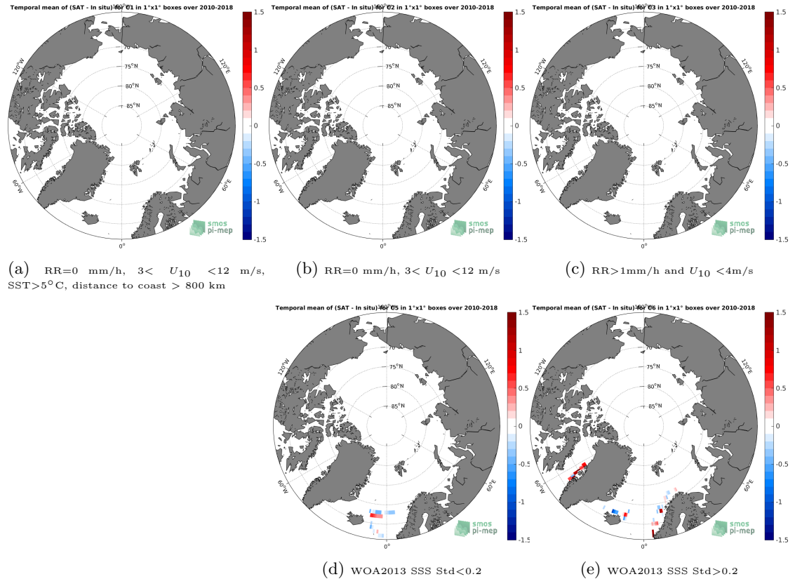
Figure 12: Temporal mean gridded over spatial boxes of size 1^{\circ}\times 1^{\circ} of \Delta\text{SSS} (CCI L4 Merged-OI v2.31 - 30-day running (ESA) - TSG (LEGOS-DM)) for 5 different subdatasets corresponding to:RR=0 mm/h, 3 < U_{10} < 12 m/s, SST >5^{\circ}\text{C} , distance to coast > 800 km (a), RR=0 mm/h, 3 < U_{10} < 12 m/s (b), RR >1 mm/h and U_{10} < 4 m/s (c), WOA2013 SSS Std <0.2 (d), WOA2013 SSS Std >0.2 (e).
