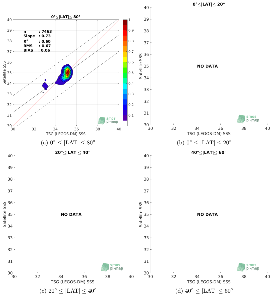
Figure 9: Contour maps of the concentration of CCI L4 Merged-OI v2.31 - 30-day running (ESA) SSS (y-axis) versus TSG (LEGOS-DM) SSS (x-axis) at match-up pairs for different latitude bands. For each plot, the red line shows x=y . The black thin and dashed lines indicate a linear fit through the data cloud and the \pm 95\% confidence levels, respectively. The number match-up pairs n , the slope and R^2 coefficient of the linear fit, the root mean square (RMS) and the mean bias between satellite and in situ data are indicated for each latitude band in each plots.
