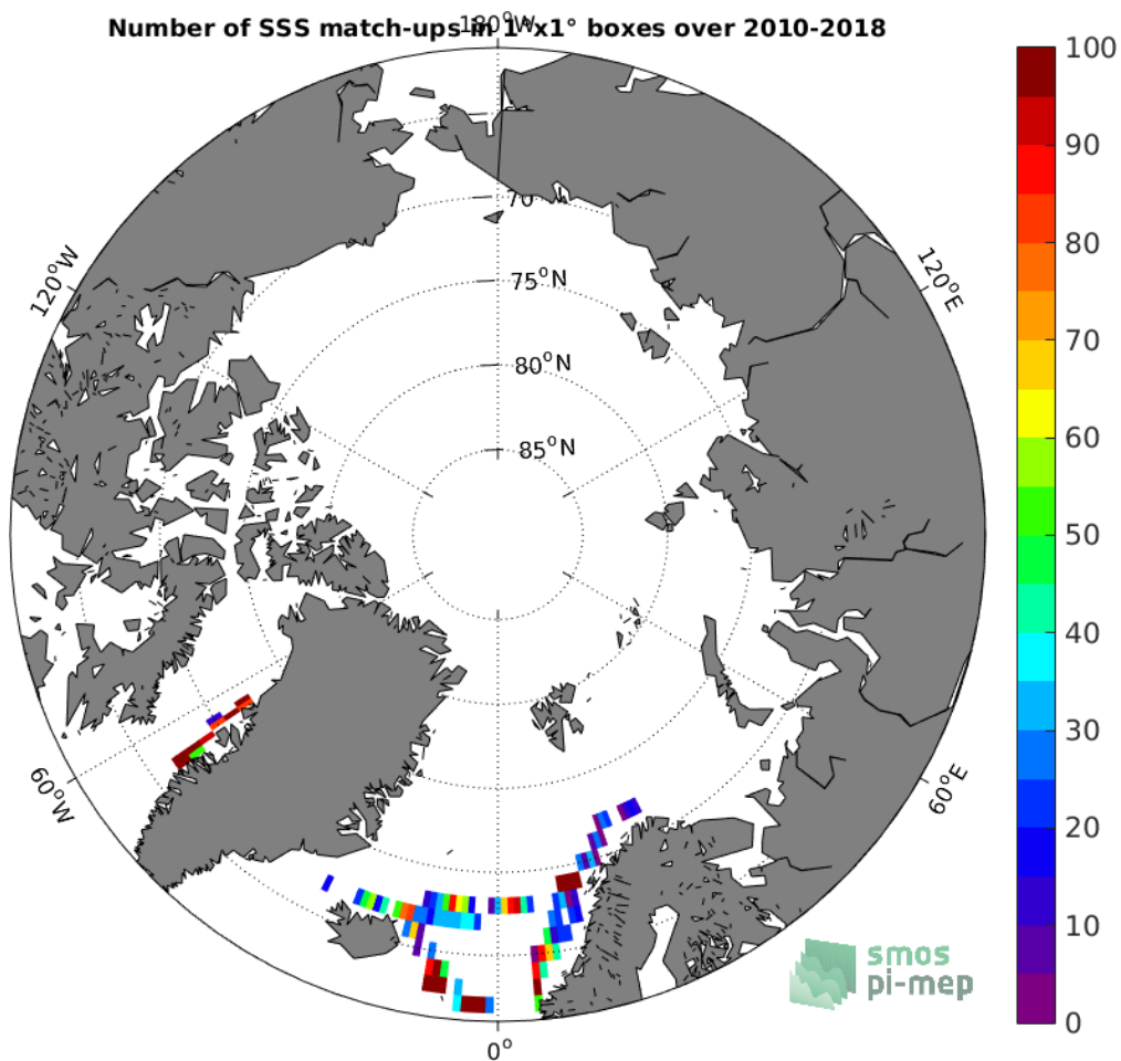
Figure 4: Number of SSS match-ups between TSG (LEGOS-DM) SSS and the CCI L4 Merged-OI v2.31 - 30-day running (ESA) SSS product for the Arctic Ocean Pi-MEP region over 1°x1° boxes and for the full satellite product period.
