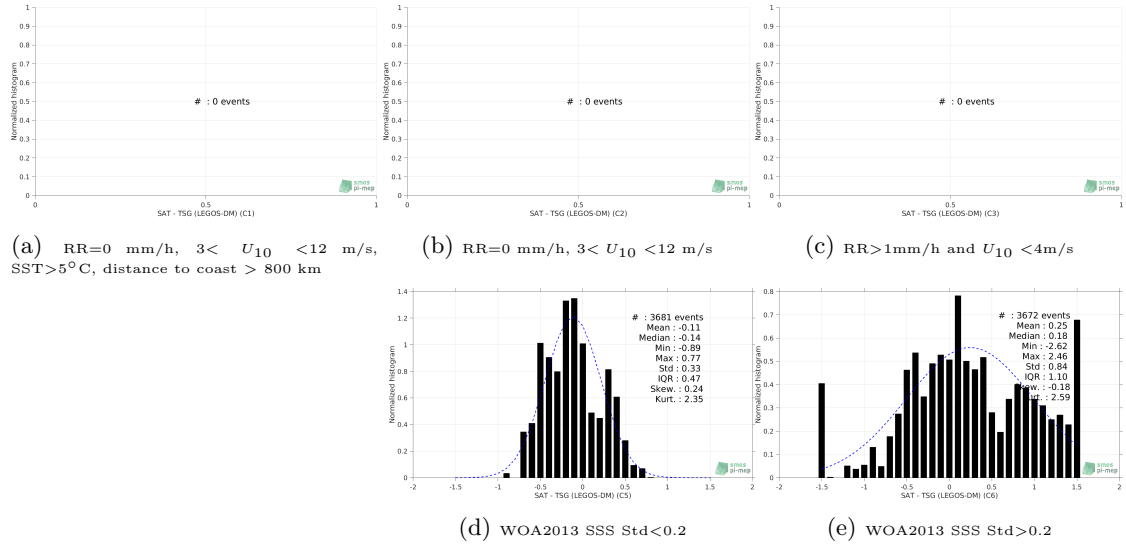
Figure 13: Normalized histogram of \Delta SSS (CCI L4 Merged-OI v2.31 - 30-day running (ESA) - TSG (LEGOS-DM)) for 5 different subdatasets corresponding to: RR=0 mm/h, 3 < U_{10} < 12 m/s, SST>5°C, distance to coast > 800 km (a), RR=0 mm/h, 3 < U_{10} < 12 m/s (b), RR>1mm/h and U_{10} < 4 m/s (c), WOA2013 SSS Std<0.2 (d), WOA2013 SSS Std>0.2 (e).
