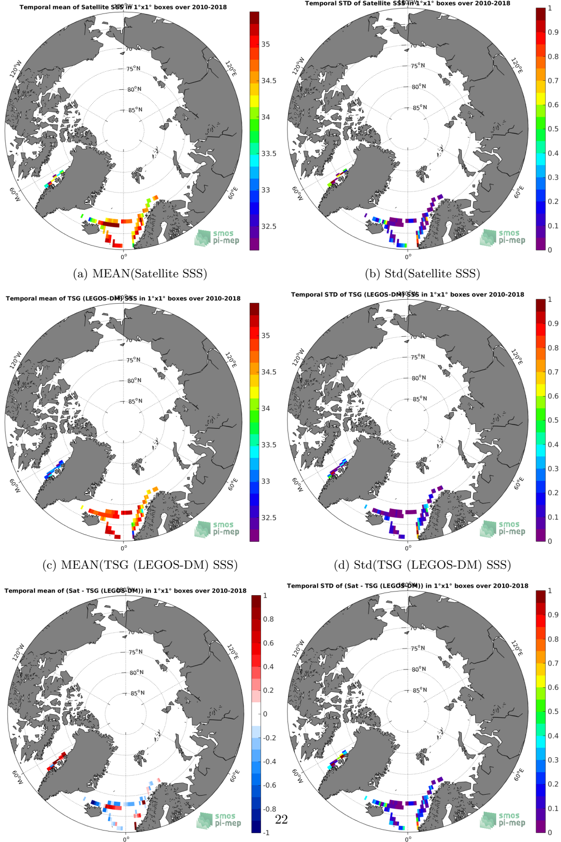
Figure 6: Temporal mean (left) and Std (right) of SSS from CCI L4 Merged-OI v2.31 - 30-day running (ESA) (top), TSG (LEGOS-DM) (middle), and of \Delta SSS (Satellite - TSG (LEGOS-DM)). Only match-up pairs are used to generate these maps.
