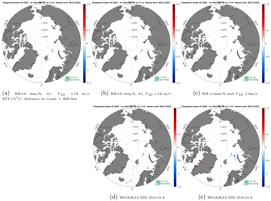
Figure 12: Temporal mean gridded over spatial boxes of size 1°x1° of \Delta SSS (CCI SSS L4 Merged-OI v2.31 - 30-day running (ESA) - TSG (GOSUD-Sailing-ship)) for 5 different subdatasets corresponding to:RR=0 mm/h, 3 < U_{10} < 12 m/s, SST>5°C, distance to coast > 800 km (a), RR=0 mm/h, 3 < U_{10} < 12 m/s (b), RR>1mm/h and U_{10} < 4 m/s (c), WOA2013 SSS Std<0.2 (d), WOA2013 SSS Std>0.2 (e).
