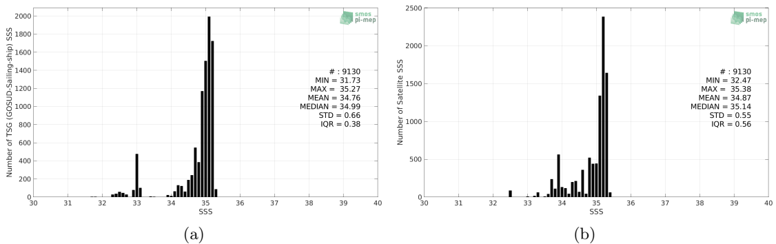
Figure 2: Histograms of SSS from TSG (GOSUD-Sailing-ship) (a) and CCI SSS L4 Merged-OI v2.31 - 30-day running (ESA) (b) considering all match-up pairs per bins of 0.1 over the Arctic Ocean Pi-MEP region and for the full satellite product period.
