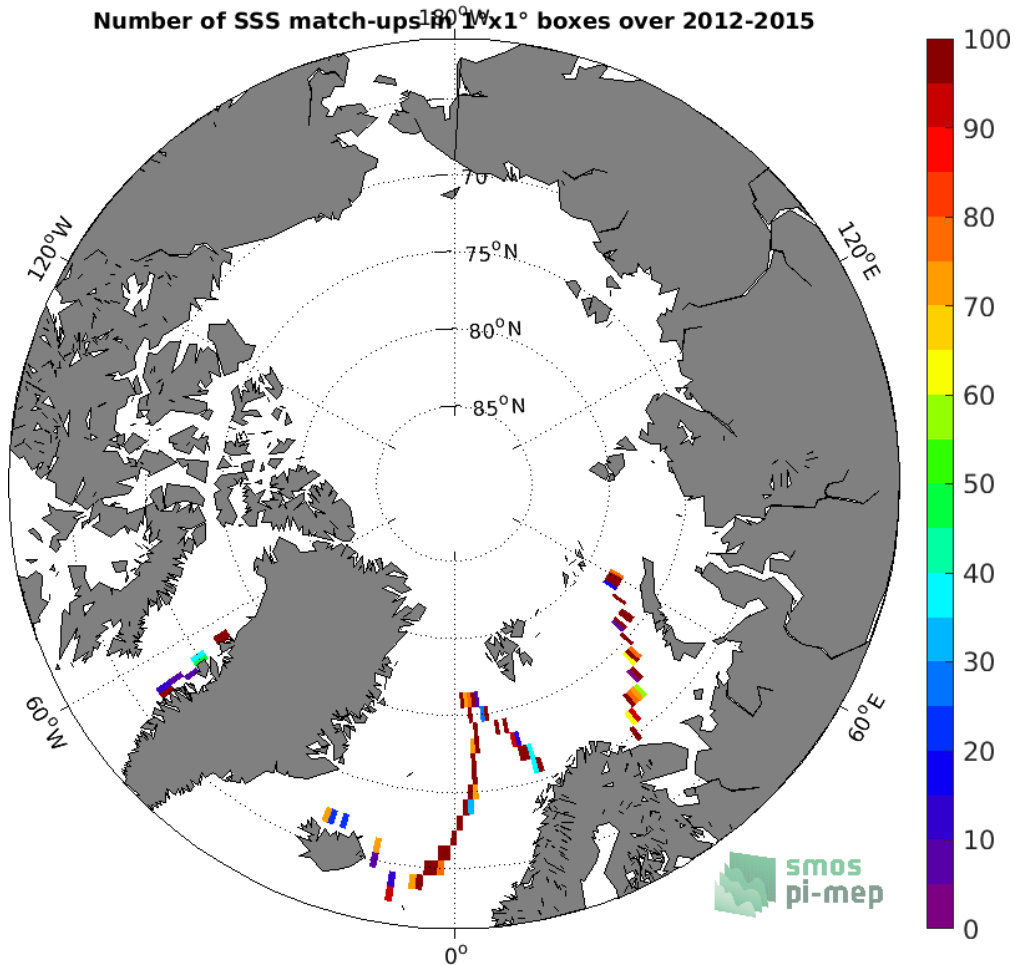
Figure 4: Number of SSS match-ups between TSG (GOSUD-Sailing-ship) SSS and the CCI SSS L4 Merged-OI v2.31 - 30-day running (ESA) SSS product for the Arctic Ocean Pi-MEP region over 1°x1° boxes and for the full satellite product period.
