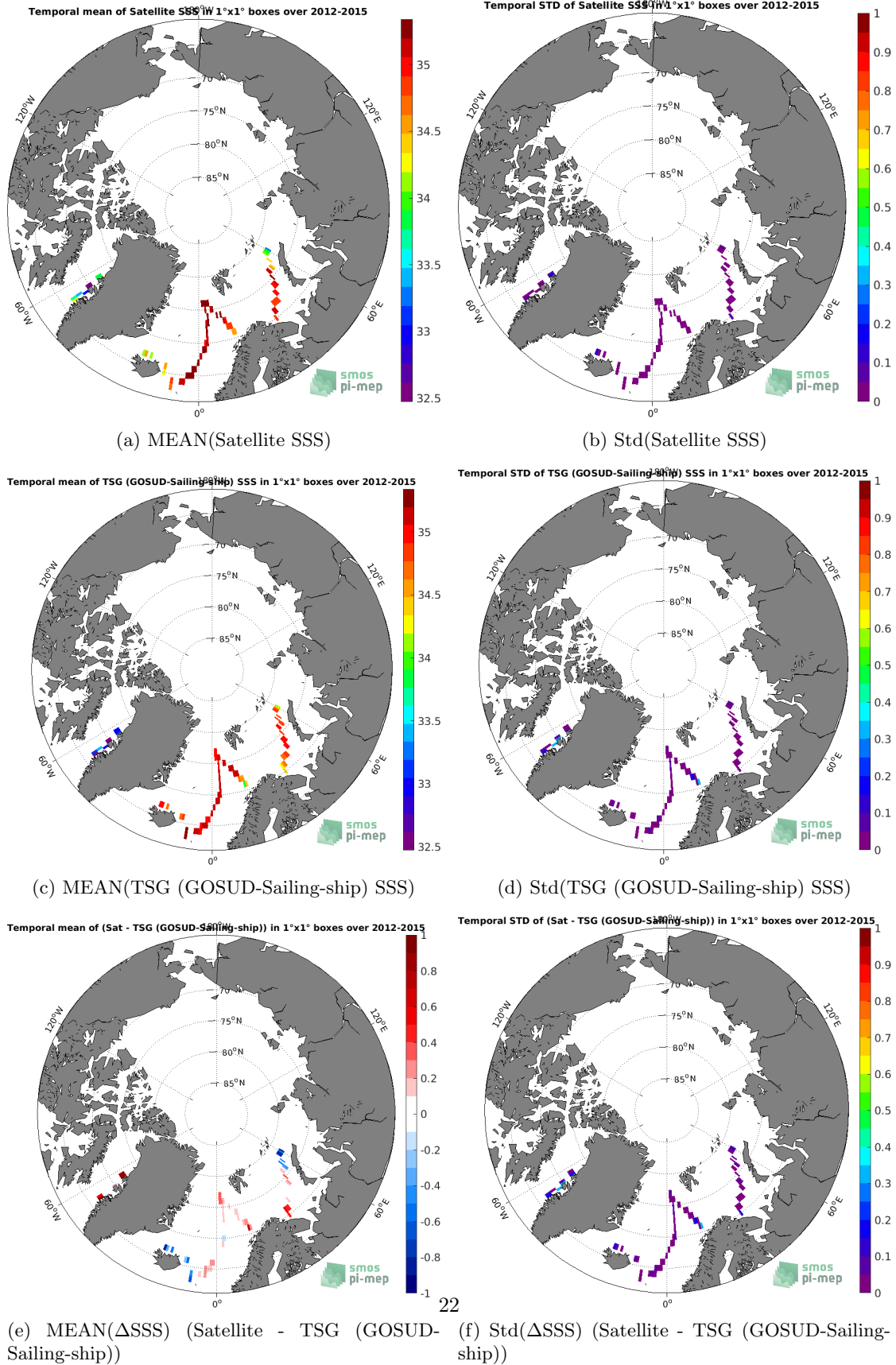
Figure 6: Temporal mean (left) and Std (right) of SSS from CCI SSS L4 Merged-OI v2.31 - 30-day running (ESA) (top), TSG (GOSUD-Sailing-ship) (middle), and of \Delta SSS (Satellite - TSG (GOSUD-Sailing-ship)). Only match-up pairs are used to generate these maps.
