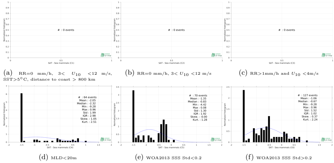
Figure 13: Normalized histogram of \Delta SSS (CCI L4 Merged-OI v2.31 - 30-day running (ESA) - Sea mammals) for 6 different subdatasets corresponding to: RR=0 mm/h, 3 < U_{10} < 12 m/s, SST > 5°C, distance to coast > 800 km (a), RR=0 mm/h, 3 < U_{10} < 12 m/s (b), RR > 1mm/h and U_{10} < 4 m/s (c), MLD < 20m (d), WOA2013 SSS Std < 0.2 (e), WOA2013 SSS Std > 0.2 (f).
