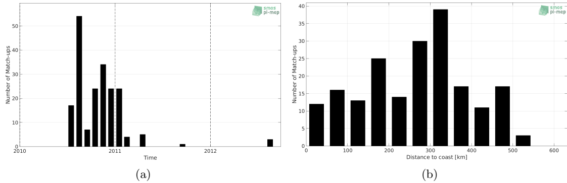
Figure 1: Number of match-ups between Sea mammals and CCI L4 Merged-OI v2.31 - 30-day running (ESA) SSS as a function of time (a) and as function of the distance to coast (b) over the Arctic Ocean Pi-MEP region and for the full satellite product period.
