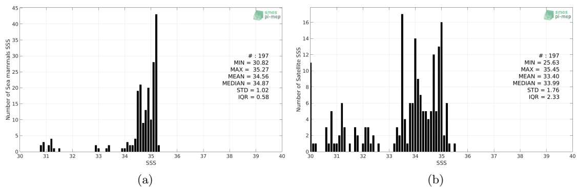
Figure 2: Histograms of SSS from Sea mammals (a) and CCI L4 Merged-OI v2.31 - 30-day running (ESA) (b) considering all match-up pairs per bins of 0.1 over the Arctic Ocean Pi-MEP region and for the full satellite product period.
