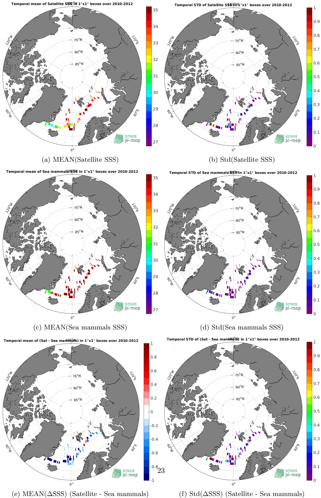
Figure 6: Temporal mean (left) and Std (right) of SSS from CCI L4 Merged-OI v2.31 - 30-day running (ESA) (top), Sea mammals (middle), and of \Delta SSS (Satellite - Sea mammals). Only match-up pairs are used to generate these maps.
