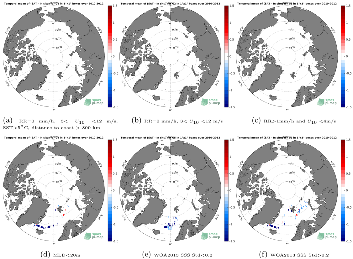
Figure 12: Temporal mean gridded over spatial boxes of size 1^{\circ}\times 1^{\circ} of \Delta\text{SSS} (CCI L4 Merged-OI v2.31 - 30-day running (ESA) - Sea mammals) for 6 different subdatasets corresponding to:RR=0 mm/h, 3 < U_{10} < 12 m/s, SST > 5^{\circ}\text{C} , distance to coast > 800 km (a), RR=0 mm/h, 3 < U_{10} < 12 m/s (b), RR > 1 mm/h and U_{10} < 4 m/s (c),MLD < 20 m (d),WOA2013 SSS Std < 0.2 (e),WOA2013 SSS Std > 0.2 (f).
