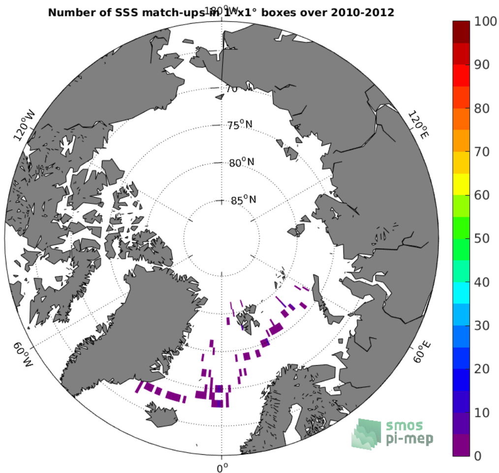
Figure 4: Number of SSS match-ups between Sea mammals SSS and the CCI L4 Merged-OI v2.31 - 30-day running (ESA) SSS product for the Arctic Ocean Pi-MEP region over 1°x1° boxes and for the full satellite product period.
