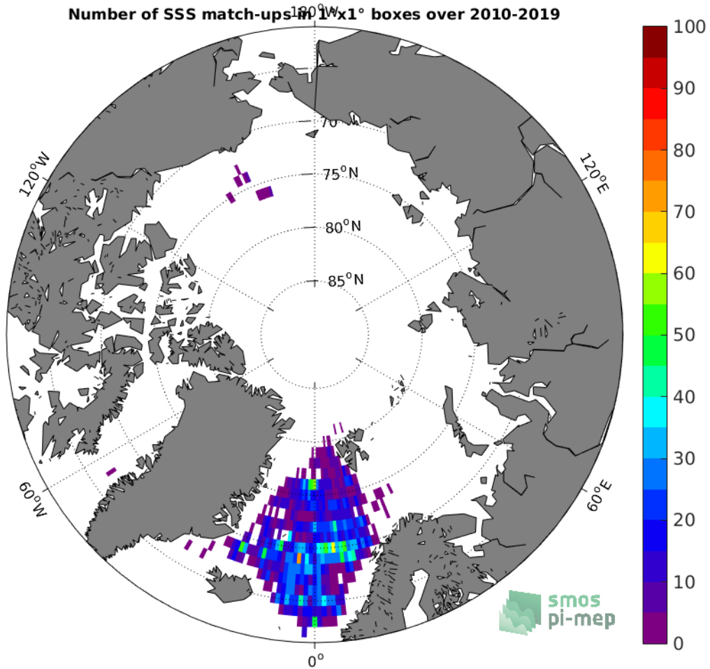
Figure 4: Number of SSS match-ups between Argo SSS and the CCI SSS L4 Merged-OI v2.31 - 30-day running (ESA) SSS product for the Arctic Ocean Pi-MEP region over 1°x1° boxes and for the full satellite product period.
