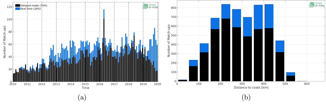
Figure 1: Number of match-ups between Argo and CCI SSS L4 Merged-OI v2.31 - 30-day running (ESA) SSS as a function of time (a) and as function of the distance to coast (b) over the Arctic Ocean Pi-MEP region and for the full satellite product period.
