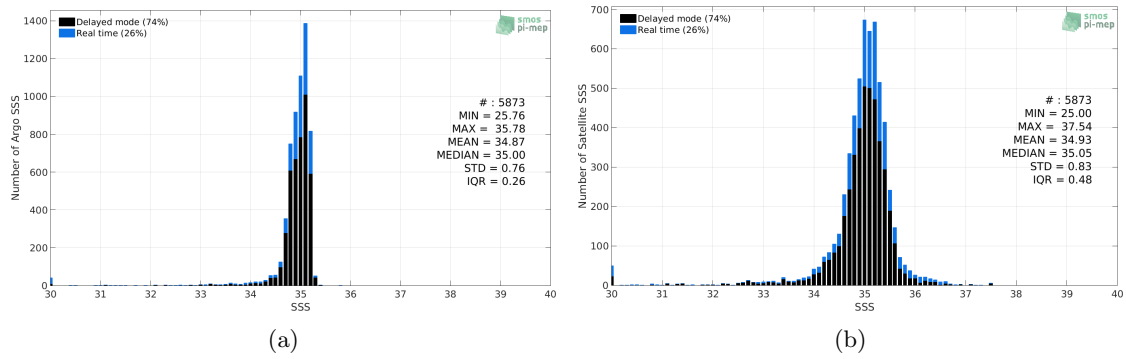
Figure 2: Histograms of SSS from Argo (a) and CCI SSS L4 Merged-OI v2.31 - 30-day running (ESA) (b) considering all match-up pairs per bins of 0.1 over the Arctic Ocean Pi-MEP region and for the full satellite product period.
