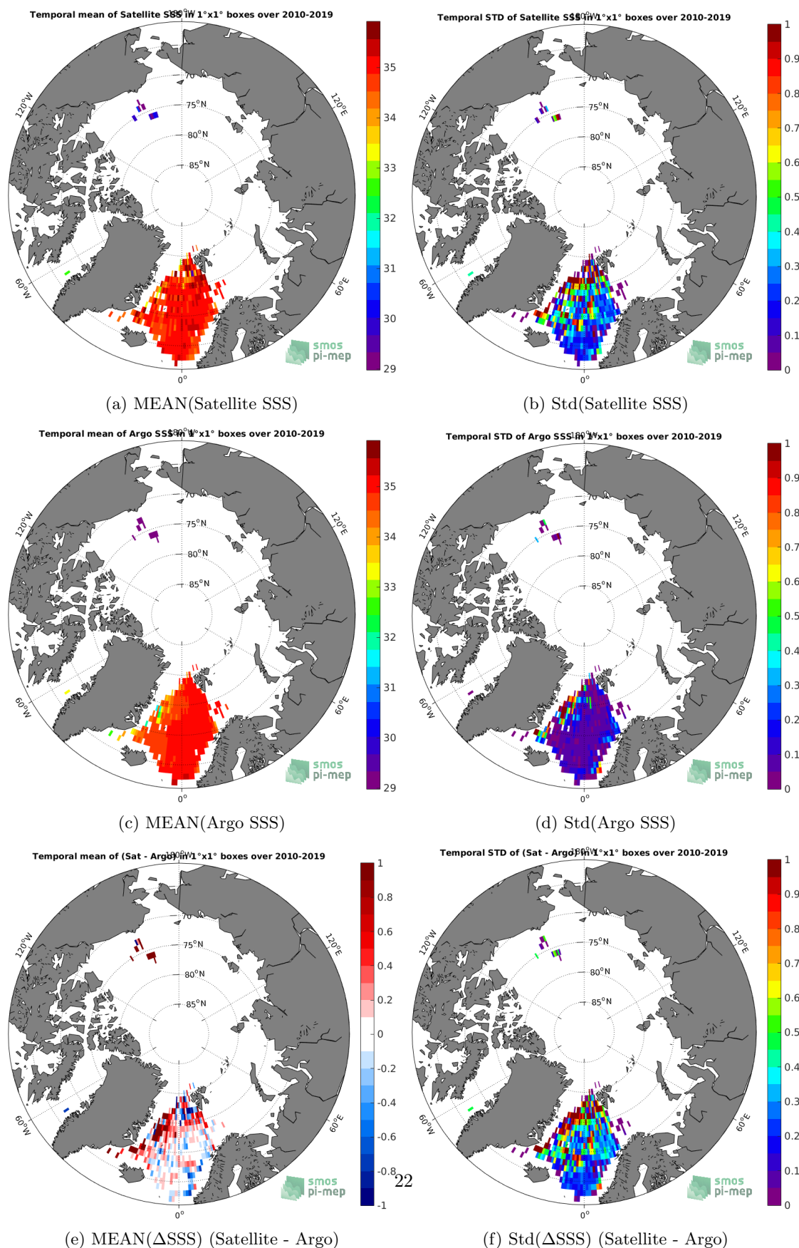
Figure 6: Temporal mean (left) and Std (right) of SSS from CCI L4 Merged-OI v2.31 - 30-day running (ESA) (top), Argo (middle), and of \Delta SSS (Satellite - Argo). Only match-up pairs are used to generate these maps.
