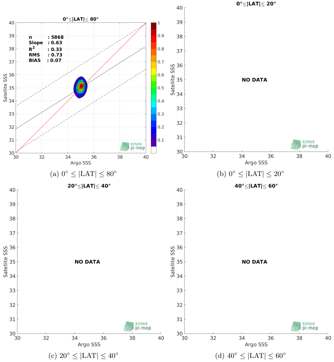
Figure 9: Contour maps of the concentration of CCI L4 Merged-OI v2.31 - 30-day running (ESA) SSS (y-axis) versus Argo SSS (x-axis) at match-up pairs for different latitude bands. For each plot, the red line shows x=y . The black thin and dashed lines indicate a linear fit through the data cloud and the \pm 95\% confidence levels, respectively. The number match-up pairs n , the slope and R^2 coefficient of the linear fit, the root mean square (RMS) and the mean bias between satellite and in situ data are indicated for each latitude band in each plots.
