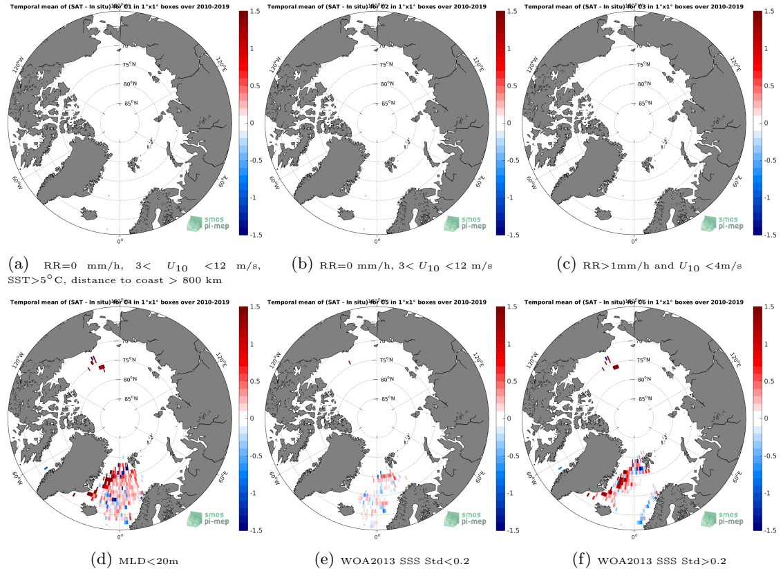
Figure 12: Temporal mean gridded over spatial boxes of size 1^{\circ}\times 1^{\circ} of \Delta\text{SSS} (CCI L4 Merged-OI v2.31 - 30-day running (ESA) - Argo) for 6 different subdatasets corresponding to:RR=0 mm/h, 3 < U_{10} < 12 m/s, SST >5^{\circ}\text{C} , distance to coast > 800 km (a), RR=0 mm/h, 3 < U_{10} < 12 m/s (b), RR >1 mm/h and U_{10} < 4 m/s (c),MLD <20 m (d),WOA2013 SSS Std <0.2 (e),WOA2013 SSS Std >0.2 (f).
