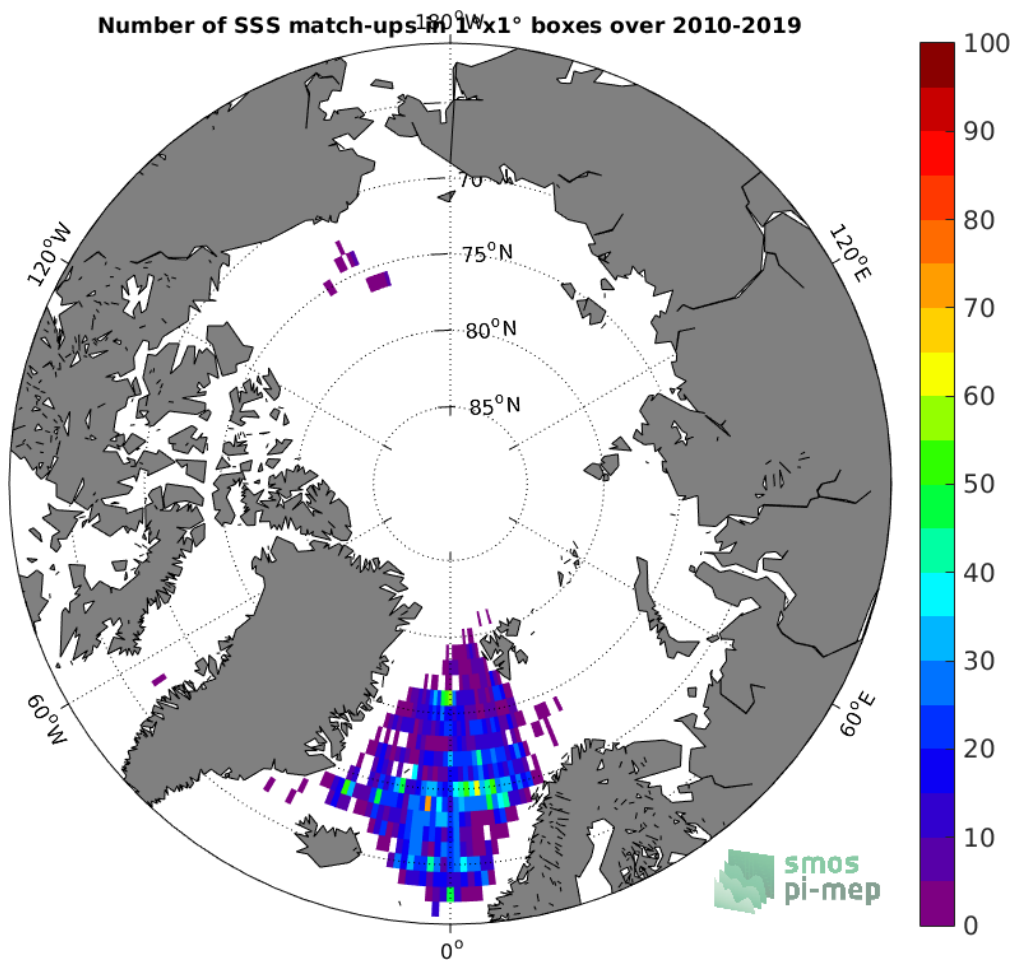
Figure 4: Number of SSS match-ups between Argo SSS and the CCI L4 Merged-OI v2.31 - 30-day running (ESA) SSS product for the Arctic Ocean Pi-MEP region over 1°x1° boxes and for the full satellite product period.
