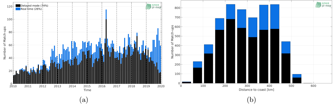
Figure 1: Number of match-ups between Argo and CCI L4 Merged-OI v2.31 - 30-day running (ESA) SSS as a function of time (a) and as function of the distance to coast (b) over the Arctic Ocean Pi-MEP region and for the full satellite product period.
