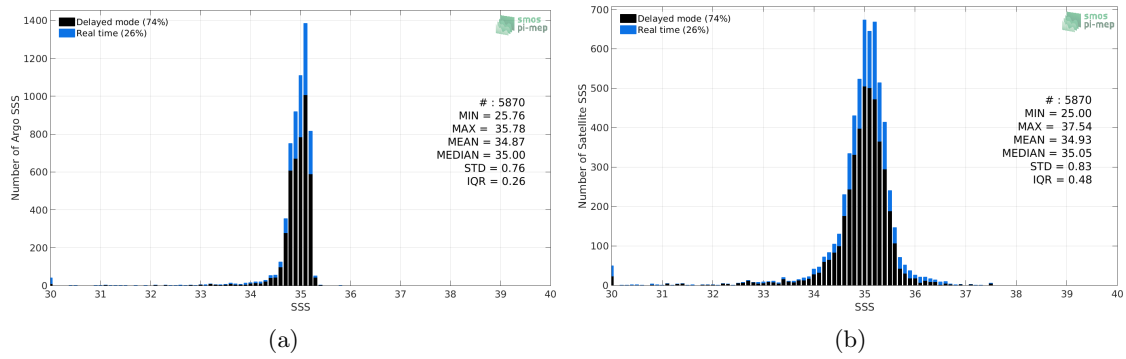
Figure 2: Histograms of SSS from Argo (a) and CCI L4 Merged-OI v2.31 - 30-day running (ESA) (b) considering all match-up pairs per bins of 0.1 over the Arctic Ocean Pi-MEP region and for the full satellite product period.
