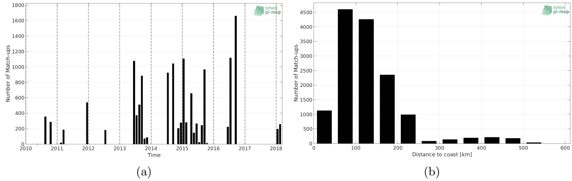
Figure 1: Number of match-ups between TSG-LEGOS-DM and CCI L4 Merged-OI v1.8 - 30-day running (ESA) SSS as a function of time (a) and as function of the distance to coast (b) over the Arctic Ocean Pi-MEP region and for the full satellite product period.
