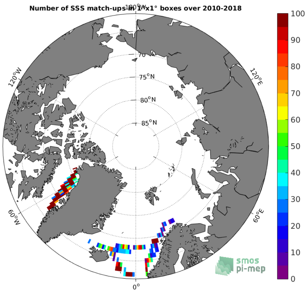
Figure 4: Number of SSS match-ups between TSG-LEGOS-DM SSS and the CCI L4 Merged-OI v1.8 - 30-day running (ESA) SSS product for the Arctic Ocean Pi-MEP region over 1°x1° boxes and for the full satellite product period.
