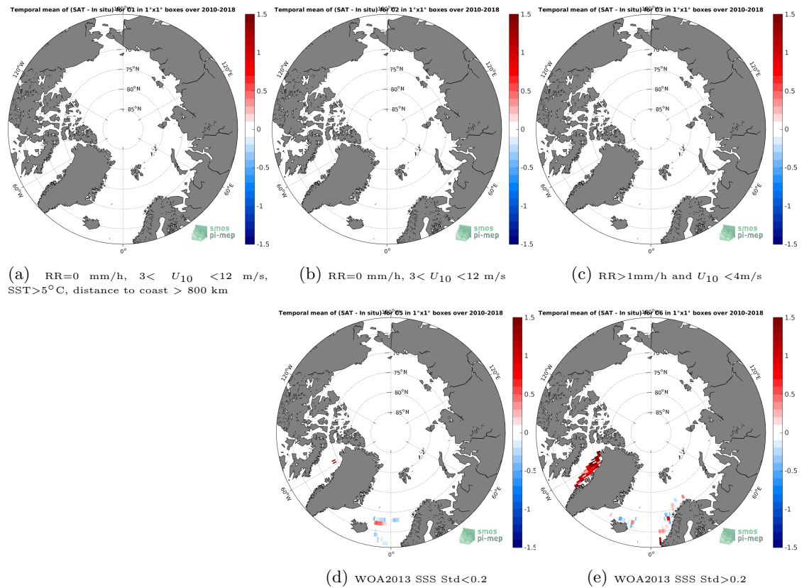
Figure 12: Temporal mean gridded over spatial boxes of size 1^{\circ}\times 1^{\circ} of \Delta\text{SSS} (CCI L4 Merged-OI v1.8 - 30-day running (ESA) - TSG-LEGOS-DM) for 5 different subdatasets corresponding to: RR=0 mm/h, 3 < U_{10} < 12 m/s, SST > 5^{\circ}\text{C} , distance to coast > 800 km (a), RR=0 mm/h, 3 < U_{10} < 12 m/s (b), RR > 1 mm/h and U_{10} < 4 m/s (c), WOA2013 SSS Std < 0.2 (d), WOA2013 SSS Std > 0.2 (e).
