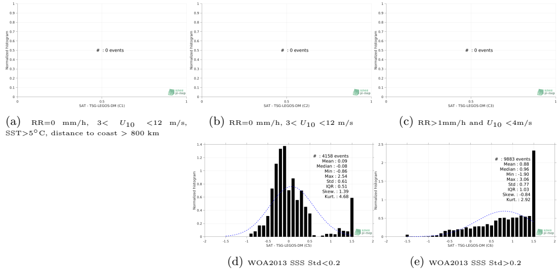
Figure 13: Normalized histogram of \Delta SSS (CCI L4 Merged-OI v1.8 - 30-day running (ESA) - TSG-LEGOS-DM) for 5 different subdatasets corresponding to: RR=0 mm/h, 3 < U_{10} < 12 m/s, SST>5°C, distance to coast > 800 km (a), RR=0 mm/h, 3 < U_{10} < 12 m/s (b), RR>1mm/h and U_{10} < 4 m/s (c), WOA2013 SSS Std<0.2 (d), WOA2013 SSS Std>0.2 (e).
