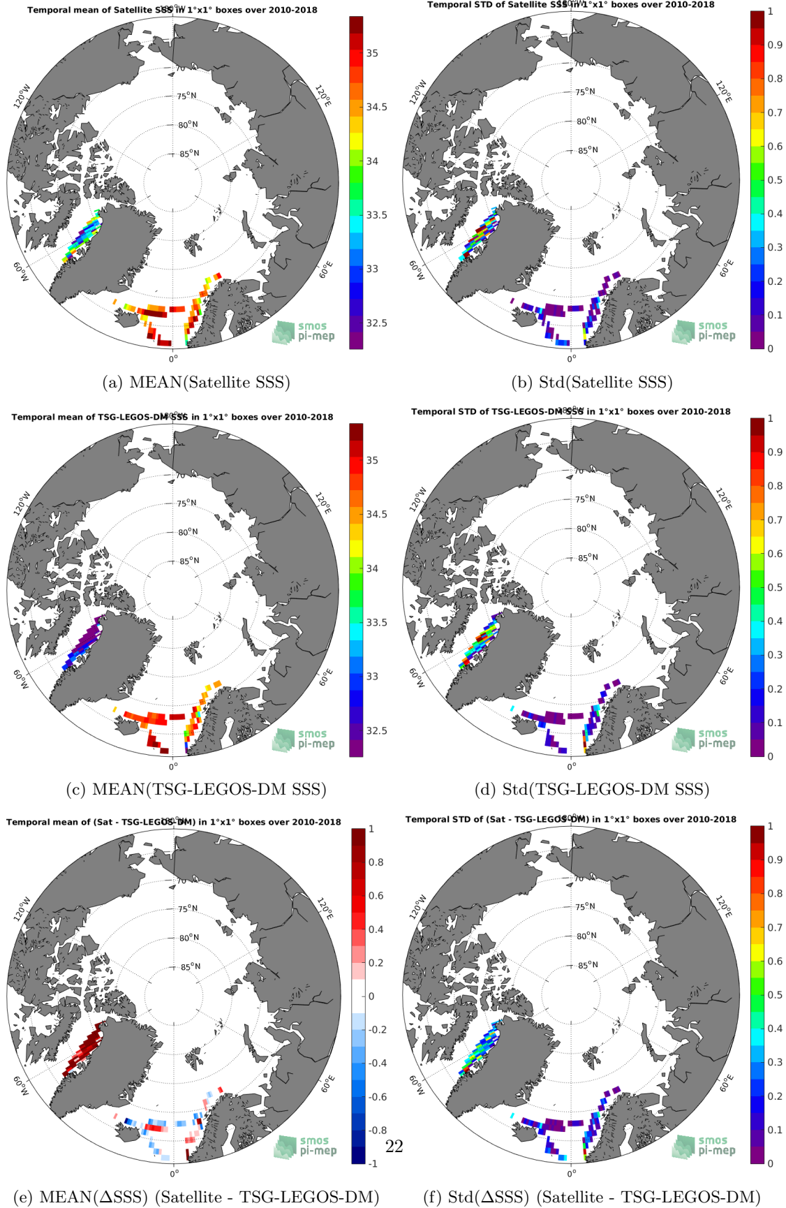
Figure 6: Temporal mean (left) and Std (right) of SSS from CCI L4 Merged-OI v1.8 - 30-day running (ESA) (top), TSG-LEGOS-DM (middle), and of \Delta SSS (Satellite - TSG-LEGOS-DM). Only match-up pairs are used to generate these maps.
