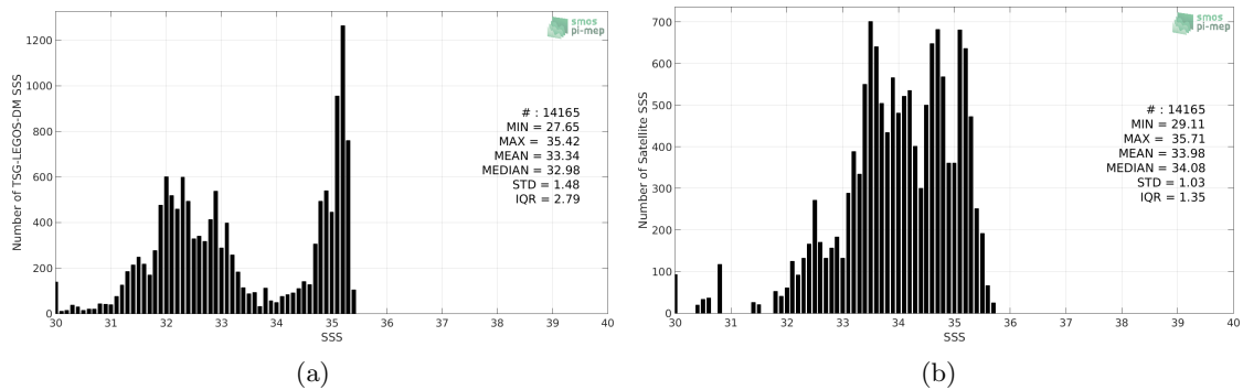
Figure 2: Histograms of SSS from TSG-LEGOS-DM (a) and CCI L4 Merged-OI v1.8 - 30-day running (ESA) (b) considering all match-up pairs per bins of 0.1 over the Arctic Ocean Pi-MEP region and for the full satellite product period.
