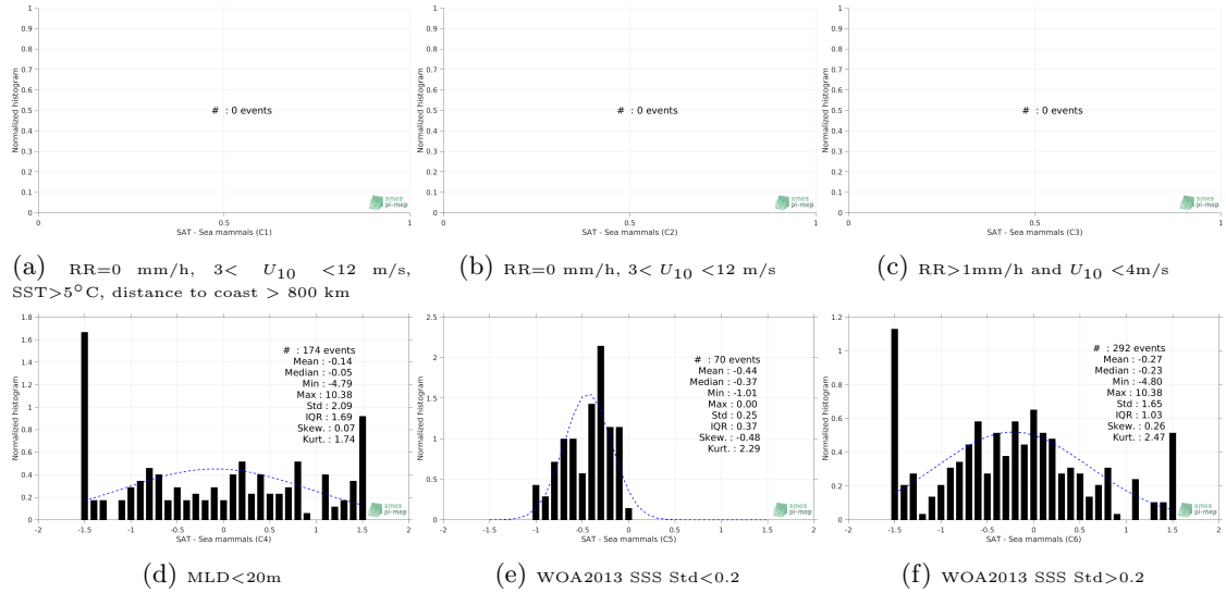
Figure 13: Normalized histogram of \Delta SSS (CCI L4 Merged-OI v1.8 - 30-day running (ESA) - Sea mammals) for 6 different subdatasets corresponding to: RR=0 mm/h, 3 < U_{10} < 12 m/s, SST > 5°C, distance to coast > 800 km (a), RR=0 mm/h, 3 < U_{10} < 12 m/s (b), RR > 1mm/h and U_{10} < 4 m/s (c), MLD < 20m (d), WOA2013 SSS Std < 0.2 (e), WOA2013 SSS Std > 0.2 (f).
