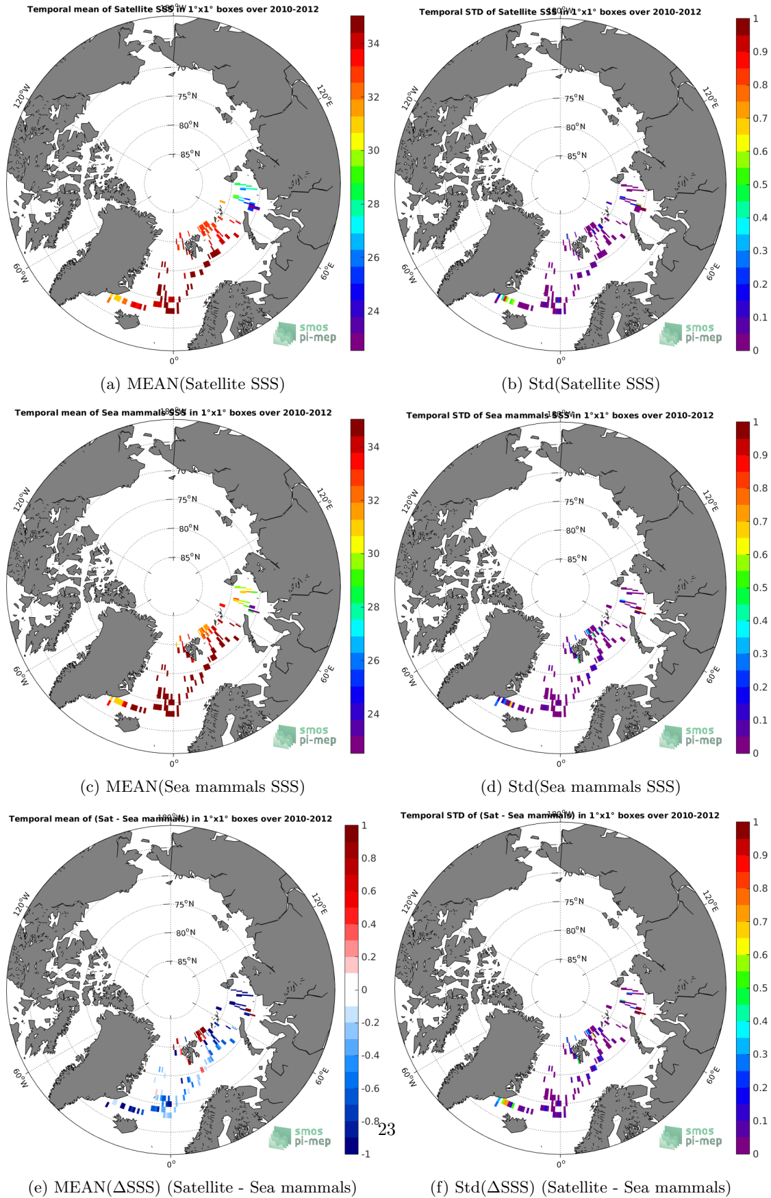
Figure 6: Temporal mean (left) and Std (right) of SSS from CCI L4 Merged-OI v1.8 - 30-day running (ESA) (top), Sea mammals (middle), and of \Delta SSS (Satellite - Sea mammals). Only match-up pairs are used to generate these maps.
