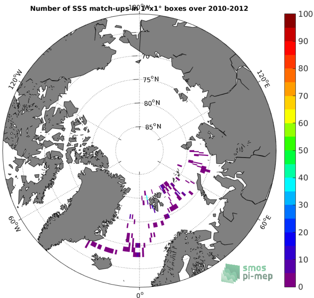
Figure 4: Number of SSS match-ups between Sea mammals SSS and the CCI L4 Merged-OI v1.8 - 30-day running (ESA) SSS product for the Arctic Ocean Pi-MEP region over 1^\circ \times 1^\circ boxes and for the full satellite product period.
