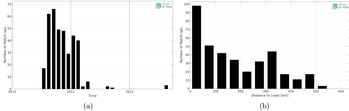
Figure 1: Number of match-ups between Sea mammals and CCI L4 Merged-OI v1.8 - 30-day running (ESA) SSS as a function of time (a) and as function of the distance to coast (b) over the Arctic Ocean Pi-MEP region and for the full satellite product period.
