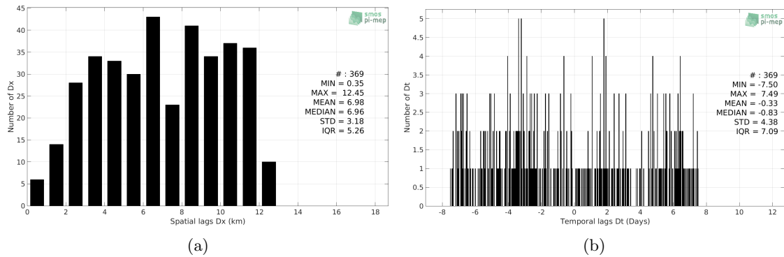
Figure 5: Histograms of the spatial (a) and temporal (b) lags between the time of the Sea mammals measurements and the date of the corresponding CCI L4 Merged-OI v1.8 - 30-day running (ESA) SSS product.
