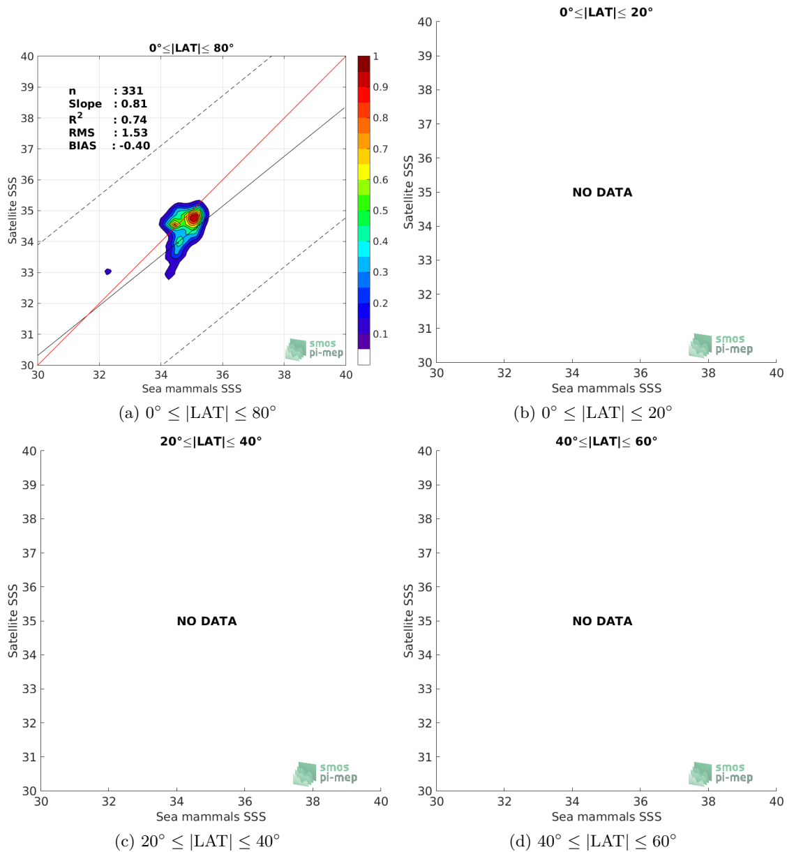
Figure 9: Contour maps of the concentration of CCI L4 Merged-OI v1.8 - 30-day running (ESA) SSS (y-axis) versus Sea mammals SSS (x-axis) at match-up pairs for different latitude bands. For each plot, the red line shows x=y . The black thin and dashed lines indicate a linear fit through the data cloud and the \pm 95\% confidence levels, respectively. The number match-up pairs n , the slope and R^2 coefficient of the linear fit, the root mean square (RMS) and the mean bias between satellite and in situ data are indicated for each latitude band in each plots.
