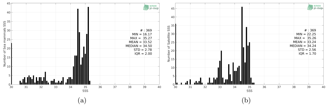
Figure 2: Histograms of SSS from Sea mammals (a) and CCI L4 Merged-OI v1.8 - 30-day running (ESA) (b) considering all match-up pairs per bins of 0.1 over the Arctic Ocean Pi-MEP region and for the full satellite product period.
