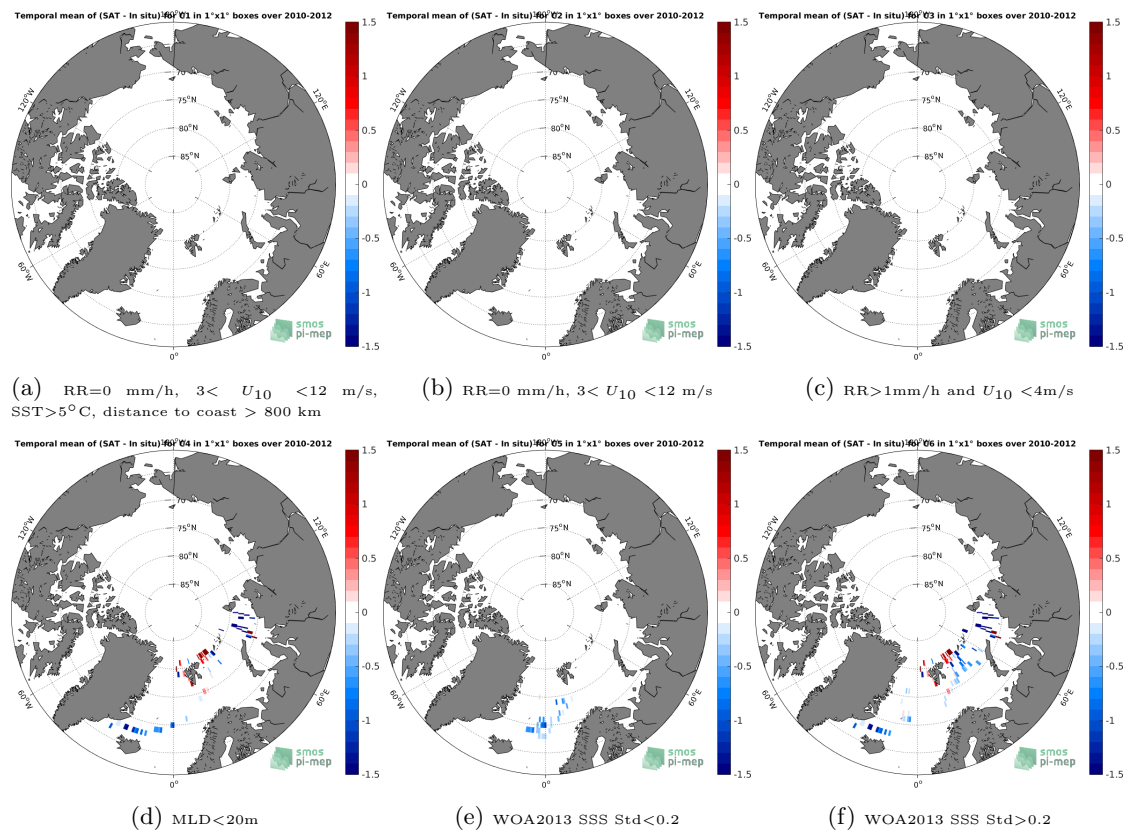
Figure 12: Temporal mean gridded over spatial boxes of size 1^{\circ}\times 1^{\circ} of \Delta\text{SSS} (CCI L4 Merged-OI v1.8 - 30-day running (ESA) - Sea mammals) for 6 different subdatasets corresponding to: RR=0 mm/h, 3 < U_{10} < 12 m/s, SST > 5^{\circ}\text{C} , distance to coast > 800 km (a), RR=0 mm/h, 3 < U_{10} < 12 m/s (b), RR > 1 mm/h and U_{10} < 4 m/s (c), MLD < 20 m (d), WOA2013 SSS Std < 0.2 (e), WOA2013 SSS Std > 0.2 (f).
