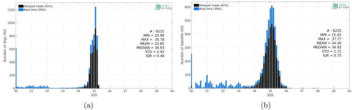
Figure 2: Histograms of SSS from Argo (a) and CCI L4 Merged-OI v1.8 - 30-day running (ESA) (b) considering all match-up pairs per bins of 0.1 over the Arctic Ocean Pi-MEP region and for the full satellite product period.
