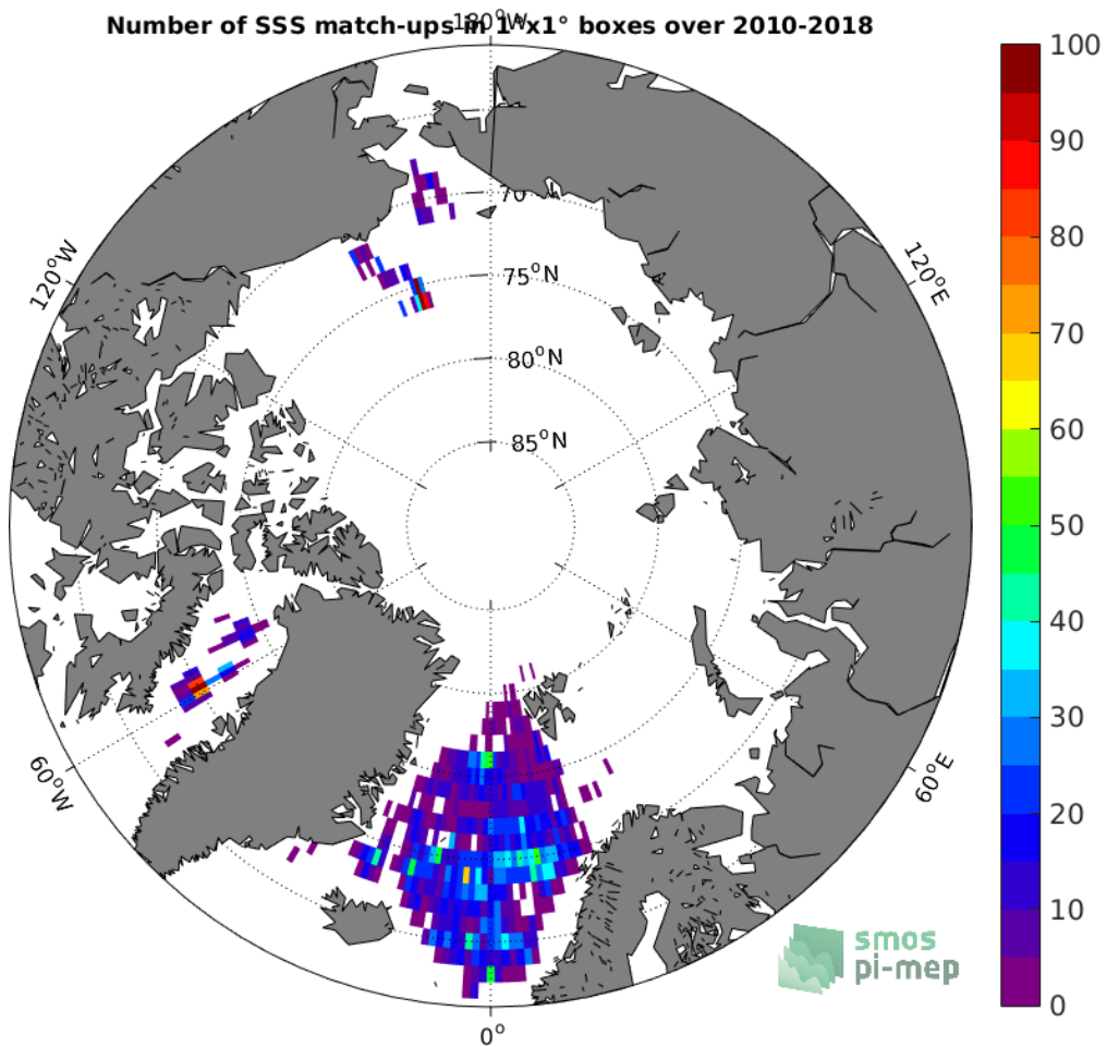
Figure 4: Number of SSS match-ups between Argo SSS and the CCI L4 Merged-OI v1.8 - 30-day running (ESA) SSS product for the Arctic Ocean Pi-MEP region over 1°x1° boxes and for the full satellite product period.
