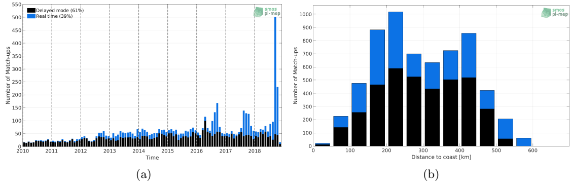
Figure 1: Number of match-ups between Argo and CCI L4 Merged-OI v1.8 - 30-day running (ESA) SSS as a function of time (a) and as function of the distance to coast (b) over the Arctic Ocean Pi-MEP region and for the full satellite product period.
