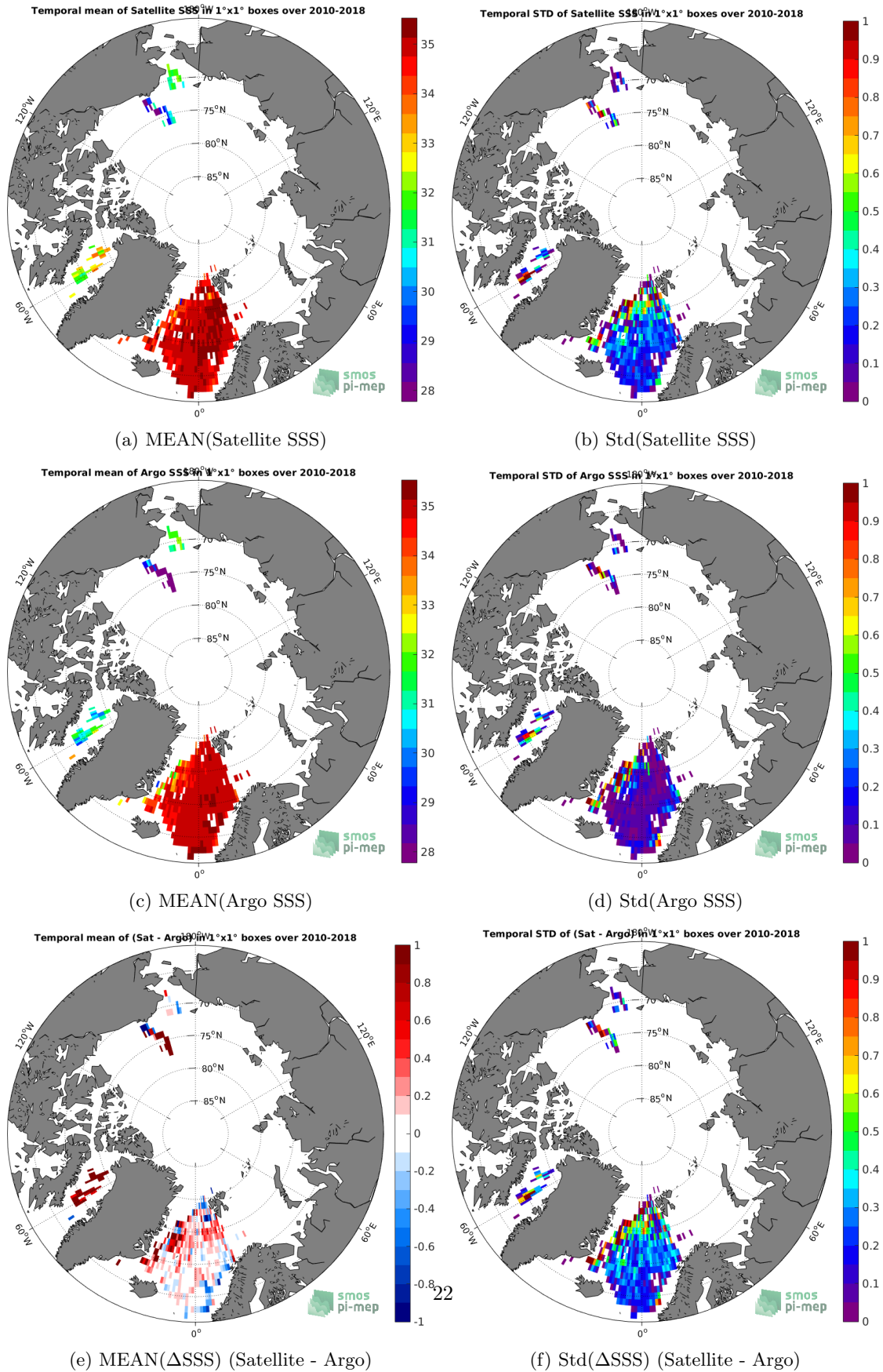
Figure 6: Temporal mean (left) and Std (right) of SSS from CCI L4 Merged-OI v1.8 - 30-day running (ESA) (top), Argo (middle), and of \Delta SSS (Satellite - Argo). Only match-up pairs are used to generate these maps.
