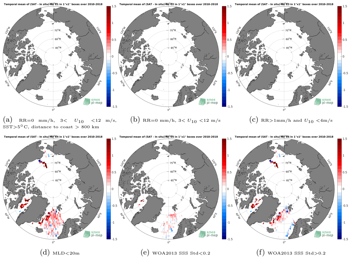
Figure 12: Temporal mean gridded over spatial boxes of size 1^{\circ}\times 1^{\circ} of \Delta\text{SSS} (CCI L4 Merged-OI v1.8 - 30-day running (ESA) - Argo) for 6 different subdatasets corresponding to:RR=0 mm/h, 3 < U_{10} < 12 m/s, SST >5^{\circ}\text{C} , distance to coast > 800 km (a), RR=0 mm/h, 3 < U_{10} < 12 m/s (b), RR >1 mm/h and U_{10} < 4 m/s (c),MLD <20 m (d),WOA2013 SSS Std <0.2 (e),WOA2013 SSS Std >0.2 (f).
