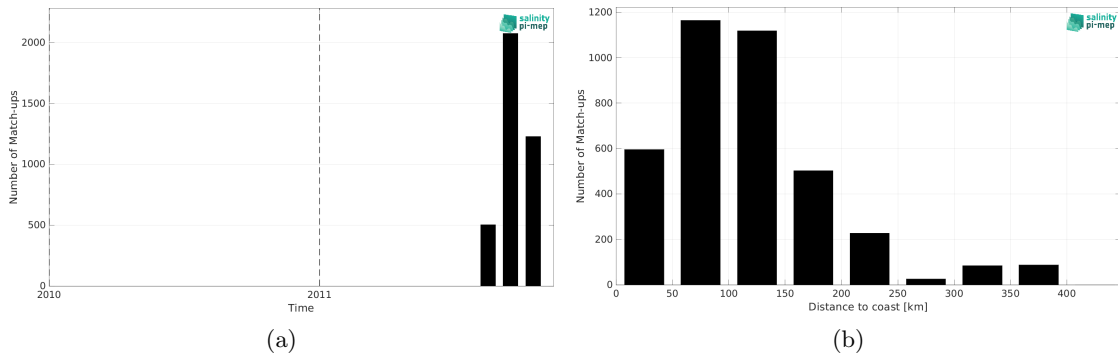
Figure 2: Number of match-ups between TSG (SAMOS) and Aquarius SSS L4 OI v5 - Weekly (IPRC) SSS as a function of time (a) and as function of the distance to coast (b) over the Arctic Ocean Pi-MEP region and for the full satellite product period.
