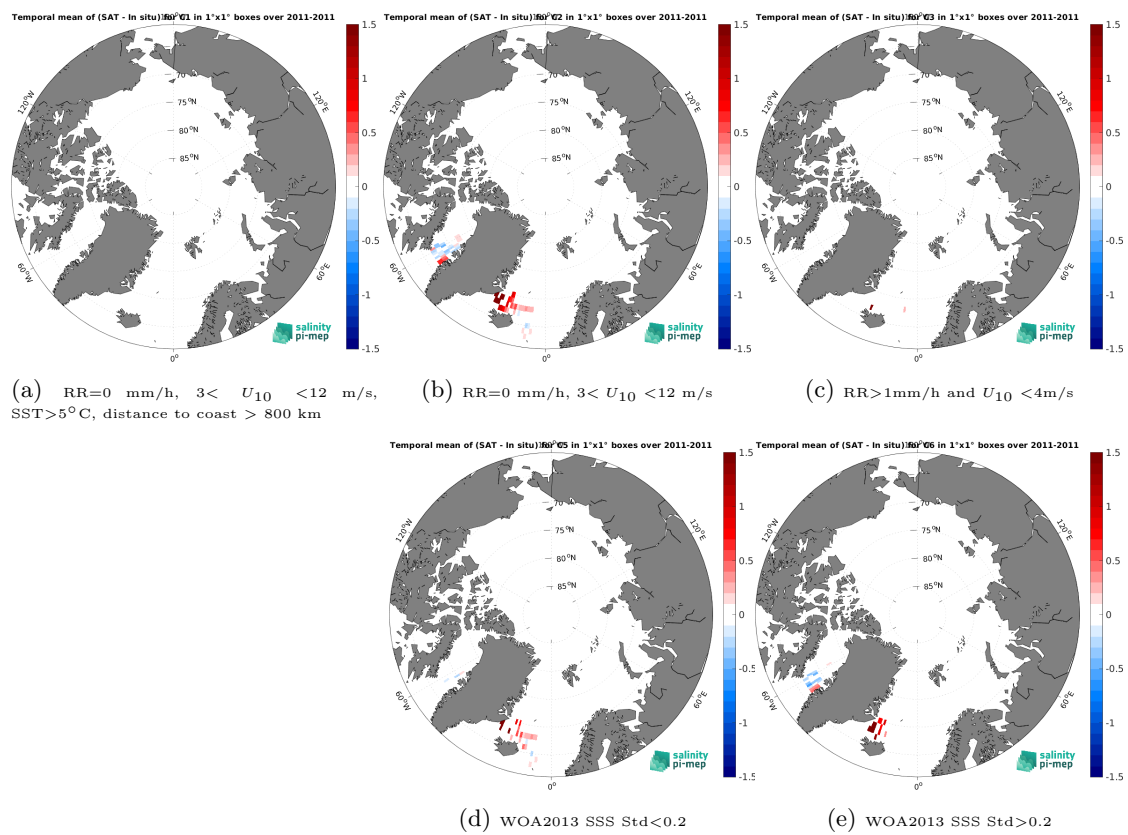
Figure 14: Temporal mean gridded over spatial boxes of size 1^\circ \times 1^\circ of \Delta\text{SSS} (Aquarius SSS L4 OI v5 - Weekly (IPRC) - TSG (SAMOS)) for 5 different subdatasets corresponding to:RR=0 mm/h, 3 < U_{10} < 12 m/s, SST > 5°C, distance to coast > 800 km (a), RR=0 mm/h, 3 < U_{10} < 12 m/s (b), RR > 1mm/h and U_{10} < 4 m/s (c), WOA2013 SSS Std < 0.2 (d), WOA2013 SSS Std > 0.2 (e).
