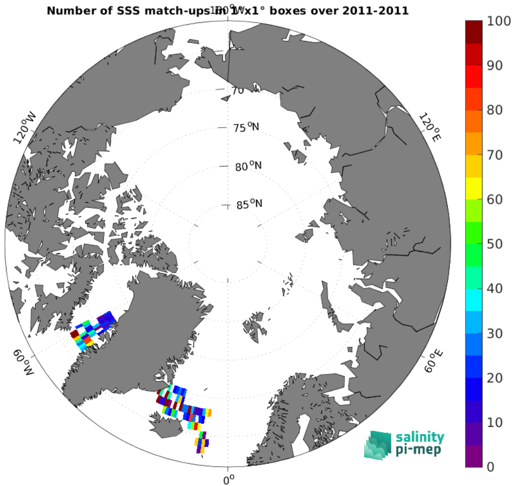
Figure 5: Number of SSS match-ups between TSG (SAMOS) SSS and the Aquarius SSS L4 OI v5 - Weekly (IPRC) SSS product for the Arctic Ocean Pi-MEP region over 1^\circ \times 1^\circ boxes and for the full satellite product period.
