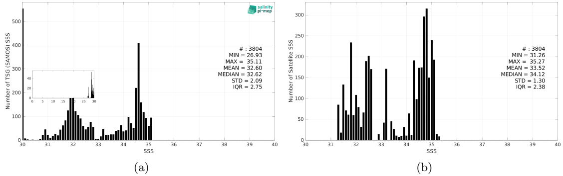
Figure 3: Histograms of SSS from TSG (SAMOS) (a) and Aquarius SSS L4 OI v5 - Weekly (IPRC) (b) considering all match-up pairs per bins of 0.1 over the Arctic Ocean Pi-MEP region and for the full satellite product period.
