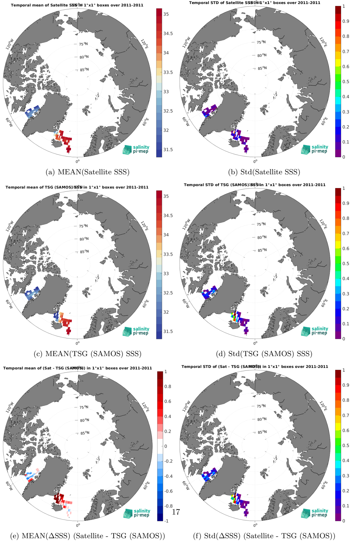
Figure 7: Temporal mean (left) and Std (right) of SSS from Aquarius SSS L4 OI v5 - Weekly (IPRC) (top), TSG (SAMOS) (middle), and of \Delta SSS (Satellite - TSG (SAMOS)). Only match-up pairs are used to generate these maps.
