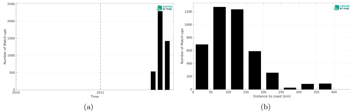
Figure 1: Number of match-ups between TSG (SAMOS) and Aquarius SSS L4 OI v5 - Weekly (IPRC) SSS as a function of time (a) and as function of the distance to coast (b) over the Arctic Ocean Pi-MEP region and for the full satellite product period.
