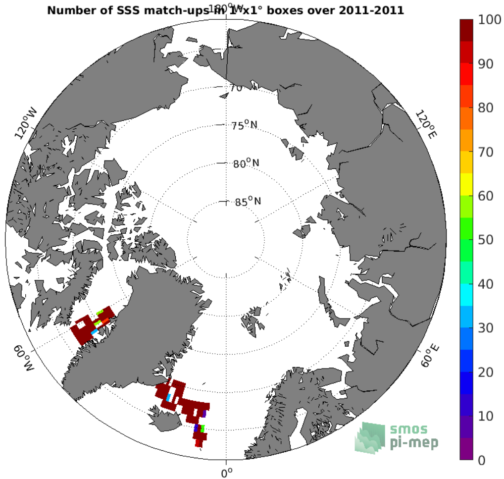
Figure 4: Number of SSS match-ups between TSG (SAMOS) SSS and the Aquarius SSS L4 OI v5 - Weekly (IPRC) SSS product for the Arctic Ocean Pi-MEP region over 1^\circ \times 1^\circ boxes and for the full satellite product period.
