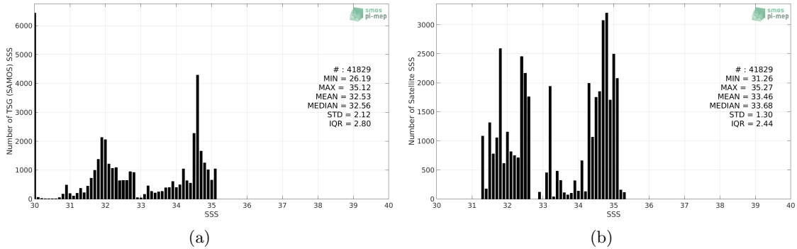
Figure 2: Histograms of SSS from TSG (SAMOS) (a) and Aquarius SSS L4 OI v5 - Weekly (IPRC) (b) considering all match-up pairs per bins of 0.1 over the Arctic Ocean Pi-MEP region and for the full satellite product period.
