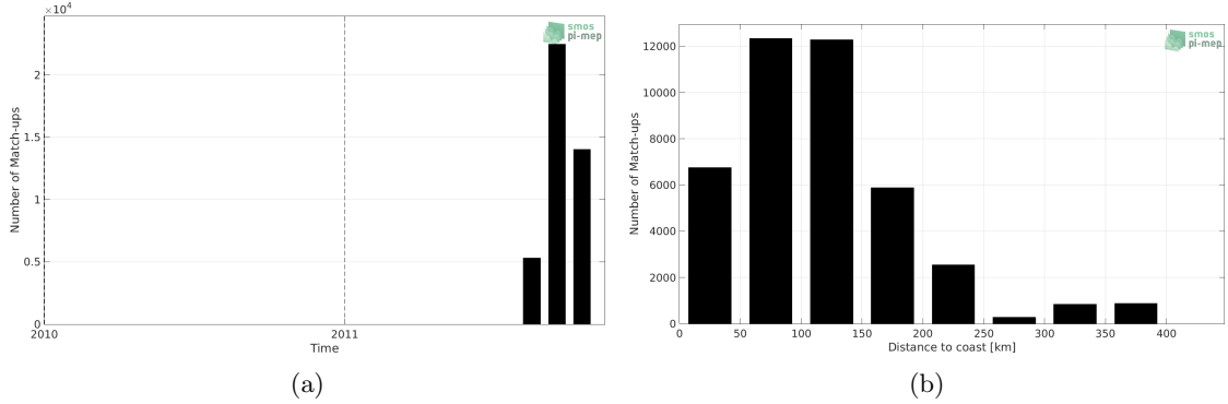
Figure 1: Number of match-ups between TSG (SAMOS) and Aquarius SSS L4 OI v5 - Weekly (IPRC) SSS as a function of time (a) and as function of the distance to coast (b) over the Arctic Ocean Pi-MEP region and for the full satellite product period.
