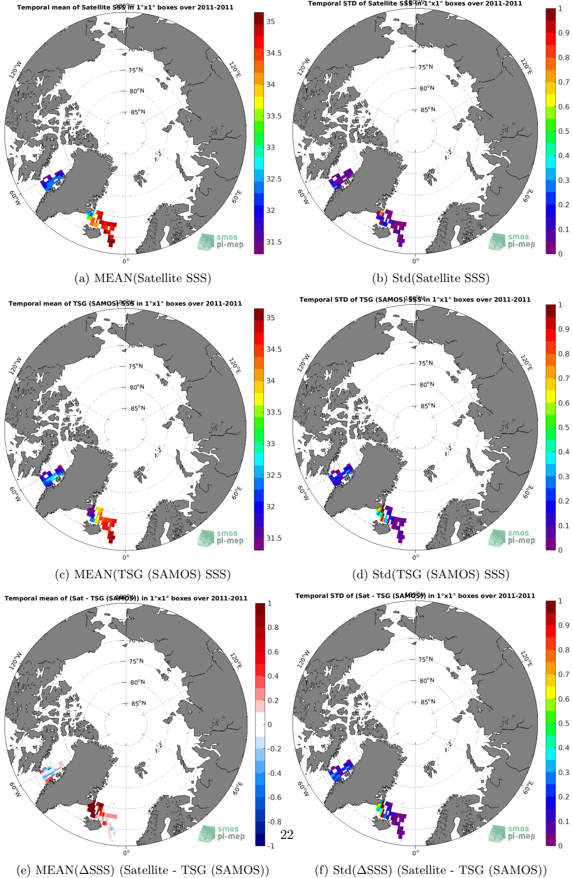
Figure 6: Temporal mean (left) and Std (right) of SSS from Aquarius SSS L4 OI v5 - Weekly (IPRC) (top), TSG (SAMOS) (middle), and of \Delta SSS (Satellite - TSG (SAMOS)). Only match-up pairs are used to generate these maps.
