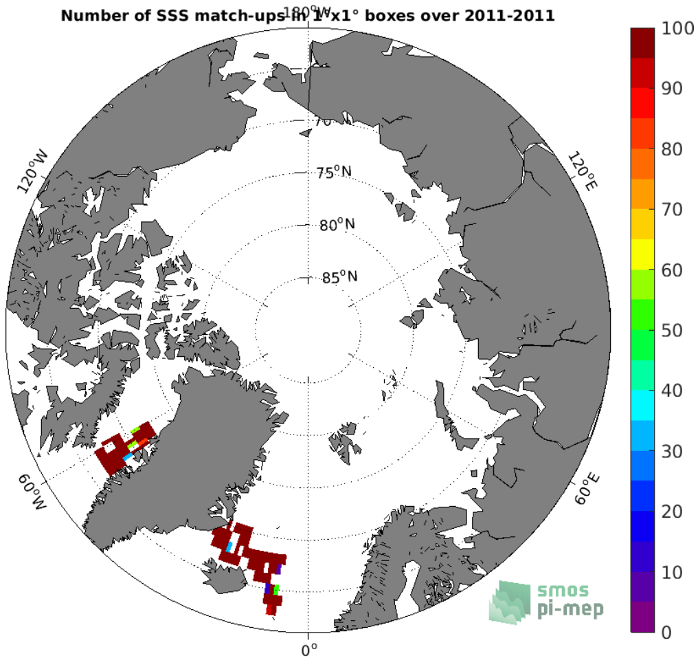
Figure 4: Number of SSS match-ups between TSG (SAMOS) SSS and the Aquarius SSS L4 OI v5 - Weekly (IPRC) SSS product for the Arctic Ocean Pi-MEP region over 1°x1° boxes and for the full satellite product period.
