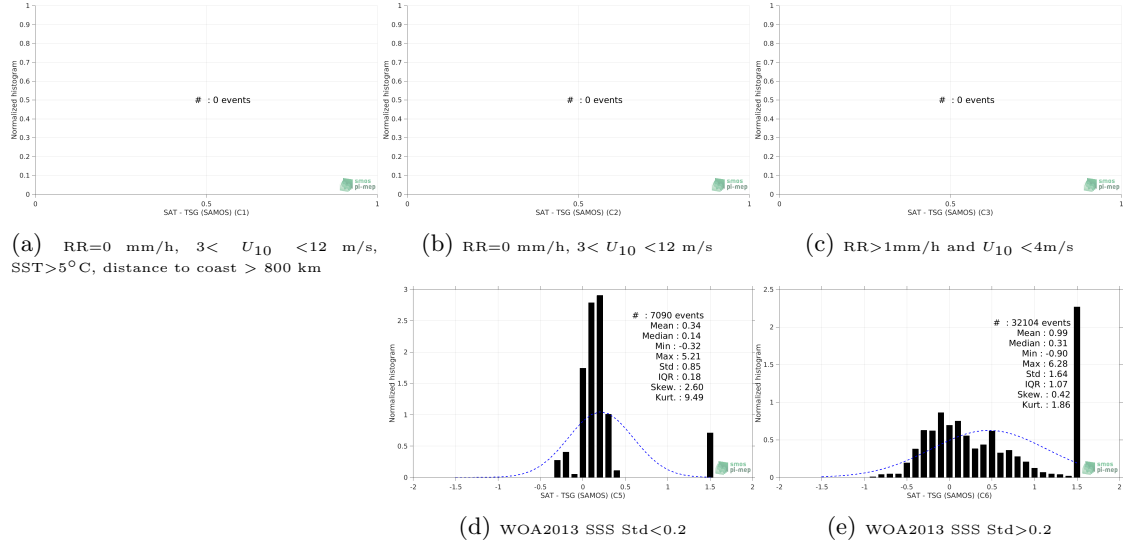
Figure 13: Normalized histogram of \Delta\text{SSS} (Aquarius SSS L4 OI v5 - Weekly (IPRC) - TSG (SAMOS)) for 5 different subdatasets corresponding to: RR=0 mm/h, 3 < U_{10} < 12 m/s, SST > 5^\circ\text{C} , distance to coast > 800 km (a), RR=0 mm/h, 3 < U_{10} < 12 m/s (b), RR > 1 mm/h and U_{10} < 4 m/s (c), WOA2013 SSS Std < 0.2 (d), WOA2013 SSS Std > 0.2 (e).
