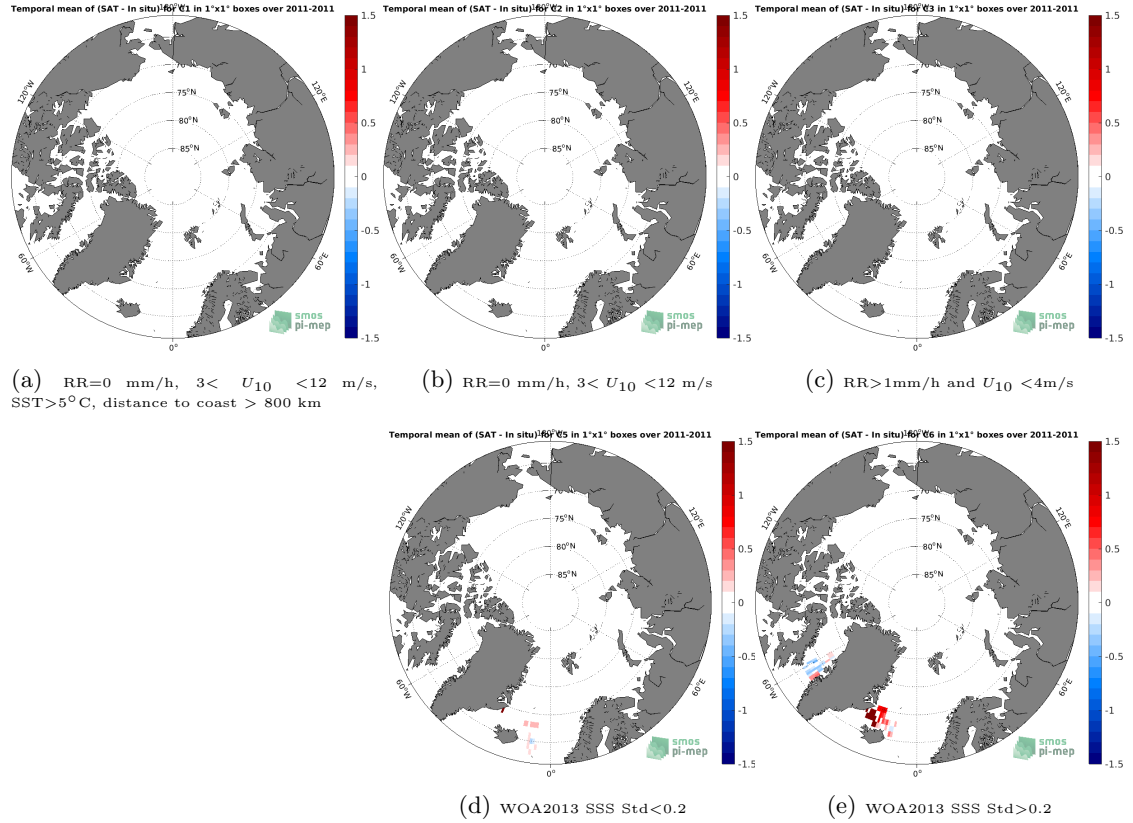
Figure 12: Temporal mean gridded over spatial boxes of size 1^{\circ}\times 1^{\circ} of \Delta\text{SSS} (Aquarius SSS L4 OI v5 - Weekly (IPRC) - TSG (SAMOS)) for 5 different subdatasets corresponding to: RR=0 mm/h, 3 < U_{10} < 12 m/s, SST >5^{\circ}\text{C} , distance to coast > 800 km (a), RR=0 mm/h, 3 < U_{10} < 12 m/s (b), RR >1 mm/h and U_{10} < 4 m/s (c), WOA2013 SSS Std <0.2 (d), WOA2013 SSS Std >0.2 (e).
