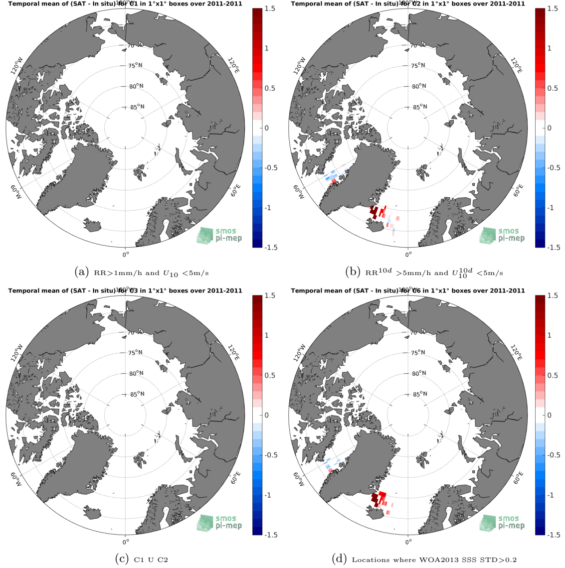
Figure 12: Temporal mean gridded over spatial boxes of size 1^\circ \times 1^\circ of \Delta SSS (Aquarius-L4-IPRC-V5-WEEKLY - TSG-SAMOS) for 4 different subdatasets corresponding to: RR > 1mm/h and U_{10} < 5\text{m/s} (a), RR 10d > 5mm/h and U_{10}^{10d} < 5\text{m/s} (b), C1 U C2 (c), Locations where WOA2013 SSS STD > 0.2 (d).
