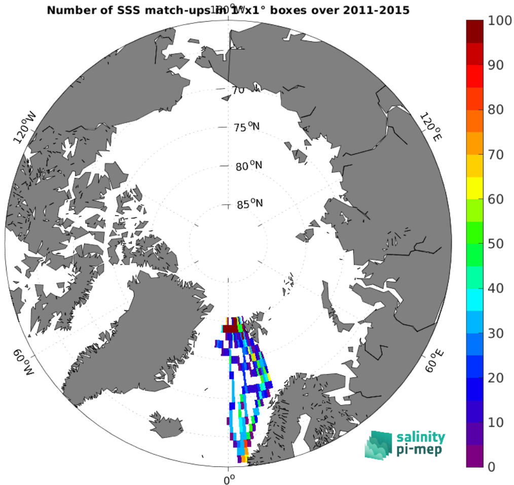
Figure 4: Number of SSS match-ups between TSG (Polarstern) SSS and the Aquarius SSS L4 OI v5 - Weekly (IPRC) SSS product for the Arctic Ocean Pi-MEP region over 1^\circ \times 1^\circ boxes and for the full satellite product period.
