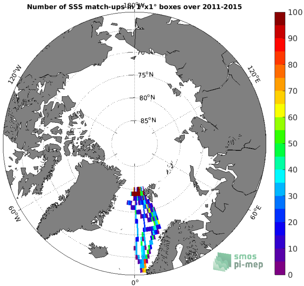
Figure 4: Number of SSS match-ups between TSG (Polarstern) SSS and the Aquarius SSS L4 OI v5 - Weekly (IPRC) SSS product for the Arctic Ocean Pi-MEP region over 1°x1° boxes and for the full satellite product period.
