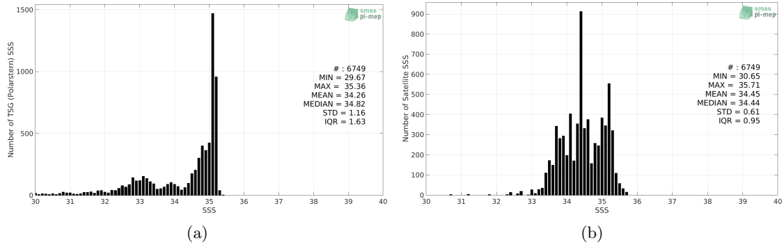
Figure 2: Histograms of SSS from TSG (Polarstern) (a) and Aquarius SSS L4 OI v5 - Weekly (IPRC) (b) considering all match-up pairs per bins of 0.1 over the Arctic Ocean Pi-MEP region and for the full satellite product period.
