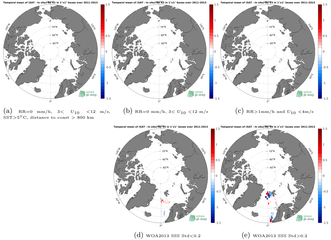
Figure 12: Temporal mean gridded over spatial boxes of size 1^{\circ}\times 1^{\circ} of \Delta\text{SSS} (Aquarius SSS L4 OI v5 - Weekly (IPRC) - TSG (Polarstern)) for 5 different subdatasets corresponding to: \text{RR}=0 mm/h, 3 < U_{10} < 12 m/s, \text{SST} > 5^{\circ}\text{C} , distance to coast > 800 km (a), \text{RR}=0 mm/h, 3 < U_{10} < 12 m/s (b), \text{RR} > 1 mm/h and U_{10} < 4 m/s (c), WOA2013 SSS Std < 0.2 (d), WOA2013 SSS Std > 0.2 (e).
