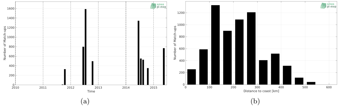
Figure 1: Number of match-ups between TSG (Polarstern) and Aquarius SSS L4 OI v5 - Weekly (IPRC) SSS as a function of time (a) and as function of the distance to coast (b) over the Arctic Ocean Pi-MEP region and for the full satellite product period.
