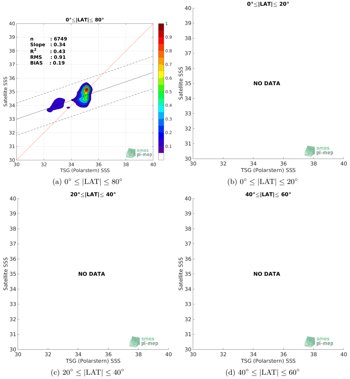
Figure 9: Contour maps of the concentration of Aquarius SSS L4 OI v5 - Weekly (IPRC) SSS (y-axis) versus TSG (Polarstern) SSS (x-axis) at match-up pairs for different latitude bands. For each plot, the red line shows x=y . The black thin and dashed lines indicate a linear fit through the data cloud and the \pm 95\% confidence levels, respectively. The number match-up pairs n , the slope and R^2 coefficient of the linear fit, the root mean square (RMS) and the mean bias between satellite and in situ data are indicated for each latitude band in each plots.
