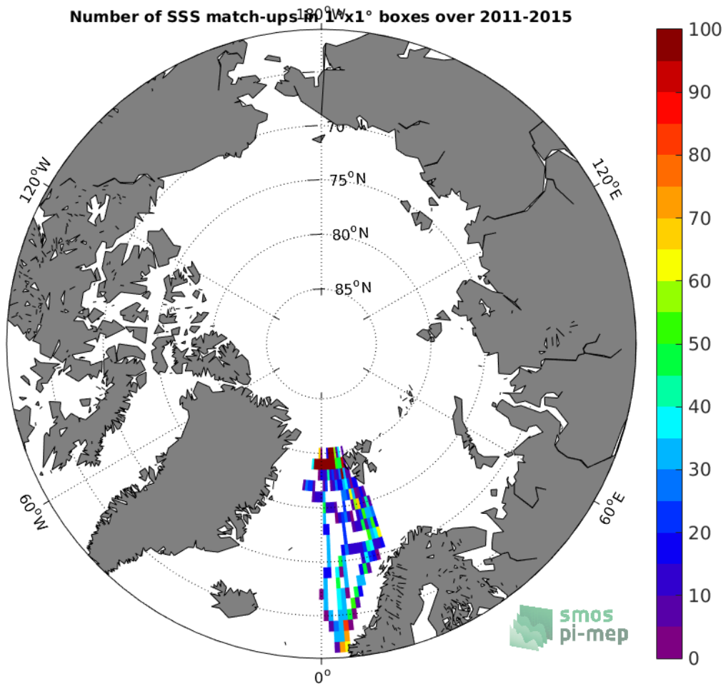
Figure 4: Number of SSS match-ups between TSG-POLARSTERN SSS and the Aquarius-L4-IPRC-V5-WEEKLY SSS product for the Arctic Ocean Pi-MEP region over 1^\circ \times 1^\circ boxes and for the full satellite product period.
