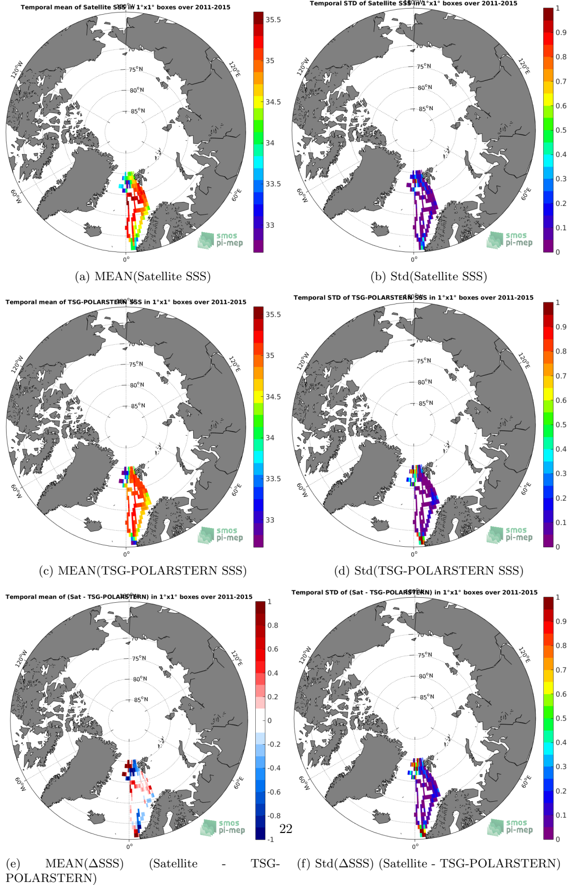
Figure 6: Temporal mean (left) and Std (right) of SSS from Aquarius-L4-IPRC-V5-WEEKLY (top), TSG-POLARSTERN (middle), and of \Delta SSS (Satellite - TSG-POLARSTERN). Only match-up pairs are used to generate these maps.
