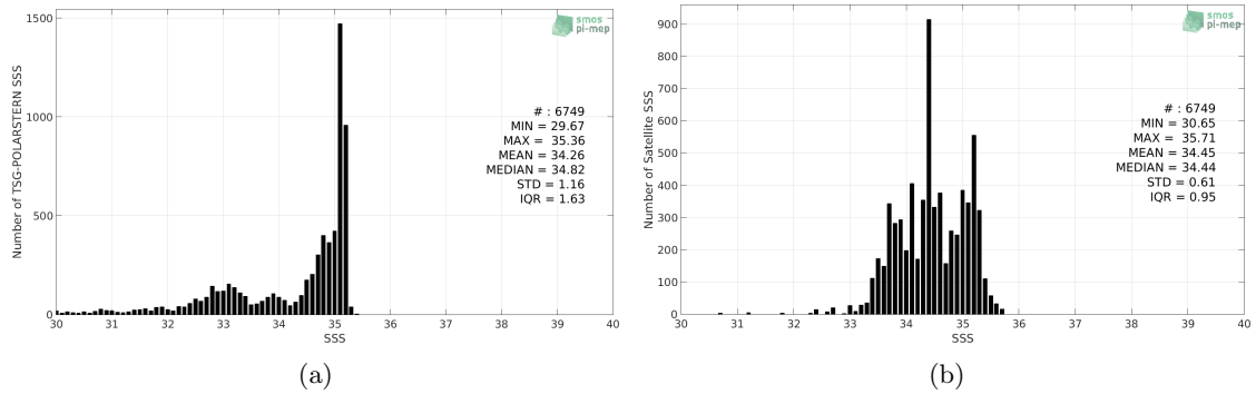
Figure 2: Histograms of SSS from TSG-POLARSTERN (a) and Aquarius-L4-IPRC-V5-WEEKLY (b) considering all match-up pairs per bins of 0.1 over the Arctic Ocean Pi-MEP region and for the full satellite product period.
