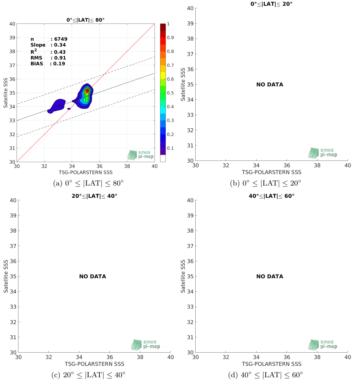
Figure 9: Contour maps of the concentration of Aquarius-L4-IPRC-V5-WEEKLY SSS (y-axis) versus TSG-POLARSTERN SSS (x-axis) at match-up pairs for different latitude bands. For each plot, the red line shows x=y . The black thin and dashed lines indicate a linear fit through the data cloud and the \pm 95\% confidence levels, respectively. The number match-up pairs n , the slope and R^2 coefficient of the linear fit, the root mean square (RMS) and the mean bias between satellite and in situ data are indicated for each latitude band in each plots.
