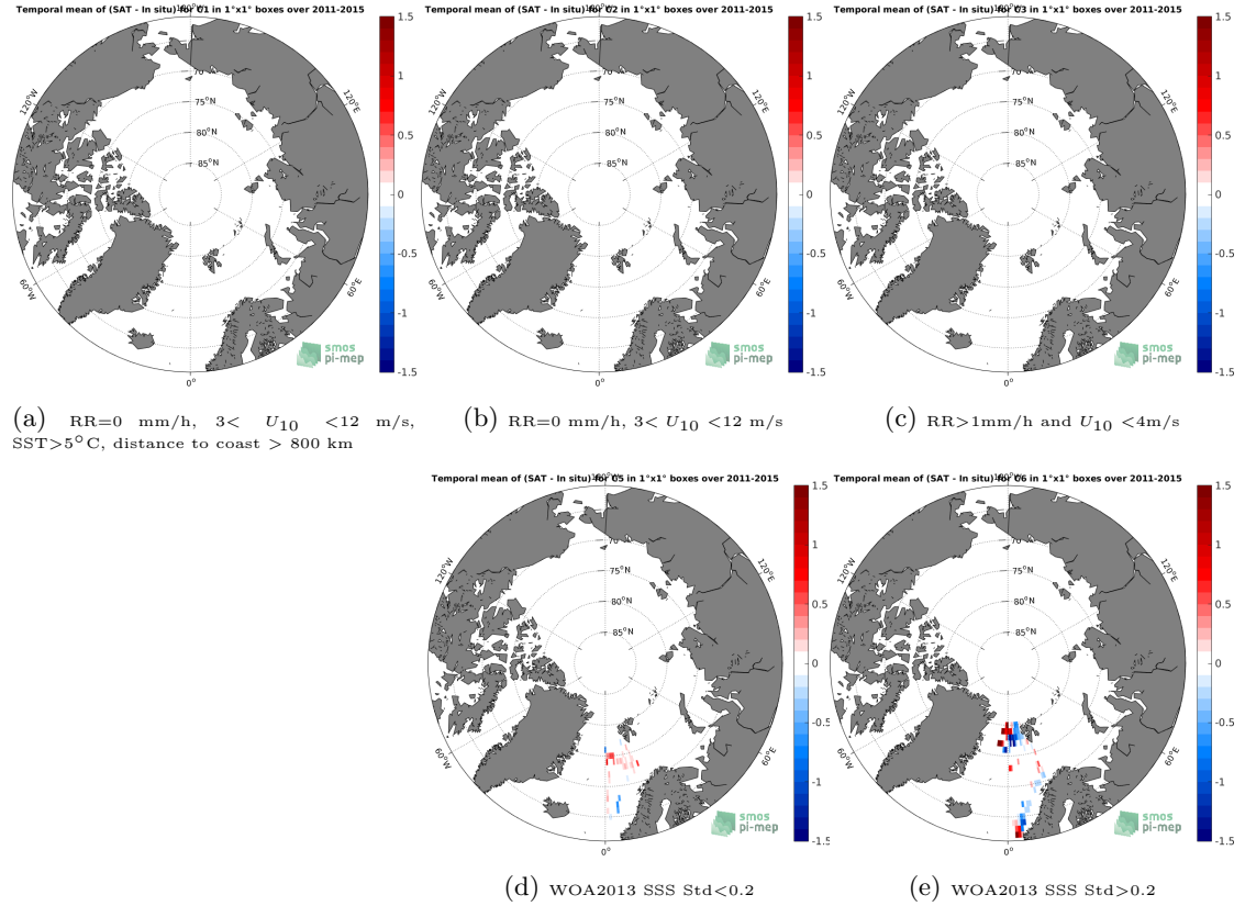
Figure 12: Temporal mean gridded over spatial boxes of size 1^{\circ}\times 1^{\circ} of \Delta\text{SSS} (Aquarius-L4-IPRC-V5-WEEKLY - TSG-POLARSTERN) for 5 different subdatasets corresponding to: RR=0 mm/h, 3 < U_{10} < 12 m/s, SST >5^{\circ}\text{C} , distance to coast > 800 km (a), RR=0 mm/h, 3 < U_{10} < 12 m/s (b), RR >1 mm/h and U_{10} < 4 m/s (c), WOA2013 SSS Std <0.2 (d), WOA2013 SSS Std >0.2 (e).
