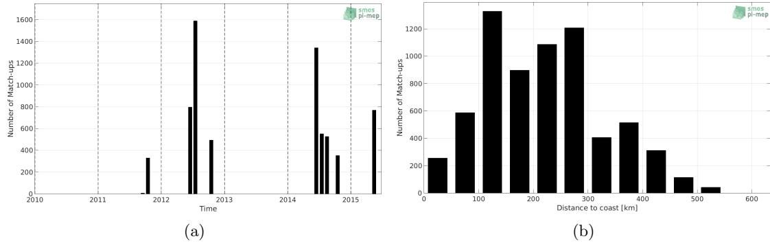
Figure 1: Number of match-ups between TSG-POLARSTERN and Aquarius-L4-IPRC-V5-WEEKLY SSS as a function of time (a) and as function of the distance to coast (b) over the Arctic Ocean Pi-MEP region and for the full satellite product period.
