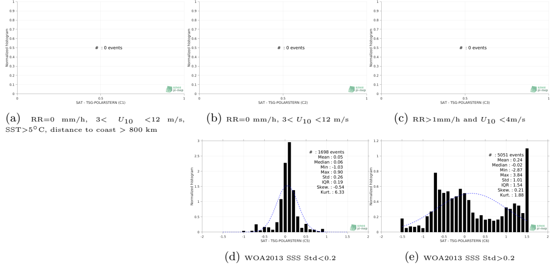
Figure 13: Normalized histogram of \Delta\text{SSS} (Aquarius-L4-IPRC-V5-WEEKLY - TSG-POLARSTERN) for 5 different subdatasets corresponding to: RR=0 mm/h, 3 < U_{10} < 12 m/s, SST >5^{\circ}\text{C} , distance to coast > 800 km (a), RR=0 mm/h, 3 < U_{10} < 12 m/s (b), RR>1\text{mm/h} and U_{10} < 4\text{m/s} (c), WOA2013 SSS Std <0.2 (d), WOA2013 SSS Std >0.2 (e).
