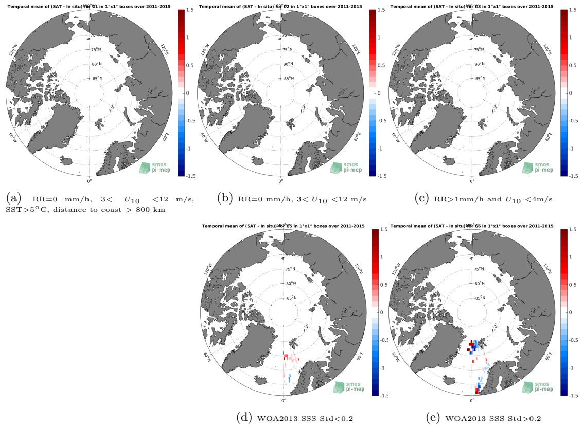
Figure 12: Temporal mean gridded over spatial boxes of size 1^\circ \times 1^\circ of \Delta SSS (Aquarius-L4-IPRC-V5-WEEKLY - TSG-POLARSTERN) for 5 different subdatasets corresponding to:RR=0 mm/h, 3 < U_{10} < 12 m/s, SST >5^\circ\text{C} , distance to coast > 800 km (a), RR=0 mm/h, 3 < U_{10} < 12 m/s (b), RR >1 mm/h and U_{10} < 4 m/s (c), WOA2013 SSS Std <0.2 (d), WOA2013 SSS Std >0.2 (e).
