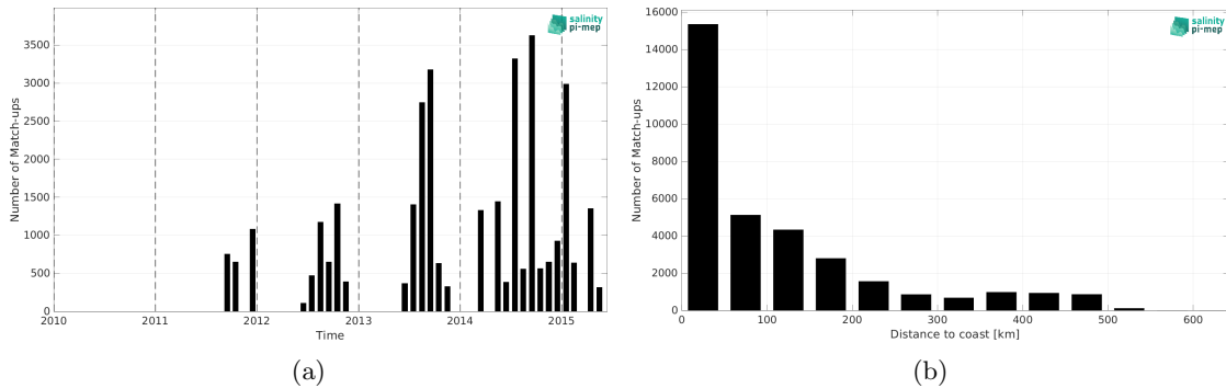
Figure 2: Number of match-ups between TSG (LEGOS-DM) and Aquarius SSS L4 OI v5 - Weekly (IPRC) SSS as a function of time (a) and as function of the distance to coast (b) over the Arctic Ocean Pi-MEP region and for the full satellite product period.
