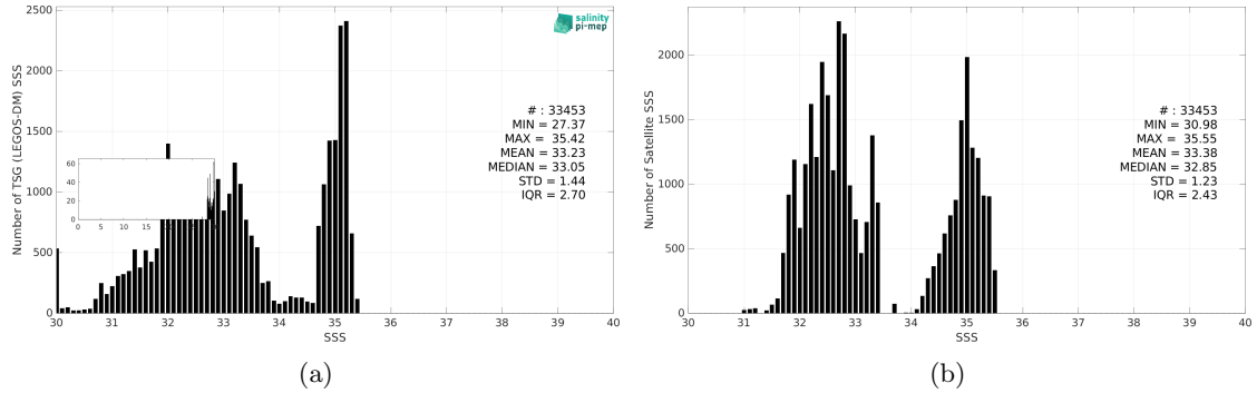
Figure 3: Histograms of SSS from TSG (LEGOS-DM) (a) and Aquarius SSS L4 OI v5 - Weekly (IPRC) (b) considering all match-up pairs per bins of 0.1 over the Arctic Ocean Pi-MEP region and for the full satellite product period.
