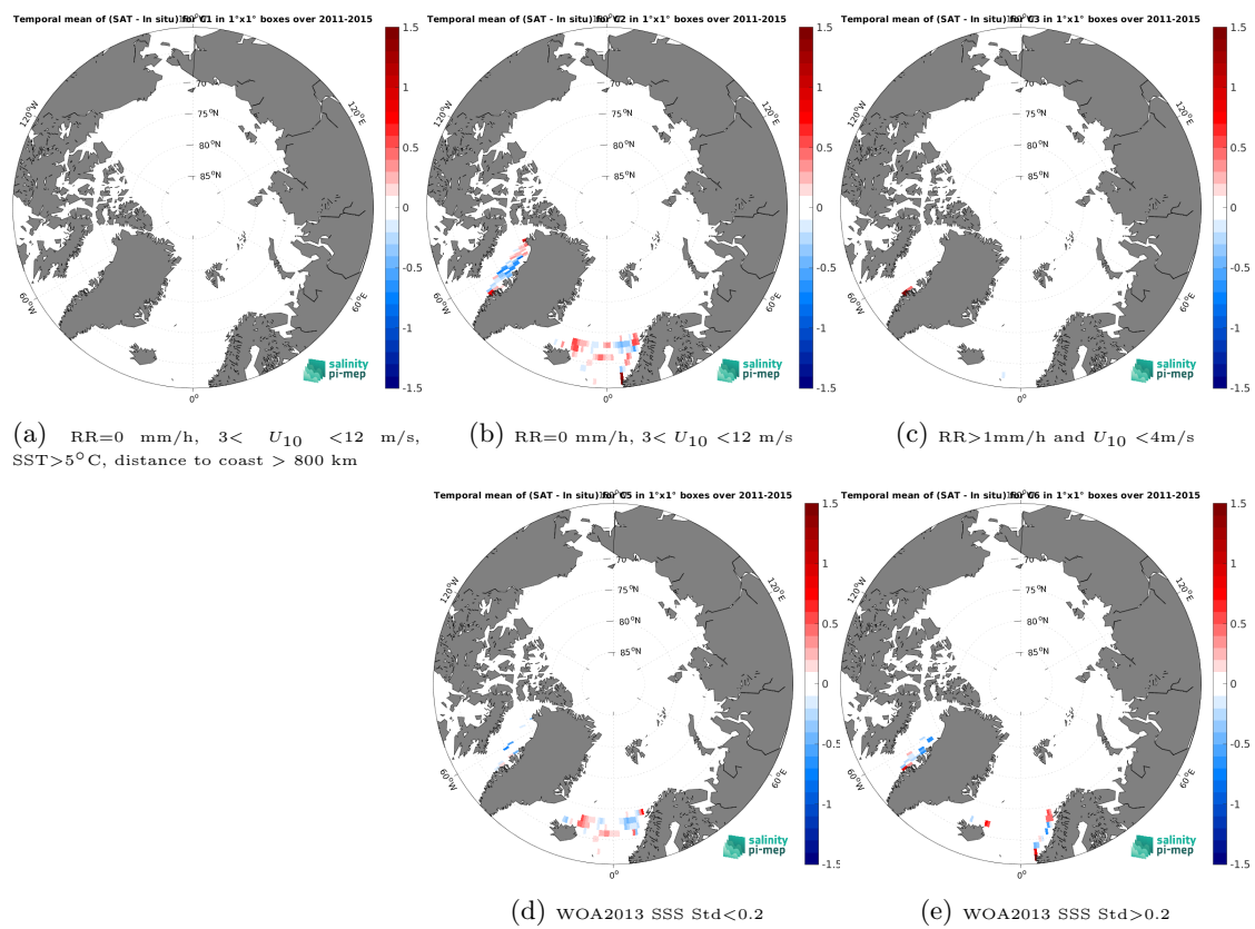
Figure 14: Temporal mean gridded over spatial boxes of size 1^\circ \times 1^\circ of \Delta SSS (Aquarius SSS L4 OI v5 - Weekly (IPRC) - TSG (LEGOS-DM)) for 5 different subdatasets corresponding to:RR=0 mm/h, 3 < U_{10} < 12 m/s, SST > 5°C, distance to coast > 800 km (a), RR=0 mm/h, 3 < U_{10} < 12 m/s (b), RR > 1mm/h and U_{10} < 4 m/s (c), WOA2013 SSS Std < 0.2 (d), WOA2013 SSS Std > 0.2 (e).
