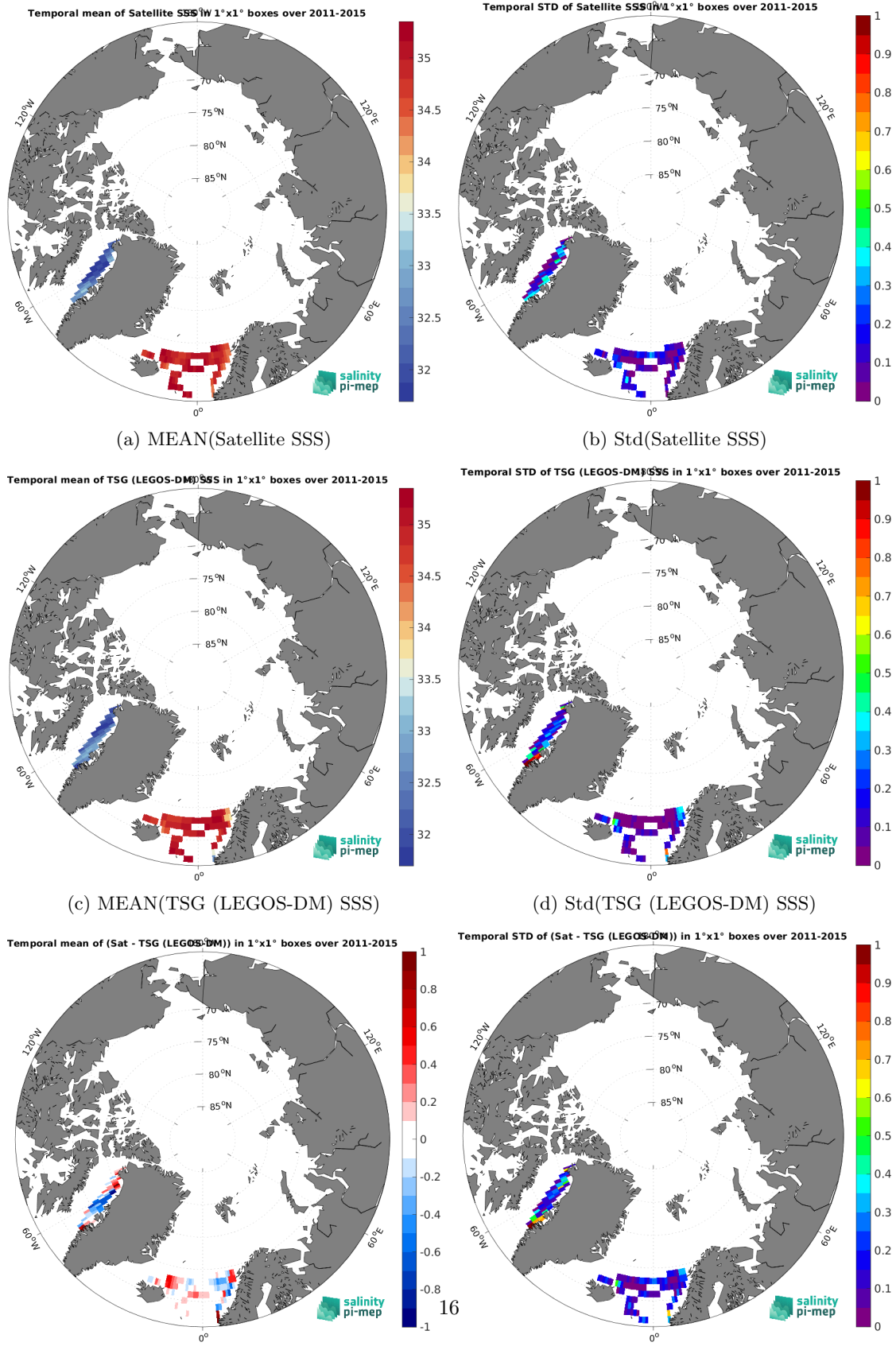
(e) MEAN( \Delta SSS) (Satellite - TSG (LEGOS-DM)) (f) Std( \Delta SSS) (Satellite - TSG (LEGOS-DM)) Figure 7: Temporal mean (left) and Std (right) of SSS from Aquarius SSS L4 OI v5 - Weekly (IPRC) (top), TSG (LEGOS-DM) (middle), and of \Delta SSS (Satellite - TSG (LEGOS-DM)). Only match-up pairs are used to generate these maps.
