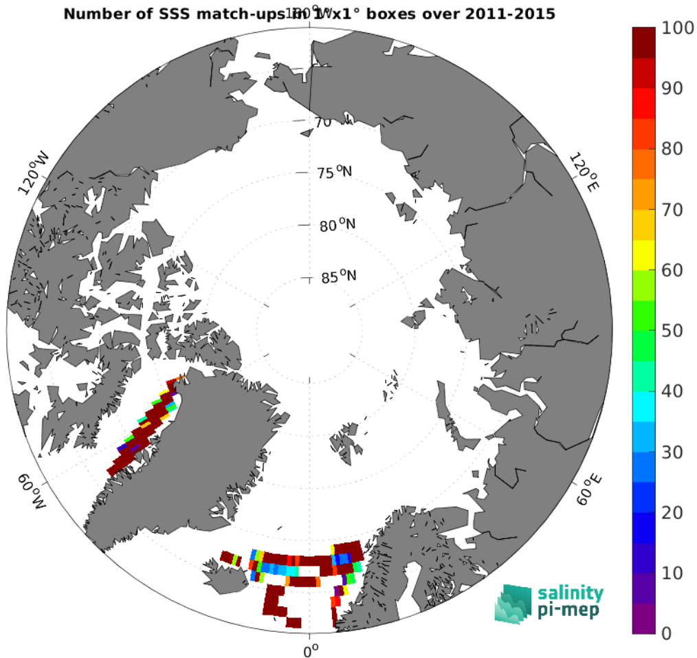
Figure 5: Number of SSS match-ups between TSG (LEGOS-DM) SSS and the Aquarius SSS L4 OI v5 - Weekly (IPRC) SSS product for the Arctic Ocean Pi-MEP region over 1^\circ \times 1^\circ boxes and for the full satellite product period.
