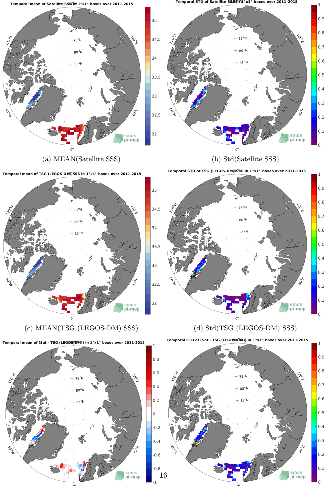
(e) MEAN( \Delta SSS) (Satellite - TSG (LEGOS-DM)) (f) Std( \Delta SSS) (Satellite - TSG (LEGOS-DM)) Figure 6: Temporal mean (left) and Std (right) of SSS from Aquarius SSS L4 OI v5 - Weekly (IPRC) (top), TSG (LEGOS-DM) (middle), and of \Delta SSS (Satellite - TSG (LEGOS-DM)). Only match-up pairs are used to generate these maps.
