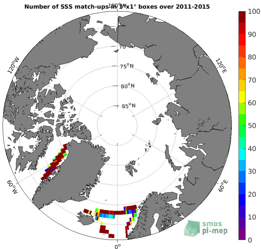
Figure 4: Number of SSS match-ups between TSG (LEGOS-DM) SSS and the Aquarius SSS L4 OI v5 - Weekly (IPRC) SSS product for the Arctic Ocean Pi-MEP region over 1^\circ \times 1^\circ boxes and for the full satellite product period.
