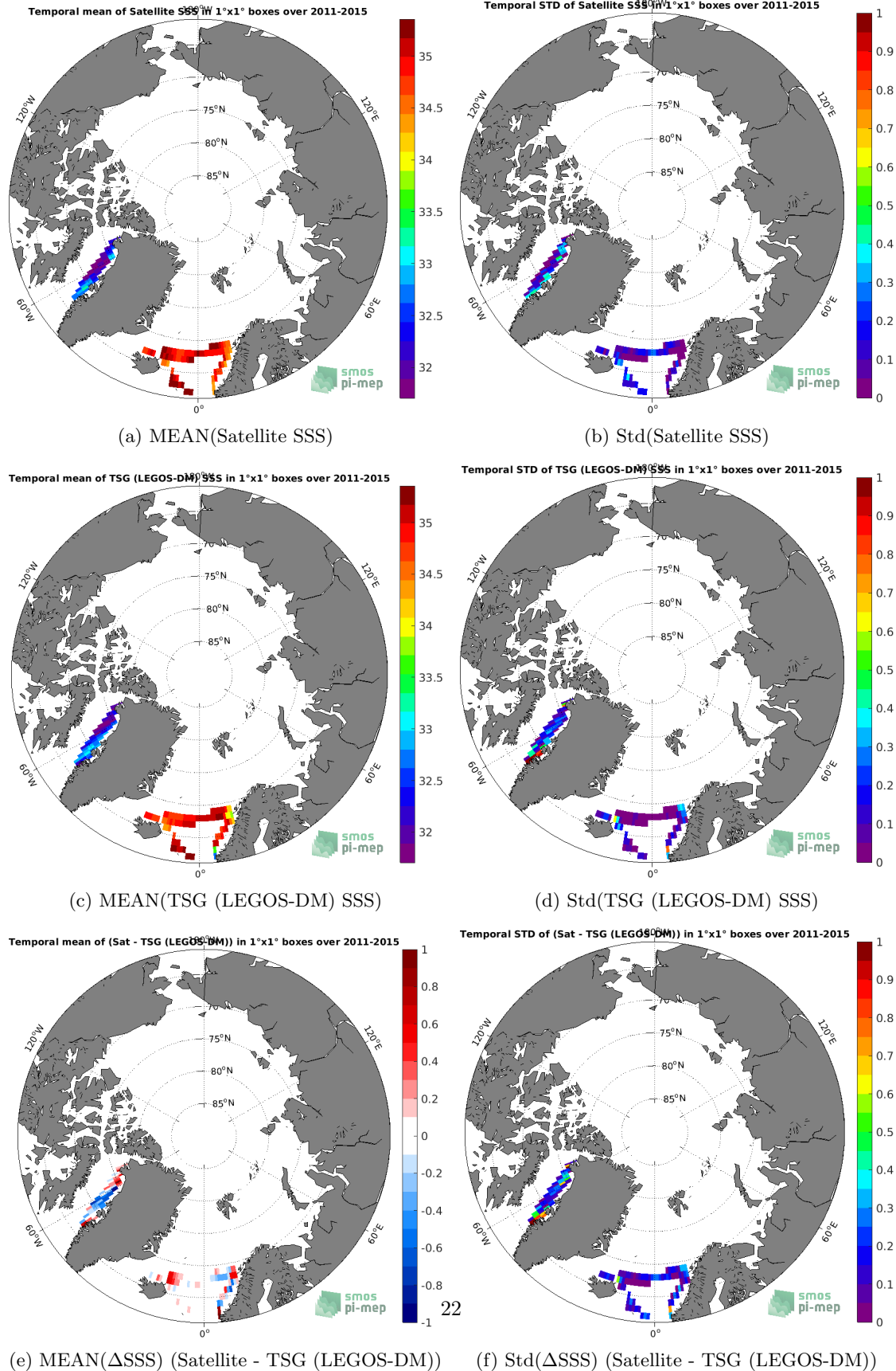
Figure 6: Temporal mean (left) and Std (right) of SSS from Aquarius SSS L4 OI v5 - Weekly (IPRC) (top), TSG (LEGOS-DM) (middle), and of \Delta SSS (Satellite - TSG (LEGOS-DM)). Only match-up pairs are used to generate these maps.
