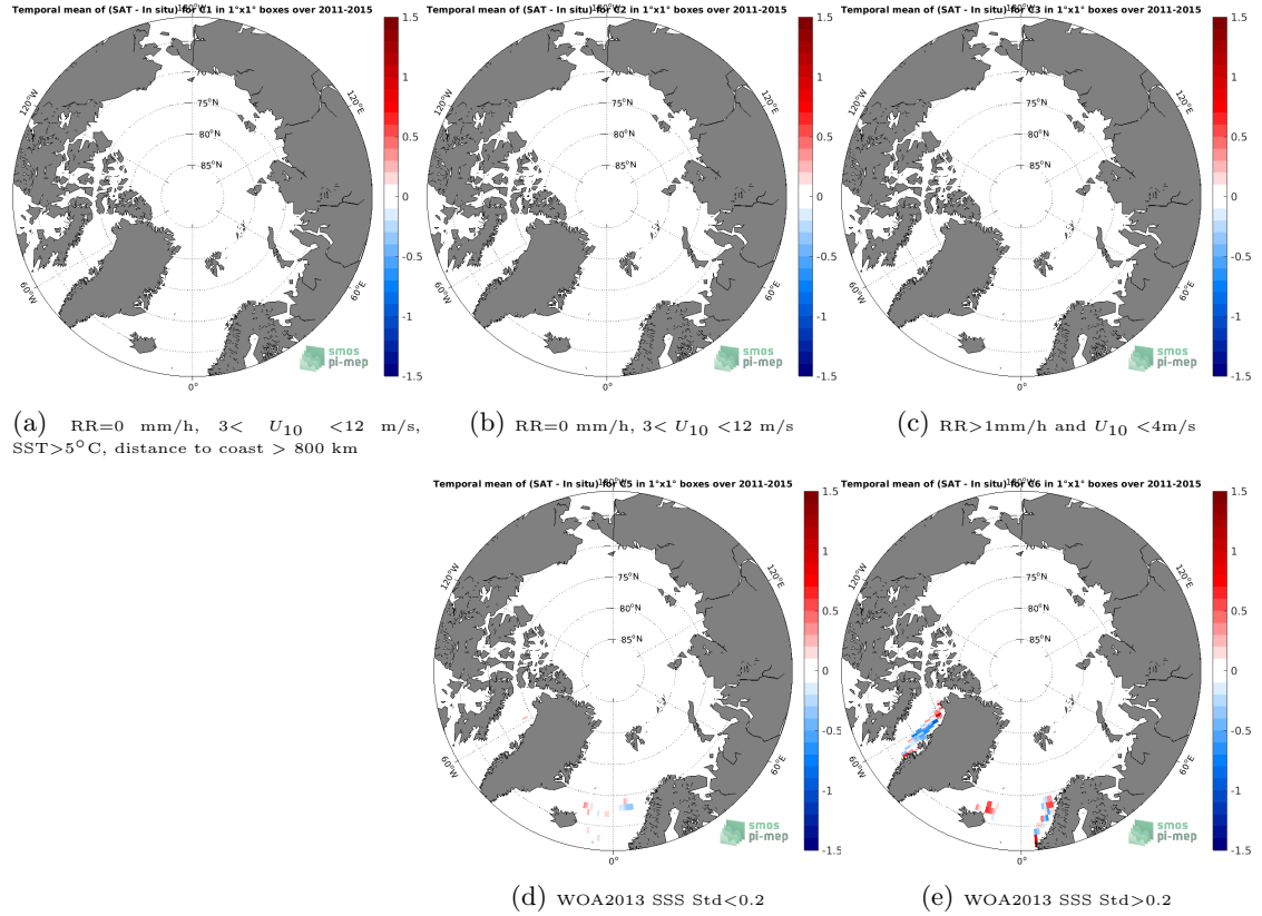
Figure 12: Temporal mean gridded over spatial boxes of size 1^{\circ}\times 1^{\circ} of \Delta\text{SSS} (Aquarius SSS L4 OI v5 - Weekly (IPRC) - TSG (LEGOS-DM)) for 5 different subdatasets corresponding to: RR=0 mm/h, 3 < U_{10} < 12 m/s, SST >5^{\circ}\text{C} , distance to coast > 800 km (a), RR=0 mm/h, 3 < U_{10} < 12 m/s (b), RR >1 mm/h and U_{10} < 4 m/s (c), WOA2013 SSS Std <0.2 (d), WOA2013 SSS Std >0.2 (e).
