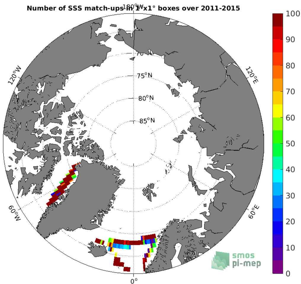
Figure 4: Number of SSS match-ups between TSG (LEGOS-DM) SSS and the Aquarius SSS L4 OI v5 - Weekly (IPRC) SSS product for the Arctic Ocean Pi-MEP region over 1°x1° boxes and for the full satellite product period.
