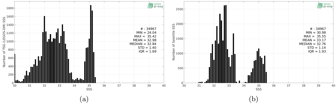
Figure 2: Histograms of SSS from TSG (LEGOS-DM) (a) and Aquarius SSS L4 OI v5 - Weekly (IPRC) (b) considering all match-up pairs per bins of 0.1 over the Arctic Ocean Pi-MEP region and for the full satellite product period.
