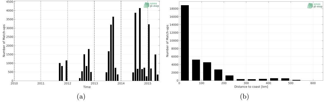
Figure 1: Number of match-ups between TSG (LEGOS-DM) and Aquarius SSS L4 OI v5 - Weekly (IPRC) SSS as a function of time (a) and as function of the distance to coast (b) over the Arctic Ocean Pi-MEP region and for the full satellite product period.
