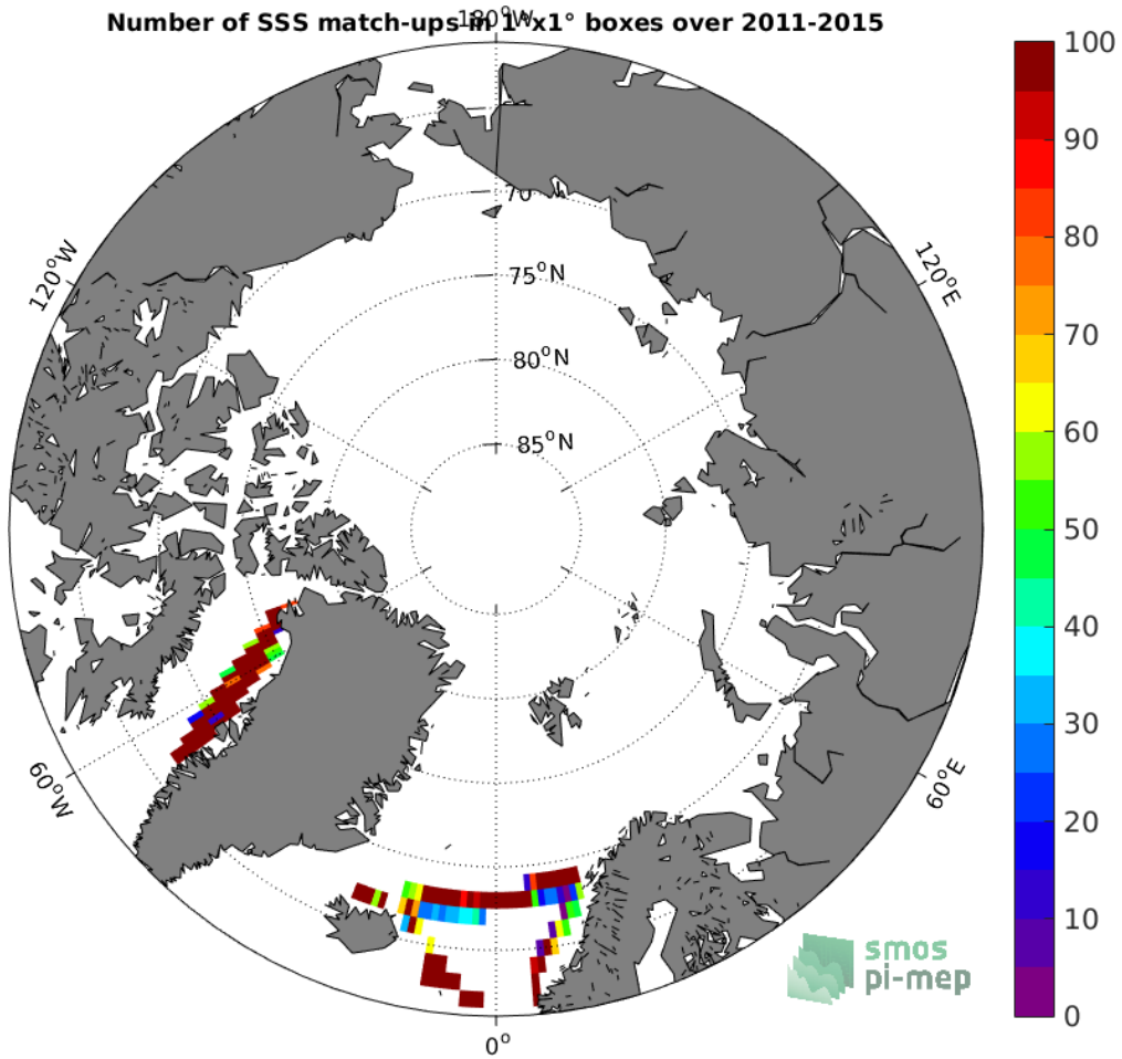
Figure 4: Number of SSS match-ups between TSG-LEGOS-DM SSS and the Aquarius-L4-IPRC-V5-WEEKLY SSS product for the Arctic Ocean Pi-MEP region over 1°x1° boxes and for the full satellite product period.
