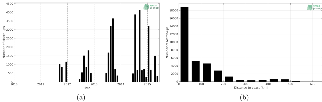
Figure 1: Number of match-ups between TSG-LEGOS-DM and Aquarius-L4-IPRC-V5-WEEKLY SSS as a function of time (a) and as function of the distance to coast (b) over the Arctic Ocean Pi-MEP region and for the full satellite product period.
