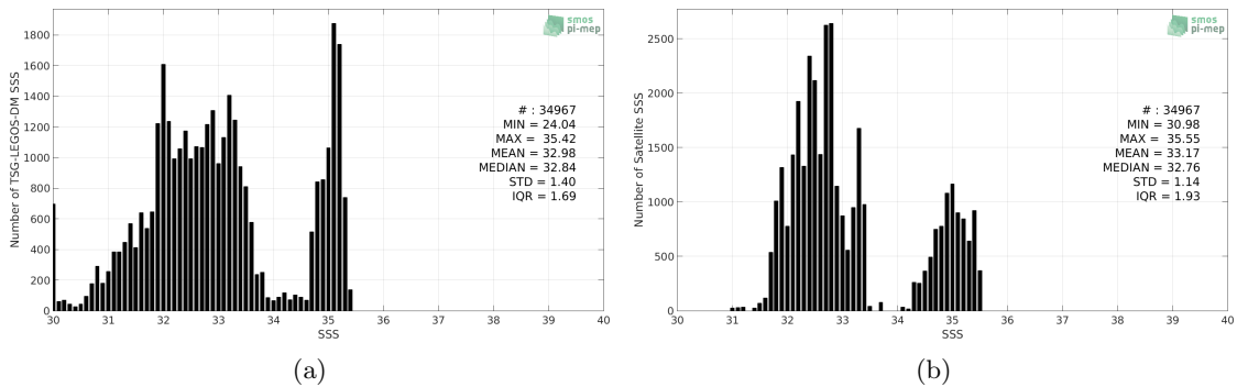
Figure 2: Histograms of SSS from TSG-LEGOS-DM (a) and Aquarius-L4-IPRC-V5-WEEKLY (b) considering all match-up pairs per bins of 0.1 over the Arctic Ocean Pi-MEP region and for the full satellite product period.
