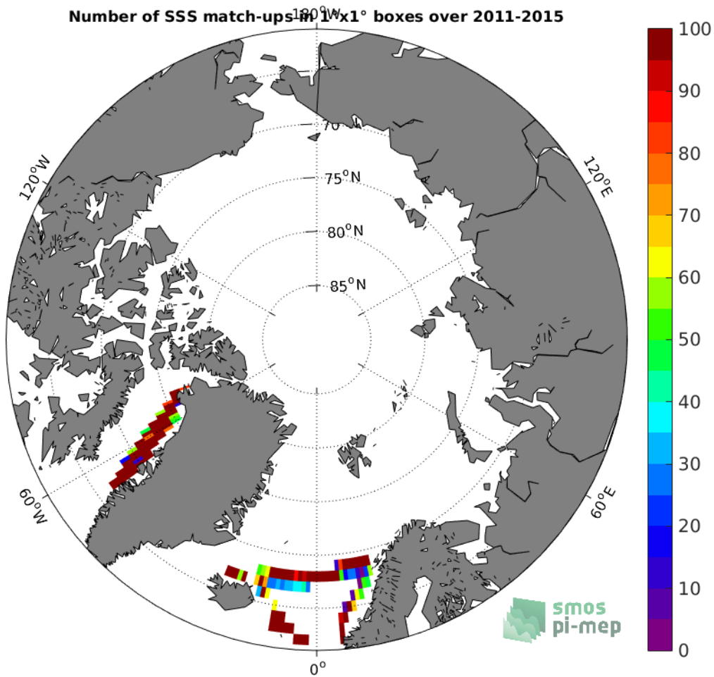
Figure 4: Number of SSS match-ups between TSG-LEGOS-DM SSS and the Aquarius-L4-IPRC-V5-WEEKLY SSS product for the Arctic Ocean Pi-MEP region over 1^\circ \times 1^\circ boxes and for the full satellite product period.
