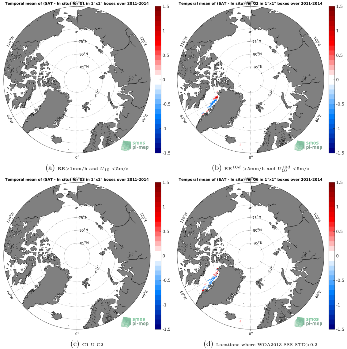
Figure 12: Temporal mean gridded over spatial boxes of size 1^\circ \times 1^\circ of \Delta SSS (Aquarius-L4-IPRC-V5-WEEKLY - TSG-LEGOS-DM) for 4 different subdatasets corresponding to: RR > 1\text{mm/h} and U_{10} < 5\text{m/s} (a), RR^{10d} > 5\text{mm/h} and U_{10}^{10d} < 5\text{m/s} (b), C1 U C2 (c), Locations where WOA2013 SSS STD > 0.2 (d).
