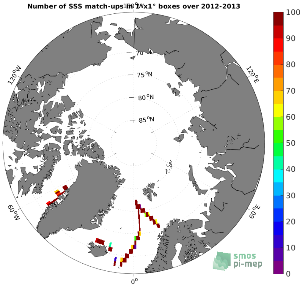
Figure 4: Number of SSS match-ups between TSG (GOSUD-Sailing-ship) SSS and the Aquarius SSS L4 OI v5 - Weekly (IPRC) SSS product for the Arctic Ocean Pi-MEP region over 1^{\circ} \times 1^{\circ} boxes and for the full satellite product period.
