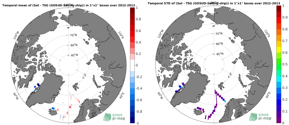
(e) MEAN( \Delta SSS) (Satellite - TSG (GOSUD-Sailing-ship))
