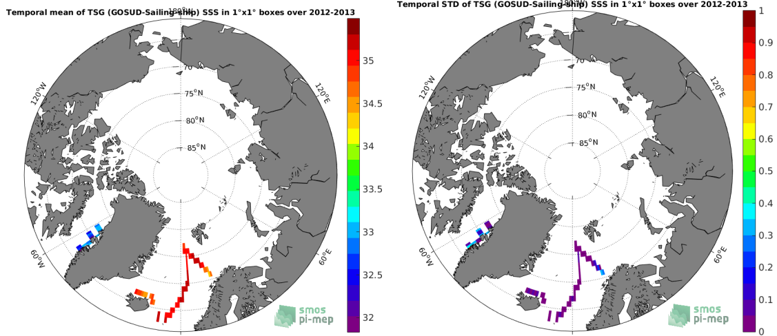
(c) MEAN(TSG (GOSUD-Sailing-ship) SSS)
