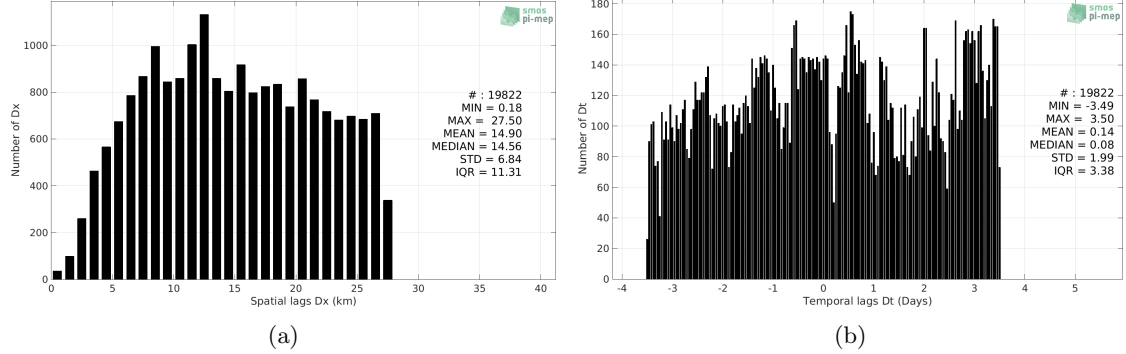
Figure 5: Histograms of the spatial (a) and temporal (b) lags between the time of the TSG (GOSUD-Sailing-ship) measurements and the date of the corresponding Aquarius SSS L4 OI v5 - Weekly (IPRC) SSS product.
