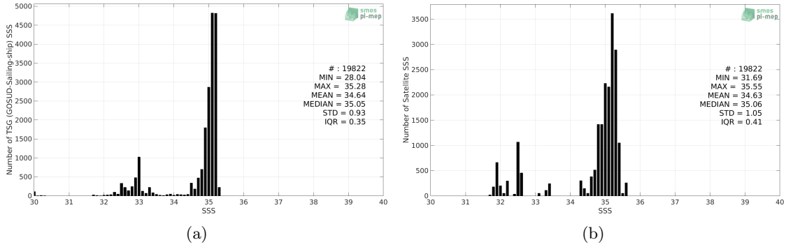
Figure 2: Histograms of SSS from TSG (GOSUD-Sailing-ship) (a) and Aquarius SSS L4 OI v5 - Weekly (IPRC) (b) considering all match-up pairs per bins of 0.1 over the Arctic Ocean Pi-MEP region and for the full satellite product period.
