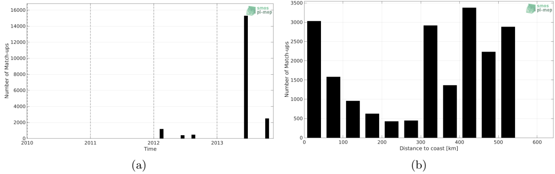
Figure 1: Number of match-ups between TSG (GOSUD-Sailing-ship) and Aquarius SSS L4 OI v5 - Weekly (IPRC) SSS as a function of time (a) and as function of the distance to coast (b) over the Arctic Ocean Pi-MEP region and for the full satellite product period.
