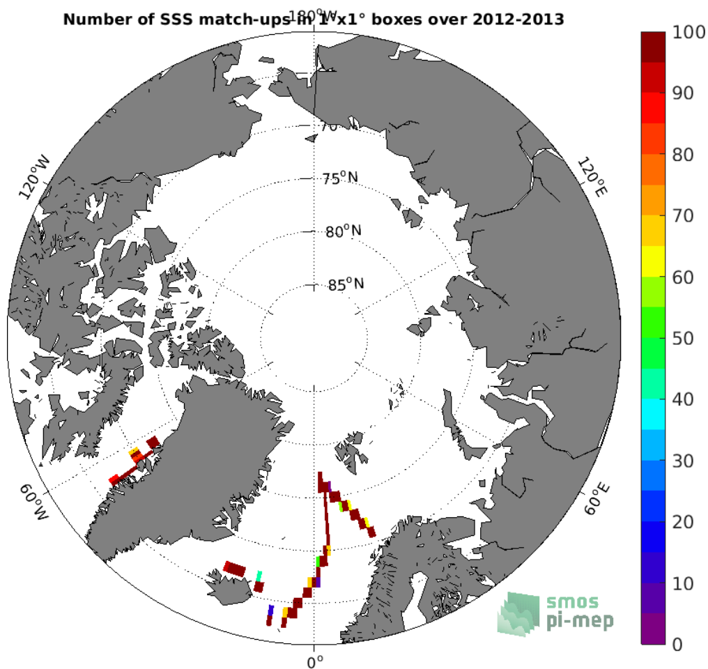
Figure 4: Number of SSS match-ups between TSG (GOSUD-Sailing-ship) SSS and the Aquarius SSS L4 OI v5 - Weekly (IPRC) SSS product for the Arctic Ocean Pi-MEP region over 1°x1° boxes and for the full satellite product period.
