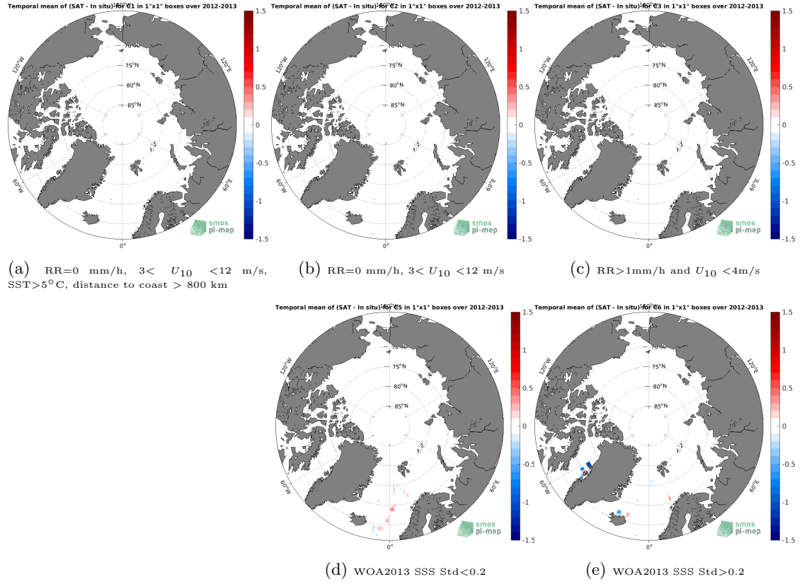
Figure 12: Temporal mean gridded over spatial boxes of size 1^\circ \times 1^\circ of \Delta\text{SSS} (Aquarius SSS L4 OI v5 - Weekly (IPRC) - TSG (GOSUD-Sailing-ship)) for 5 different subdatasets corresponding to: RR=0 mm/h, 3 < U_{10} < 12 m/s, SST > 5^\circ\text{C} , distance to coast > 800 km (a), RR=0 mm/h, 3 < U_{10} < 12 m/s (b), RR > 1 mm/h and U_{10} < 4 m/s (c), WOA2013 SSS Std < 0.2 (d), WOA2013 SSS Std > 0.2 (e).
