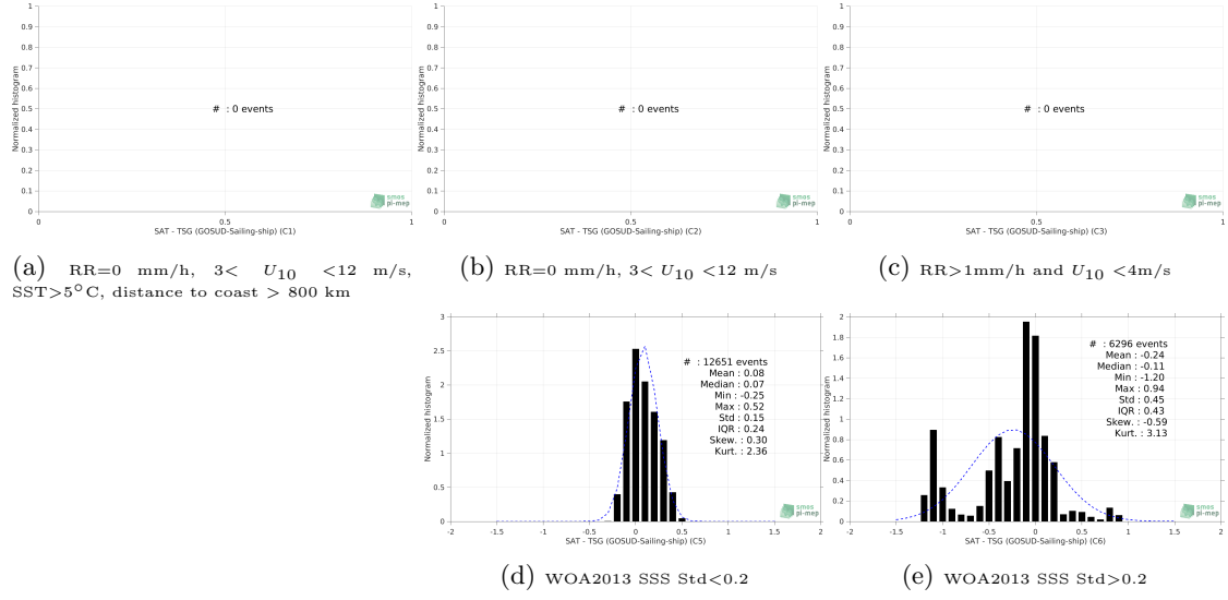
Figure 13: Normalized histogram of \Delta\text{SSS} (Aquarius SSS L4 OI v5 - Weekly (IPRC) - TSG (GOSUD-Sailing-ship)) for 5 different subdatasets corresponding to: RR=0 mm/h, 3 < U_{10} < 12 m/s, SST > 5^\circ\text{C} , distance to coast > 800 km (a), RR=0 mm/h, 3 < U_{10} < 12 m/s (b), RR > 1 mm/h and U_{10} < 4 m/s (c), WOA2013 SSS Std < 0.2 (d), WOA2013 SSS Std > 0.2 (e).
