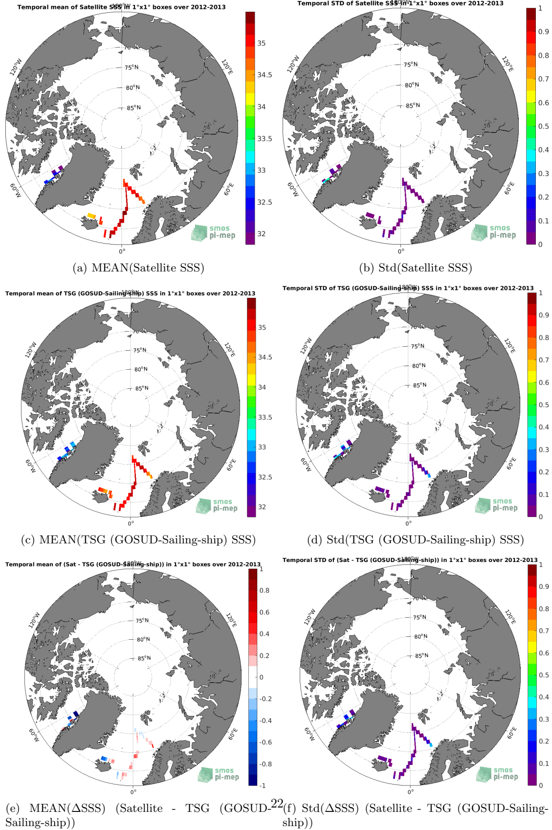
Figure 6: Temporal mean (left) and Std (right) of SSS from Aquarius SSS L4 OI v5 - Weekly (IPRC) (top), TSG (GOSUD-Sailing-ship) (middle), and of \Delta SSS (Satellite - TSG (GOSUD-Sailing-ship)). Only match-up pairs are used to generate these maps.
