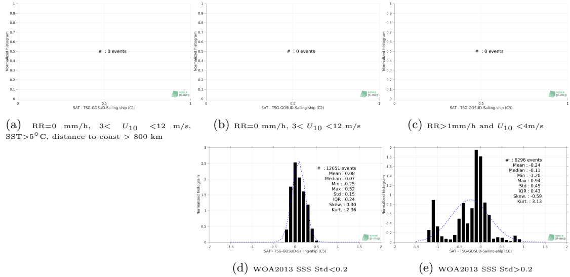
Figure 13: Normalized histogram of \Delta SSS (Aquarius-L4-IPRC-V5-WEEKLY - TSG-GOSUD-Sailing-ship) for 5 different subdatasets corresponding to: RR=0 mm/h, 3 < U_{10} < 12 m/s, SST > 5°C, distance to coast > 800 km (a), RR=0 mm/h, 3 < U_{10} < 12 m/s (b), RR > 1mm/h and U_{10} < 4 m/s (c), WOA2013 SSS Std < 0.2 (d), WOA2013 SSS Std > 0.2 (e).
