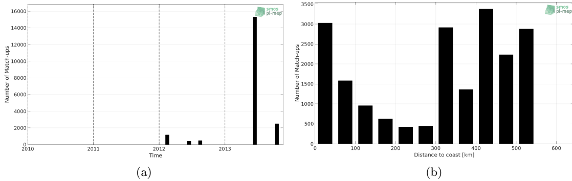
Figure 1: Number of match-ups between TSG-GOSUD-Sailing-ship and Aquarius-L4-IPRC-V5-WEEKLY SSS as a function of time (a) and as function of the distance to coast (b) over the Arctic Ocean Pi-MEP region and for the full satellite product period.
