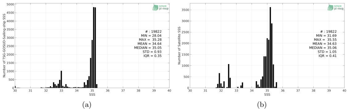
Figure 2: Histograms of SSS from TSG-GOSUD-Sailing-ship (a) and Aquarius-L4-IPRC-V5-WEEKLY (b) considering all match-up pairs per bins of 0.1 over the Arctic Ocean Pi-MEP region and for the full satellite product period.
