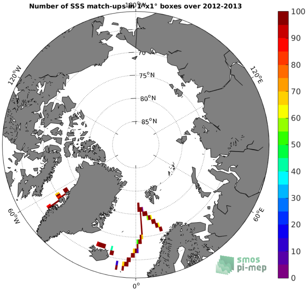
Figure 4: Number of SSS match-ups between TSG-GOSUD-Sailing-ship SSS and the Aquarius-L4-IPRC-V5-WEEKLY SSS product for the Arctic Ocean Pi-MEP region over 1°x1° boxes and for the full satellite product period.
