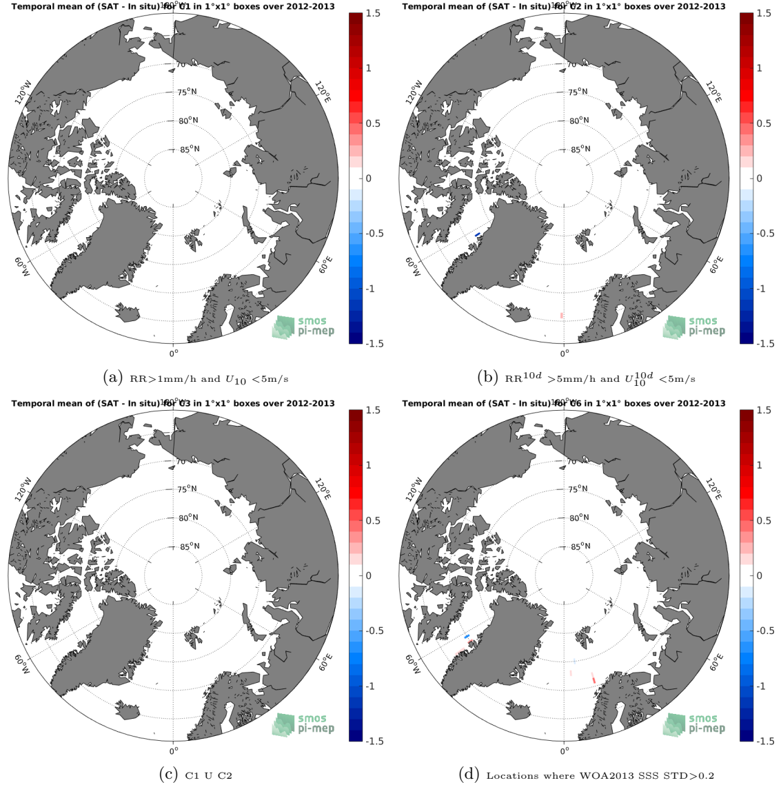
Figure 12: Temporal mean gridded over spatial boxes of size 1^\circ \times 1^\circ of \Delta SSS (Aquarius-L4-IPRC-V5-WEEKLY - TSG-GOSUD-Sailing-ship) for 4 different subdatasets corresponding to: RR > 1\text{mm/h} and U_{10} < 5\text{m/s} (a), RR^{10d} > 5\text{mm/h} and U_{10}^{10d} < 5\text{m/s} (b), C1 U C2 (c), Locations where WOA2013 SSS STD > 0.2 (d).
